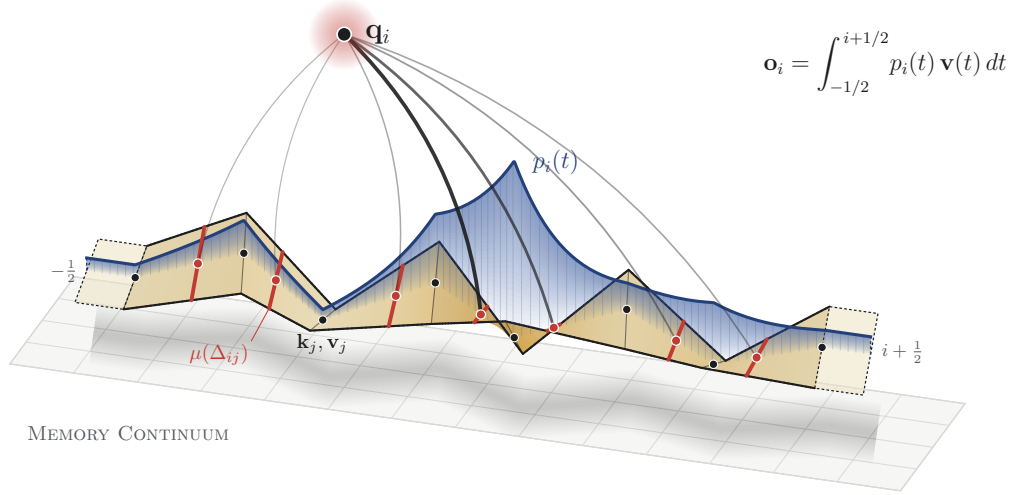
Figure 1: Overview of Continuum Attention. Adjacent key and value representations define a continuous memory trajectory. Each query induces a relevance density p_i(t) and determines adaptive retrieval positions \mu(\Delta_{ij}) within memory segments. Exact integration, including the half token boundary extensions, produces the attention output.
