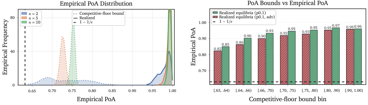
Figure 2 | Left: Empirical distributions of the Theorem 3 bound (dotted) and the empirical PoA (solid) across 100k random n -model subsets of EmbedLLM, for n \in \{2, 5, 10\} . Both distributions tighten as n grows, and are well above the distribution-free baseline (dashed). Right: Bottom 0.1% of empirical PoA across sub-markets grouped by bound bin (100k samples per bin), for both typical equilibria (solid green) and approximate, adversarial equilibria (hatched red).
