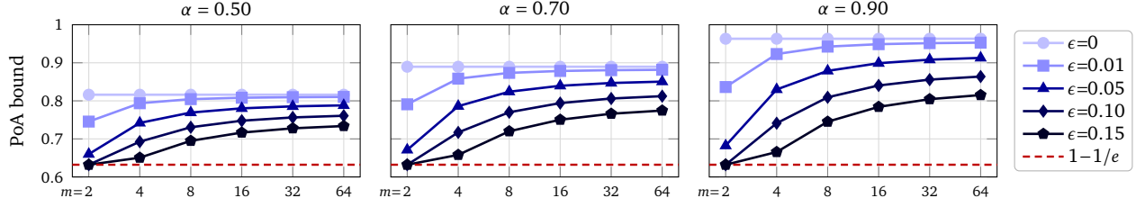
Figure 1 | Price-of-anarchy bounds under competitive floors, for various settings of (\alpha, m, \epsilon) . Each entry represents the bound for any distribution with \mathbb{P}(V_{(m)} < \alpha \mathbb{E}[V_{(1)}]) \leq \epsilon . At \epsilon = 0 , we recover the deterministic floor bound from Equation (4); higher \epsilon start to degrade the efficiency. Larger numbers of credible competitors ( m \geq 4 ) stabilize the market, and preserve efficiency even under high \epsilon .
