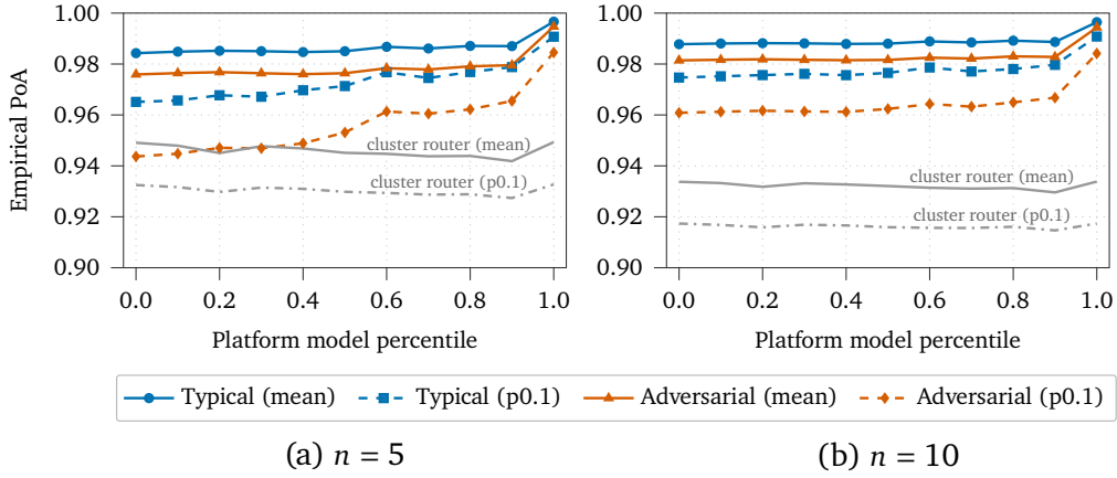
Figure 4 | Empirical PoA with a platform-owned bidder, as a function of where the platform model sits in the ranking of EmbedLLM models by average value. Each point averages 10,000 markets made of the strongest model, n random rivals, and the platform model. Solid lines are means and dashed lines are the 0.1 percentile across markets, for typical (blue) and adversarial (orange) equilibria. Gray lines mark the cluster router on the same markets (mean solid, 0.1 percentile dash-dotted).
