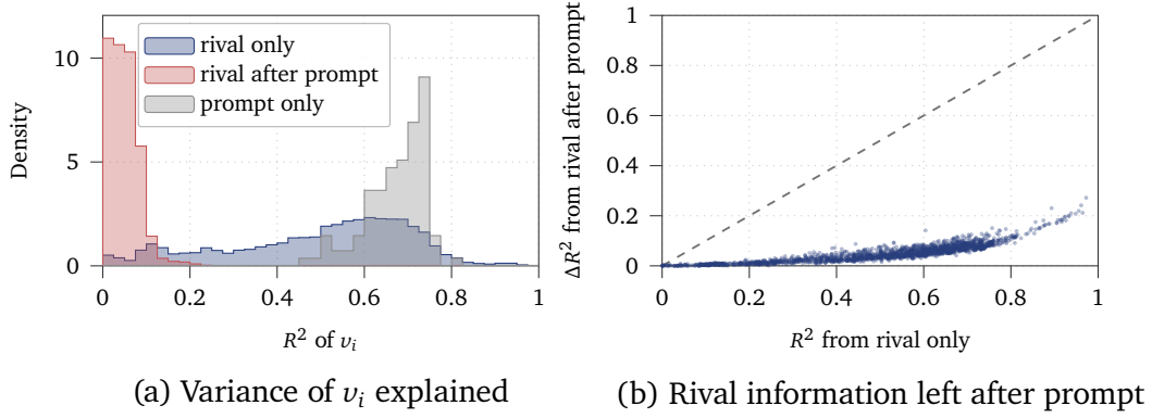
Figure 3 | How well the prompt and a rival predict each model’s value v_i . (a) Distribution of R^2 from the held-out ridge prediction g_i(q) alone (one value per model), and from a rival’s value v_j alone and the gain from adding the rival once the prompt is known (one value per ordered model pair (i, j) ). (b) Each point is one of 2,000 randomly sampled model pairs (i, j) , plotting the rival’s R^2 on its own against the gain it adds once the prompt is known. The dashed line is y = x . For points far below it, most of what the rival’s value predicts about v_i is already captured by the prompt.
