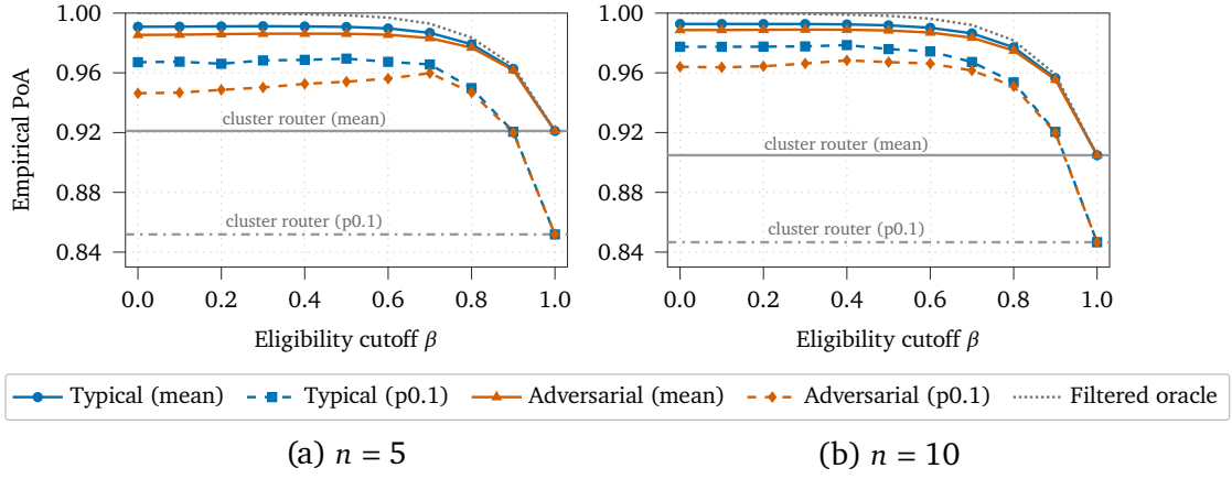
Figure 5 | Empirical PoA under pre-auction filtering, as a function of the eligibility cutoff \beta . Each point averages 10,000 random markets of n models. Solid lines are means and dashed lines are the 0.1 percentile across markets, for typical (blue) and adversarial (orange) equilibria. The dotted line is the filtered oracle, the welfare of always allocating to the best admitted model. Gray lines mark the cluster router, which sends every prompt to its cluster’s best model (mean solid, 0.1 percentile dash-dotted).
