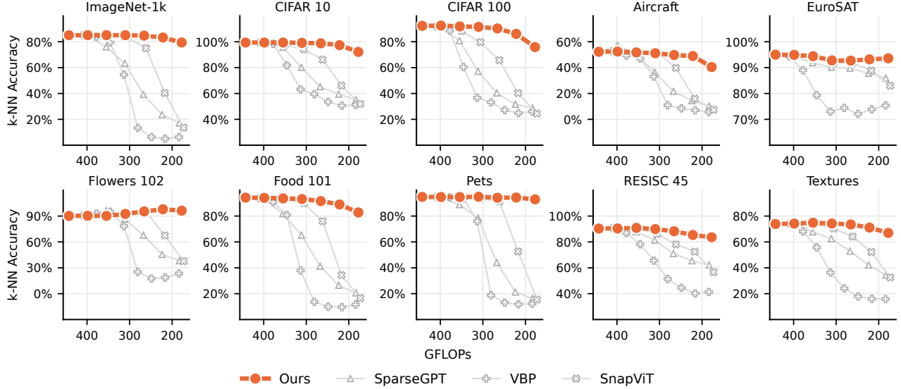
Figure 15 DINOv3 ViT-H+/16 is nearly lossless at 50% sparsity, and improves on Flowers 102. Top-1 k-NN accuracy versus GFLOPs curves on ImageNet-1k and the nine transfer datasets for DINOv3 ViT-H+/16 pruned from 10% to 60% sparsity with our method and the baselines. At 50% sparsity, our method loses 1.8% on ImageNet-1k, and between 0.5% on Pets and 6.2% on CIFAR-100 on the transfer datasets, while Flowers 102 improves from 90.2% to 97.9%. At the same sparsity, it leads SnapViT, the runner-up, by 42.9% on ImageNet-1k, and from 40% onward it matches or exceeds every baseline on every dataset.
