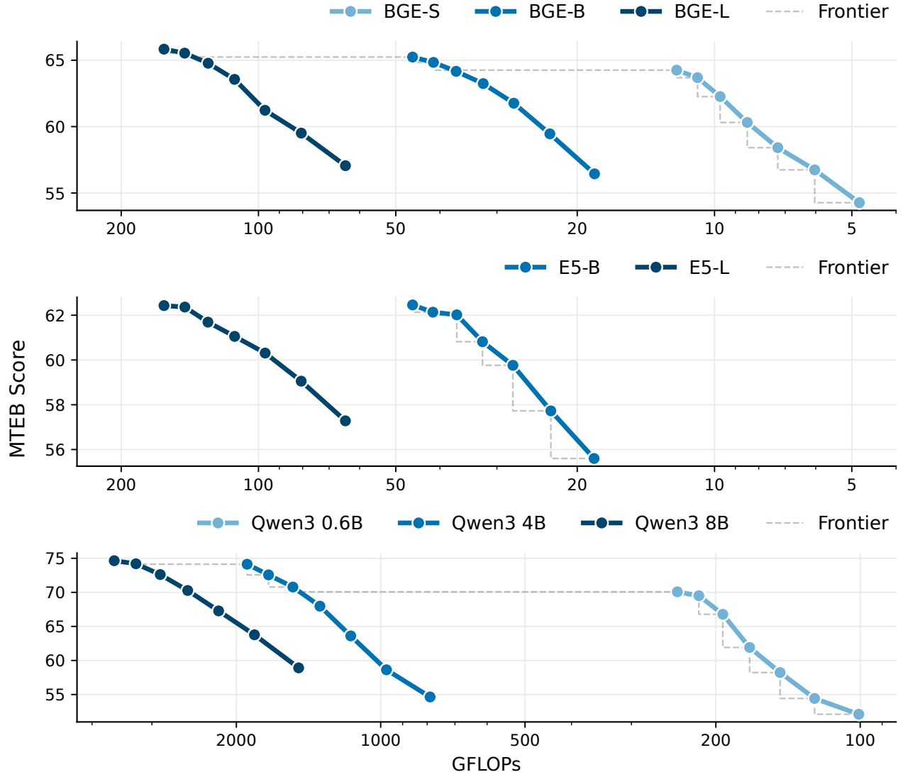
Figure 19 Elastic pruning extends the performance-compute frontier of dense text encoders. MTEB score versus GFLOPs for BGE, E5, and Qwen3 encoders, from dense to 60% sparsity. Dashed lines indicate the pareto frontier. GFLOPs are shown on a logarithmic scale.
