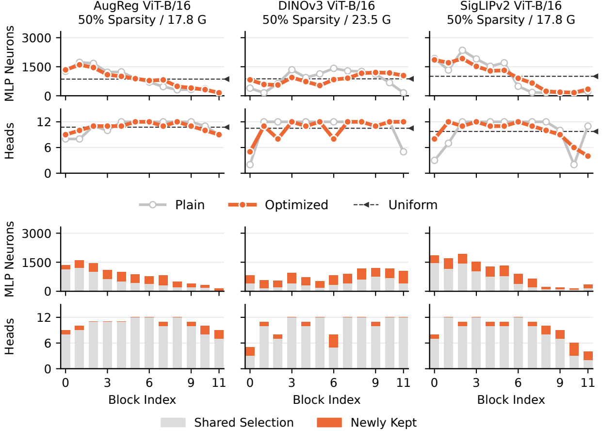
Figure 5 Ranking optimization changes both cross-block sparsity allocation and within-block selection. Retained MLP neurons and attention heads at 50% sparsity for AugReg, DINOv3, and SigLIPv2 ViT-B/16. The top rows compare per-block allocations from plain and optimized scores with uniform pruning. The bottom rows use the optimized per-block allocation and divide its retained units into those also selected by the plain scores and those newly selected after ranking optimization. Newly retained units appear even where block-level allocations remain nearly unchanged, showing that ranking optimization also reorders units within blocks rather than merely redistributing capacity across them.
