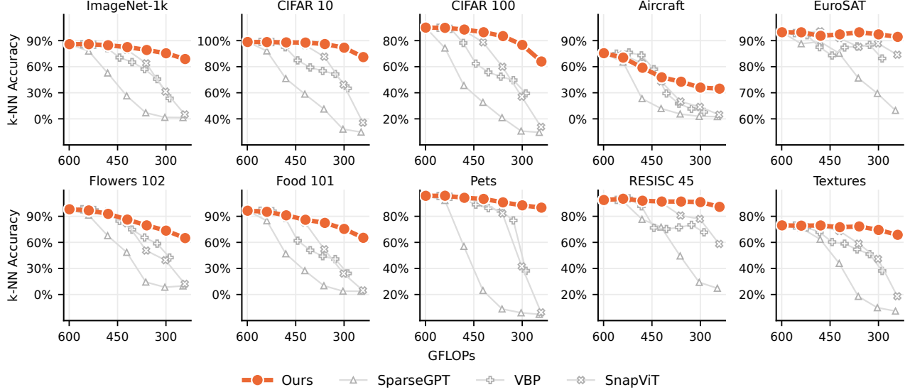
Figure 16 SigLIPv2 ViT-G/16 degrades unevenly at 50% sparsity, with fine-grained tasks being the most sensitive. Top-1 k-NN accuracy versus GFLOPs curves on ImageNet-1k and the nine transfer datasets for SigLIPv2 ViT-G/16 pruned from 10% to 60% sparsity with our method and the baselines. At 50% sparsity, our method loses 10.5% on ImageNet-1k, and between 0.8% on EuroSAT and 39.6% on Aircraft on the transfer datasets. Under shallow pruning, VBP and SnapViT lead on Aircraft, by 12.9% and 5.4% at 20% sparsity, but from 30% onward our method leads every baseline on every dataset.
