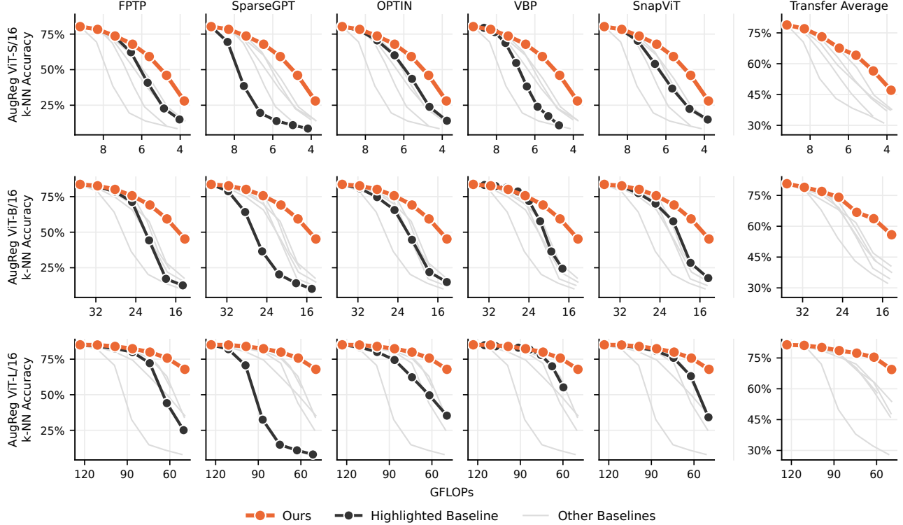
Figure 9 Larger AugReg models tolerate more pruning. Top-1 k-NN accuracy on ImageNet-1k and transfer datasets for AugReg models pruned with our method and the baselines.
