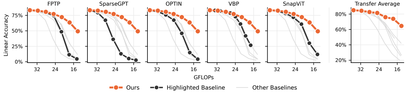
Figure 7 Our method degrades more smoothly under linear probing on AugReg ViT-B/16. Top-1 accuracy in linear classification on ImageNet-1k and transfer datasets for AugReg ViT-B/16 models pruned with our method and the baselines. Compared with the corresponding k-NN results in Figure 9, linear probes retain more accuracy under deep pruning.
