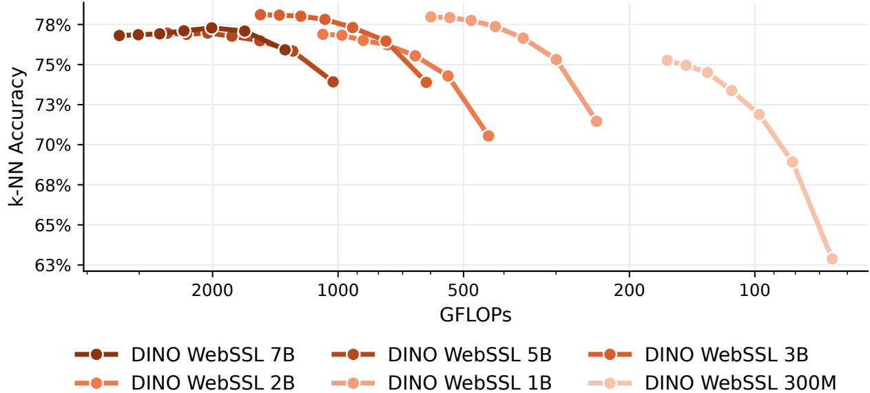
Figure 13 Pruned larger models can outperform smaller dense models. ImageNet-1k top-1 k-NN accuracy versus GFLOPs for the six-model DINO WebSSL family, pruned with our method from dense to 60% sparsity. Pruned 3B and 7B models pareto-dominate the dense 2B and 5B anchors.
