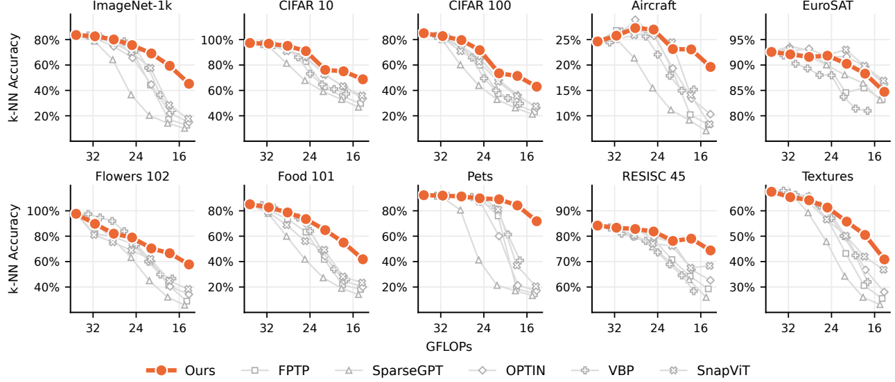
Figure 14 AugReg ViT-B/16 degrades unevenly across tasks, with fine-grained tasks being the most sensitive. Top-1 k-NN accuracy versus GFLOPs curves on ImageNet-1k and the nine transfer datasets for AugReg ViT-B/16 pruned from 10% to 60% sparsity with our method and the baselines. At 50% sparsity, our method loses 24.3% on ImageNet-1k and over 30% on CIFAR-100, Flowers 102, and Food 101, but at most 8.1% on Pets, EuroSAT, and RESISC45. Our method leads the baselines under moderate and deep pruning, except on EuroSAT, where SnapViT and OPTIN retain higher accuracy.
