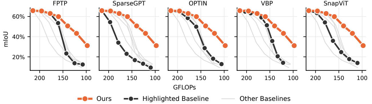
Figure 17 Our method preserves patch-level representations. In-context semantic segmentation mIoU on Pascal VOC 2012 for AugReg ViT-B/16 models pruned with our method and the baselines. Our method retains performance under pruning, improving on the runner-up, OPTIN, by up to 25.1% at 50% sparsity.
