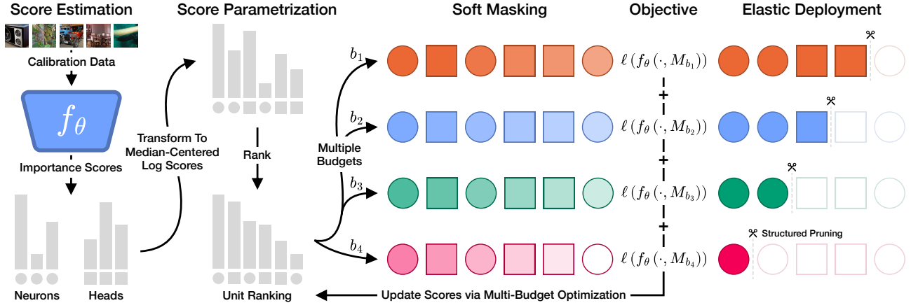
Figure 1 Differentiable soft pruning. Initial importance scores for MLP neurons and attention heads are transformed into learnable log-scores and median-centered by type, aligning their reference points without changing within-type rankings. At each optimization step, the joint ranking determines a threshold \kappa_b and soft mask M_b for each sparsity target b \in \mathcal{B} . We run the same calibration batch through the frozen model under each mask, average losses across targets, and update only the log-scores. Mask gradients concentrate near each threshold, so multiple targets expose different regions of the ranking to useful gradients. The optimized ranking can then be hard-pruned to any inference budget without further optimization.
