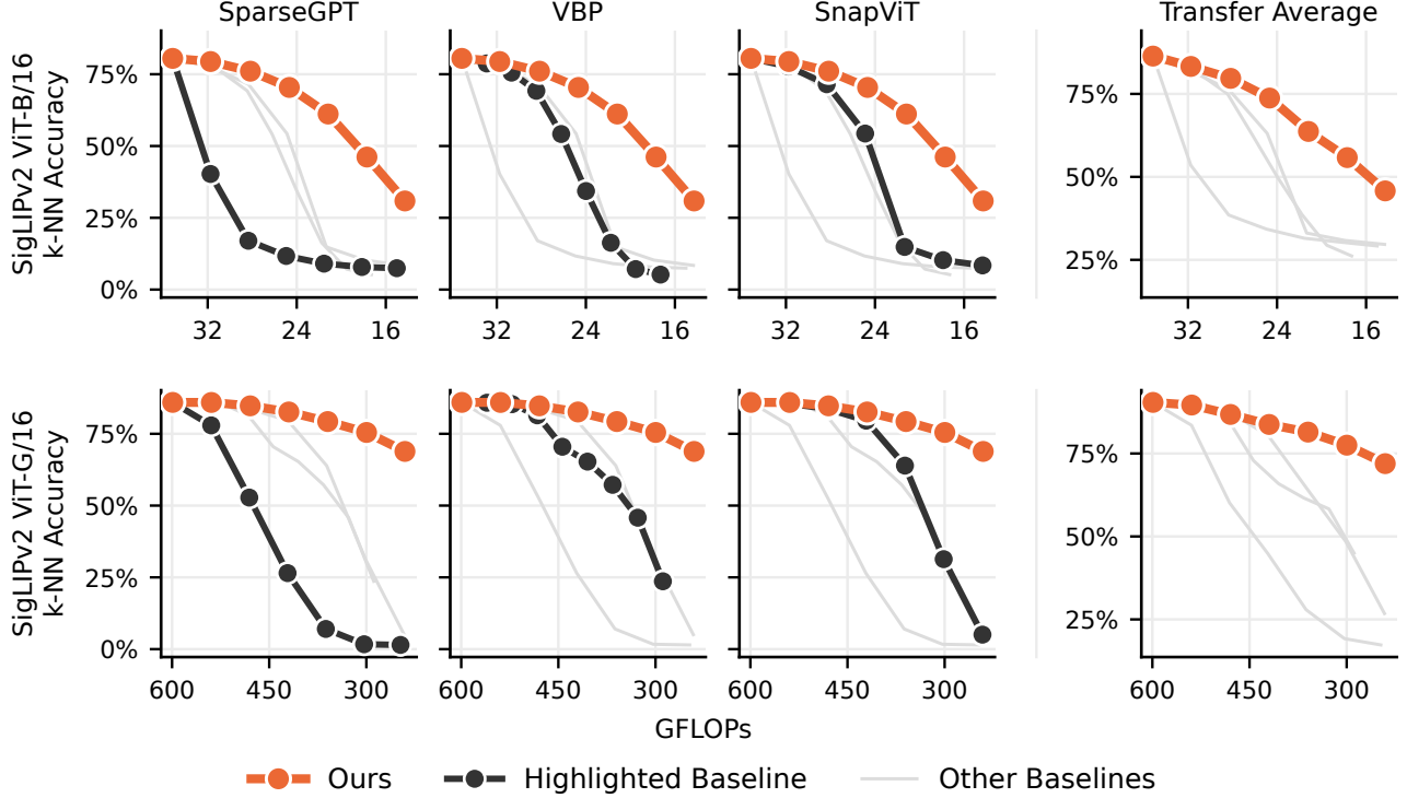
Figure 12 Larger SigLIPv2 models tolerate more pruning. Top-1 k-NN accuracy on ImageNet-1k and the transfer average for SigLIPv2 ViT-B/16 and ViT-G/16 models pruned with our method and the baselines. Our method yields smoother degradation on both models. Pruning the ViT-G/16 to 50% sparsity removes 573M parameters, while reducing k-NN accuracy by 10.5 percentage points on ImageNet-1k and 12.9 percentage points on the transfer average.
