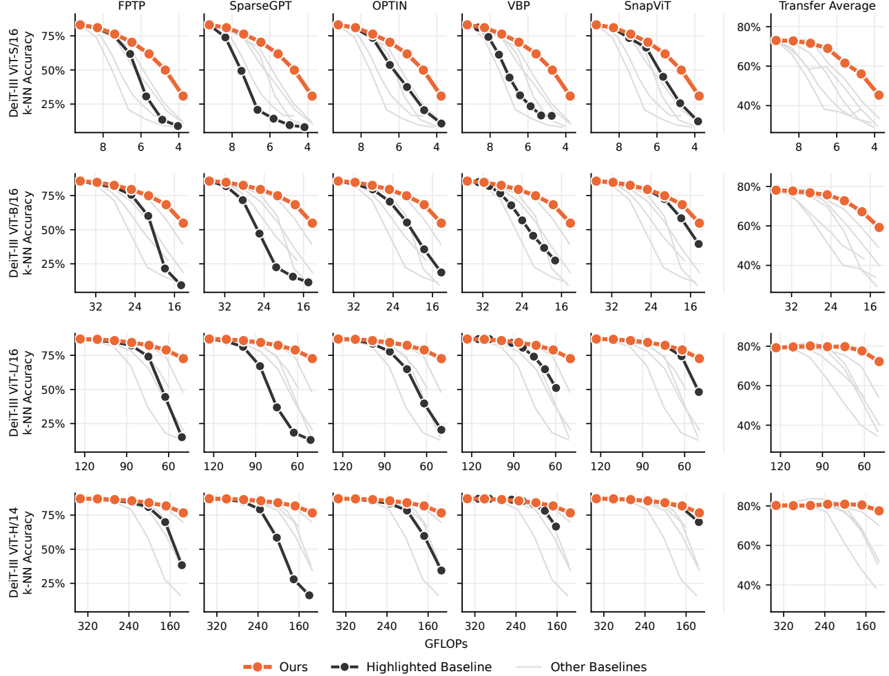
Figure 10 Larger DeiT-III models tolerate more pruning. Top-1 k-NN accuracy on ImageNet-1k and transfer datasets for DeiT-III models pruned with our method and the baselines. At 60% sparsity, ViT-H/14 loses 10.4% on ImageNet-1k and 2.73% on the transfer average, while removing approximately 378M parameters.
