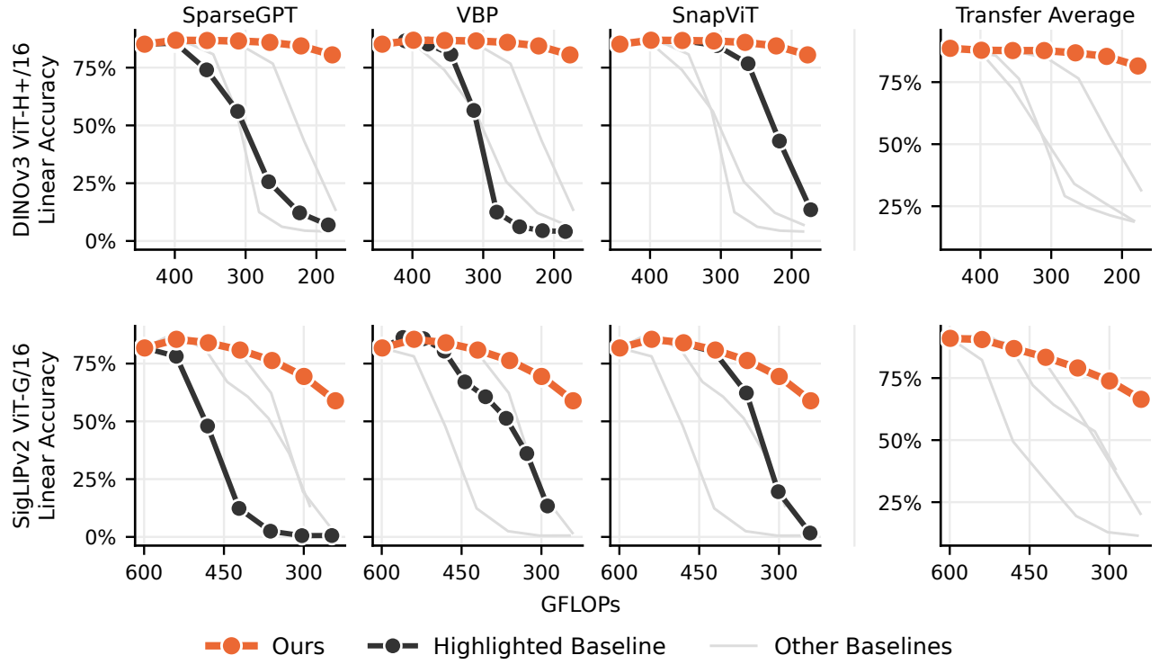
Figure 8 Our method outperforms baselines in linear classification under deep pruning on large DINOv3 and SigLIPv2 models. Top-1 accuracy in linear classification on ImageNet-1k and transfer datasets for DINOv3 ViT-H+/16 (top) and SigLIPv2 ViT-G/16 (bottom), comparing our method with compatible baselines. Notably, the linear accuracy on ImageNet-1k for DINOv3 is essentially flat at up to 50% sparsity.
