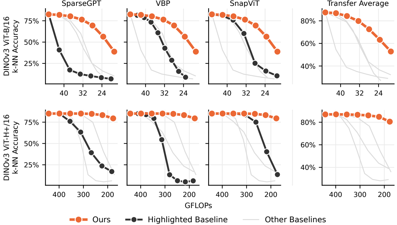
Figure 11 Larger DINOv3 models tolerate more pruning. Top-1 k-NN accuracy on ImageNet-1k and the transfer average for DINOv3 models pruned with our method and the baselines. Our method yields smoother degradation on both models. Pruning the ViT-H+/16 to 60% sparsity removes 512M parameters, while reducing k-NN accuracy by 5.6% on ImageNet-1k and 6.4% on the transfer average.
