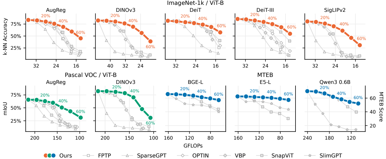
Figure 2 Our method yields smooth degradation curves across vision and text tasks. Performance versus compute for our method and six baselines from dense to 60% sparsity. Curve labels indicate FLOP sparsity. Top: ImageNet-1k top-1 k-NN accuracy. Bottom left: Pascal VOC 2012 Hummingbird mIoU. Bottom right: mean MTEB score. Baselines remain competitive under shallow pruning, but our method retains higher performance as sparsity increases, with the largest gains under moderate and deep pruning.
