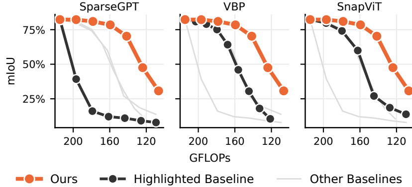
Figure 18 Our method preserves DINOv3’s patch-level representations under pruning. In-context semantic segmentation mIoU on Pascal VOC 2012 for DINOv3 ViT-B/16 models pruned with our method and the baselines. Our method degrades smoothly and consistently outperforms each baseline at comparable compute.
