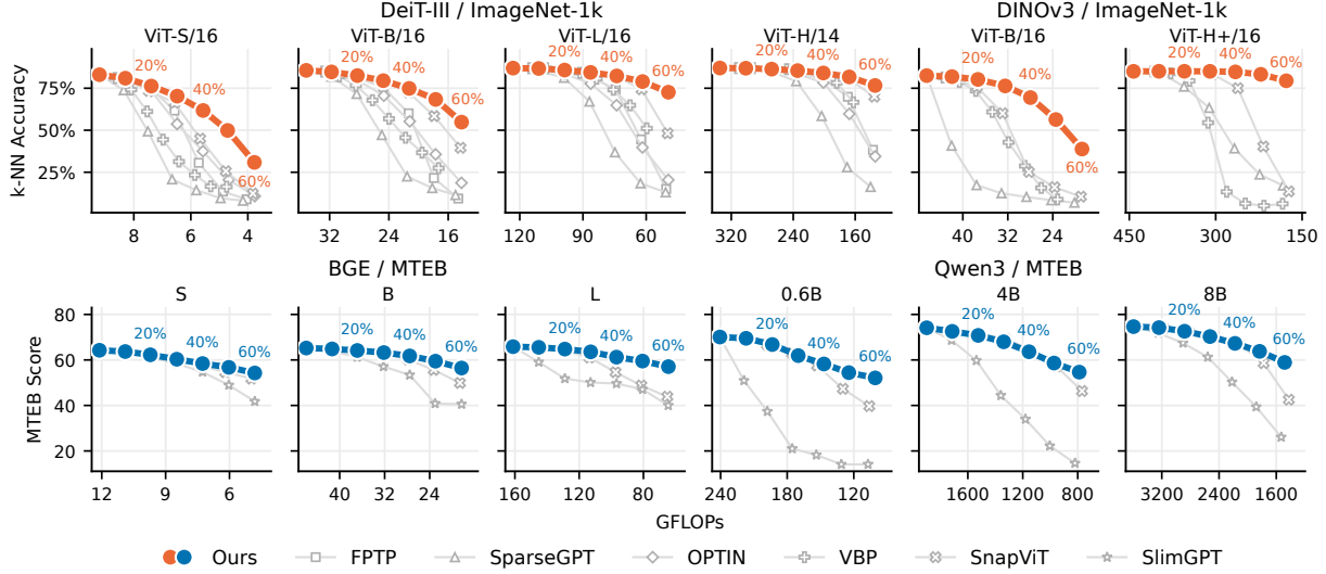
Figure 3 Larger vision models tolerate more pruning. Performance versus compute for our method and baselines from dense to 60% sparsity. Curve labels indicate FLOP sparsity. Top: ImageNet-1k top-1 k-NN accuracy for DeiT-III and DINOv3. Bottom: mean MTEB score for BGE and Qwen3. Size helps BGE modestly and Qwen3 inconsistently. Our advantage grows with size except on DeiT-III, where SnapViT remains competitive.
