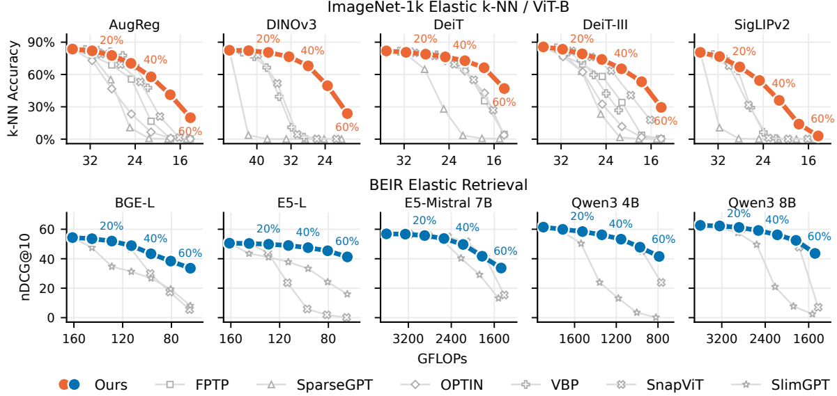
Figure 4 Our method better preserves compatibility with a fixed dense index. Performance versus compute for our method and baselines from dense to 60% sparsity, with the index encoded once by the dense model and queries encoded by its pruned counterparts. Curve labels indicate FLOP sparsity. Top: ImageNet-1k top-1 k-NN accuracy. Bottom: mean BEIR nDCG@10. Baselines remain competitive under shallow pruning, but our method supports deeper query encoder pruning without rebuilding the index.
