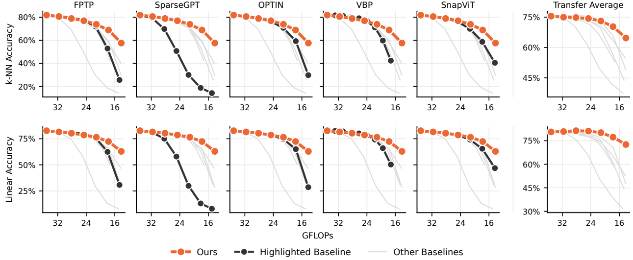
Figure 6 Our method retains higher accuracy under deep pruning on DeiT-B/16. Top-1 k-NN (top) and linear-probing (bottom) accuracy versus GFLOPs on ImageNet-1k and the transfer average. Most baselines are competitive under shallow pruning, but degrade more sharply than our method as sparsity increases.
