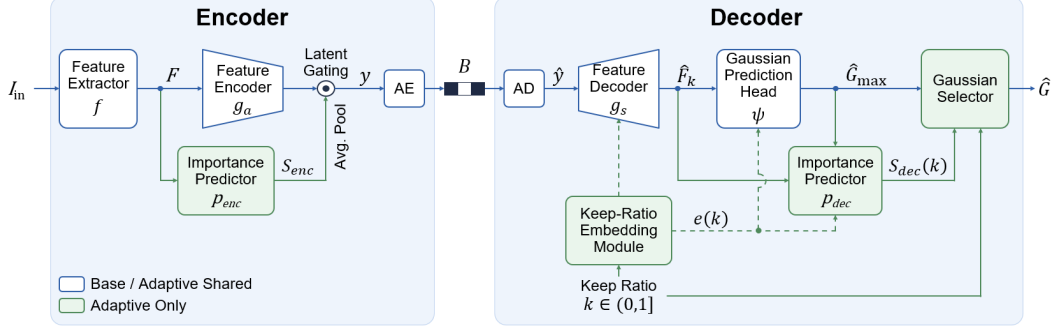
Figure 3: Overview of the MFGS framework from multi-view feature extraction through Gaussian reconstruction. The sender extracts F from sparse input views and encodes it into a bitstream, while the receiver decodes \hat{F} and predicts Gaussian primitives. The MFGS-Adaptive model additionally supports importance-guided bit allocation and receiver-side Gaussian selection. Green modules are specific to the MFGS-Adaptive model. AE and AD denote arithmetic encoding and decoding, respectively.
