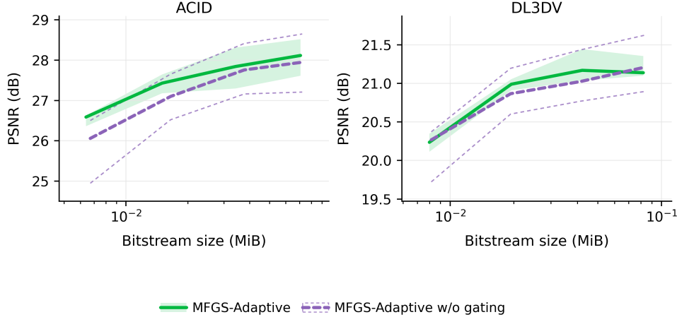
Figure 10: Encoder-side latent-gating ablation on ACID and DL3DV. The no-gating variant omits gating and the importance-alignment loss. Green shading and thin purple boundary curves indicate the ranges for the full and no-gating models, respectively. These ranges span k \in \{0.2, 0.4, 0.6, 0.8, 1.0\} ; lines connect rate settings at k = 0.4 .
