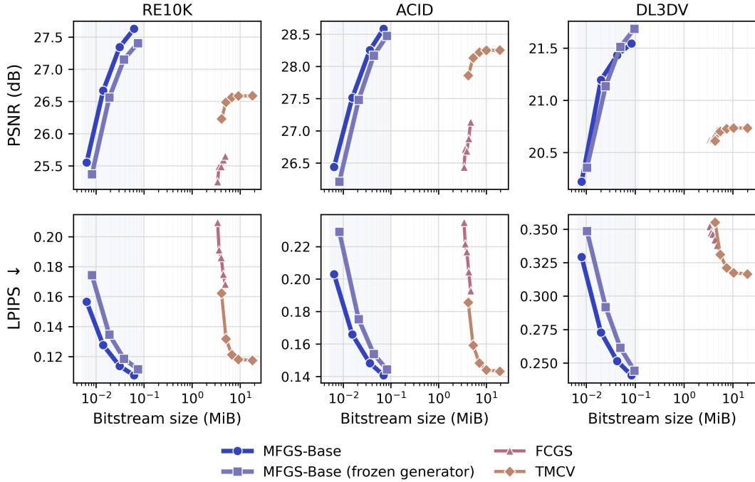
Figure 4: Rate–distortion curves for the MFGS-Base model, its frozen-generator variant, FCGS, and TMCV on RE10K, ACID, and DL3DV. The horizontal axis shows scene bitstream size on a logarithmic scale.
