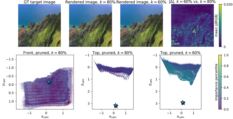
Figure 9: Scene-level Gaussian selection on ACID. The top row shows the ground-truth target image, reconstructions at k=0.8 and k=0.6 from the same bitstream, and their mean absolute RGB difference. The bottom row shows camera-aligned orthographic projections of excluded Gaussians, colored by decoder-side importance percentile within the full candidate set at each budget. Blue stars mark the reference input-camera center.
