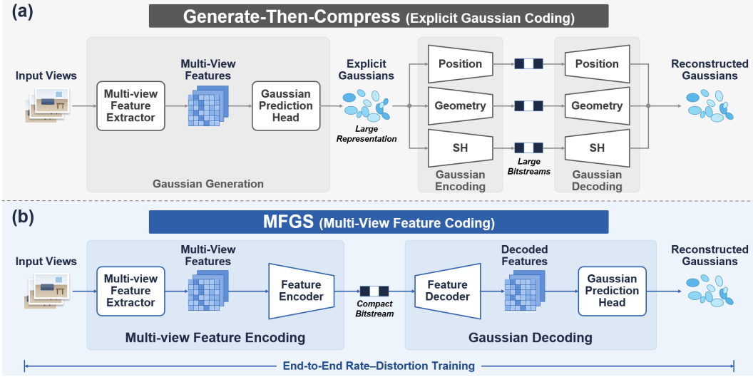
Figure 1: Comparison of 3D scene coding pipelines. (a) Generate-then-compress predicts explicit Gaussians and encodes their attributes through specialized paths, limiting joint compression of geometry and appearance. Non-differentiable operations such as G-PCC also hinder end-to-end training. (b) The MFGS framework compresses multi-view features with an established learned image codec and predicts Gaussian attributes from the decoded features at the receiver. This unified path simplifies coding, exploits cross-attribute redundancy, and enables end-to-end rate-distortion training, while compact latent grids reduce computation.
