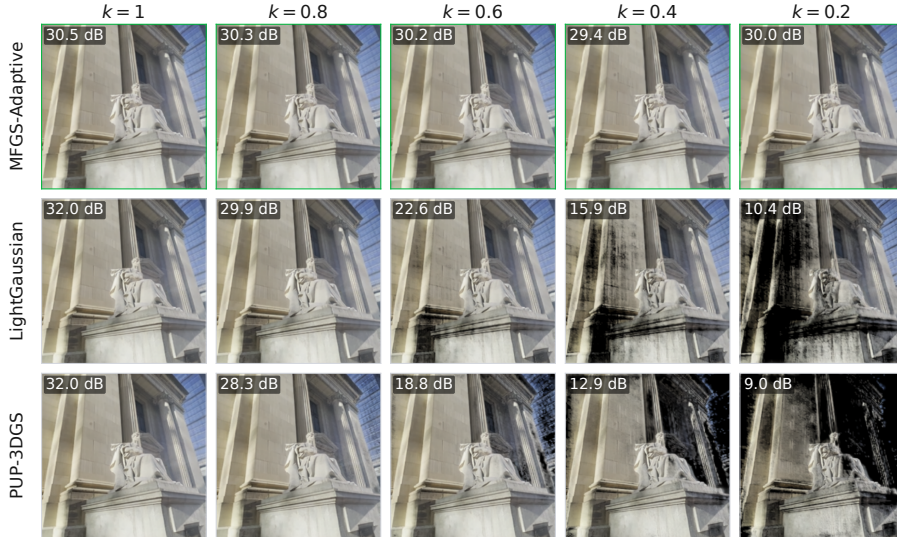
Figure 8: Qualitative pruning comparison on DL3DV across Gaussian keep ratios. Rows show the MFGS-Adaptive model and post-hoc pruning baselines at \lambda = 0.0256 , and columns show k decreasing from 1.0 to 0.2. Each panel reports PSNR with respect to the ground-truth target image.
