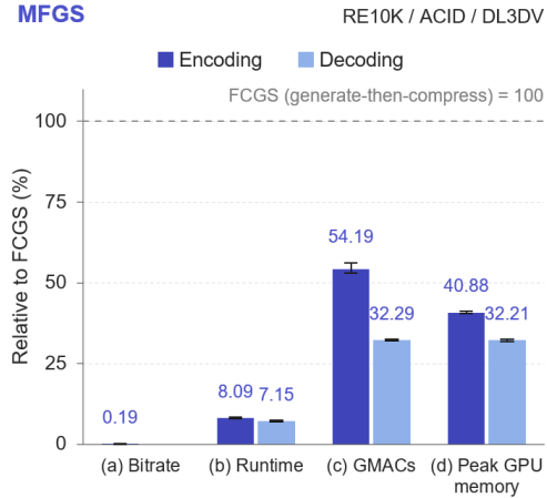
Figure 2: Relative bitrate and complexity of MFGS-Base versus FCGS (generate-then-compress), using the same generator architecture (Section 4.2). FCGS is normalized to 100%; lower is better. (a) Bitrate at comparable quality; (b) runtime, (c) GMACs, and (d) peak GPU memory. Panels (b)–(d) distinguish encoding and decoding. Bars show means across datasets; whiskers span their minima and maxima.
