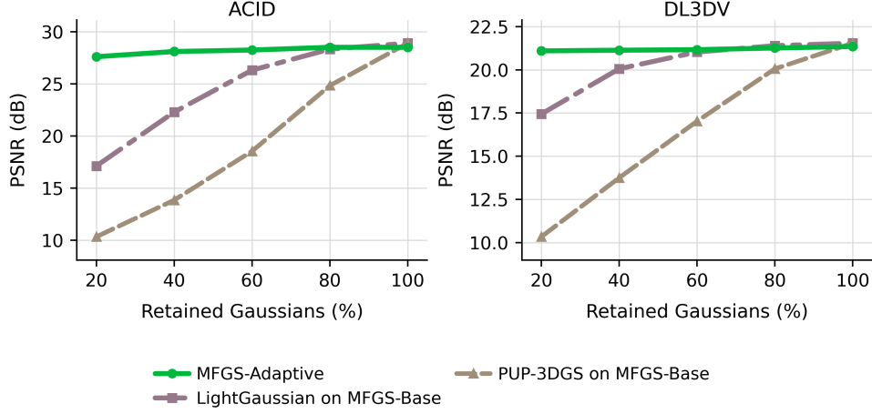
Figure 7: PSNR comparison between the MFGS-Adaptive model and post-hoc pruning baselines across Gaussian keep ratios on ACID and DL3DV at \lambda=0.0256 . LightGaussian and PUP-3DGS are applied to the Gaussians reconstructed by the MFGS-Base model.
