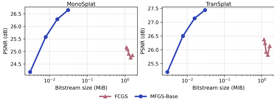
Figure 6: Rate–distortion comparison of the MFGS-Base model and matched FCGS baselines on ACID with MonoSplat and TranSplat.
