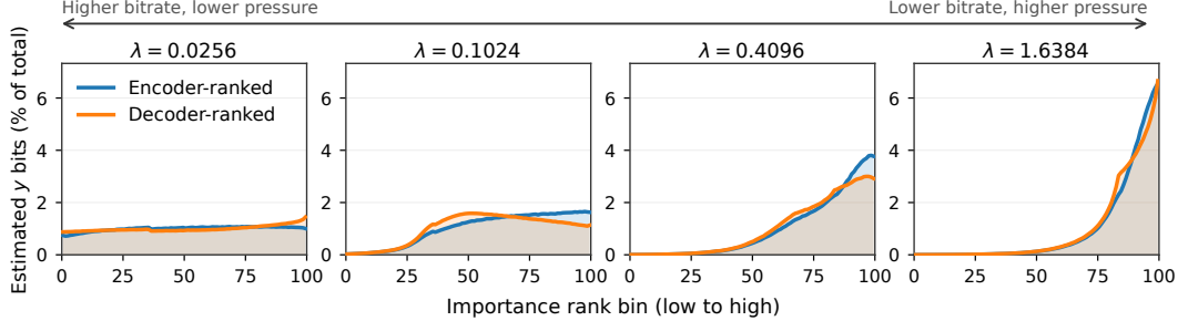
Figure 11: Importance-ranked allocation of estimated main-latent bits on ACID at k = 0.8 . Each panel uses one rate weight \lambda . Curves show the mean percentage of estimated scene-level y bits in each of 100 bins ordered from low to high encoder- or decoder-side importance. Both rankings average all 1,810 scenes at every \lambda .
