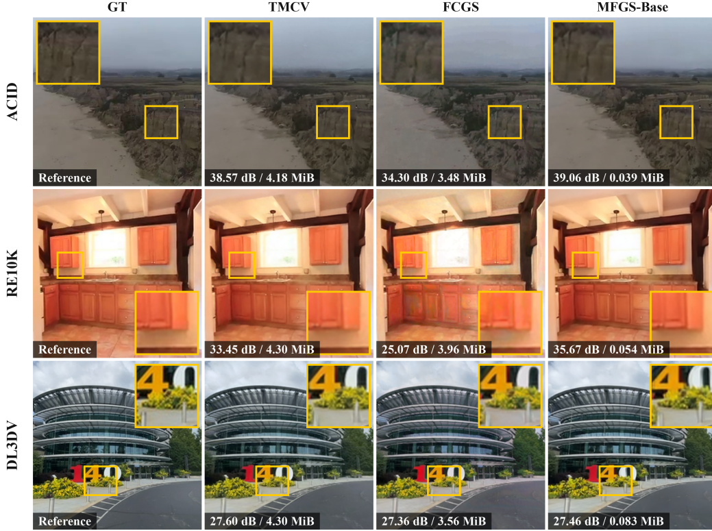
Figure 5: Target-view reconstructions on ACID, RE10K, and DL3DV. FCGS and TMCV compress the output of the standalone MVSplat+ZPressor generator. Yellow boxes mark regions enlarged in the insets. Each panel reports target-view PSNR and the complete scene bitstream size.
