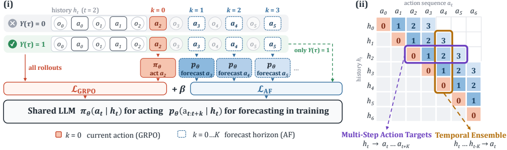
Figure 2: Overview of COPE. (i) Joint training of acting and forecasting. One LLM backbone is shared by both, and \mathcal{L}_{AF} fits the successful action chunk a_{t:t+K} . (ii) Co-evolution of acting and forecasting. Acting helps forecasting via trajectory collection, and forecasting helps acting via implicit temporal ensembling.
