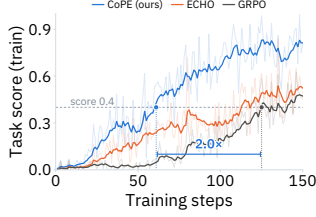
Figure 3: Analysis of sample efficiency. COPE reaches 0.4 in about half the RL steps required by GRPO on ScienceWorld.
