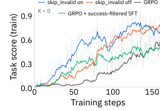
Figure 5: Invalid-action filtering. Replacing invalid action with the next valid one improves the sample efficiency of the K=0 baseline.
