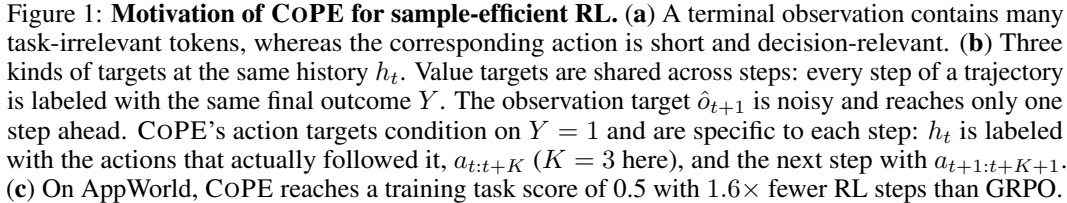
Key challenges. Both existing prediction targets are difficult to construct effectively in complex agentic environments. (1) Value targets are derived from only the shared outcome. A trajectory records only its final outcome, not the success probability of each step, so every step is labeled with this same outcome, whose randomness comes mostly from later actions and observations rather than from the step itself. Distinguishing between steps requires step-level annotations, additional rollouts from intermediate states, or exact recurrence of states across rollouts. (2) Observation targets are noisy and reach only one step ahead. In web navigation or agentic coding, most tokens of the next observation (e.g., HTML DOM trees or verbose terminal logs) are irrelevant to the decision (Fig. 1a), so the prediction loss is dominated by reproducing them. The target also covers only single-step transition; reaching later steps requires chaining predictions, where errors compound.
