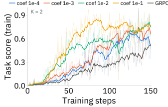
Figure 7: Ablation on action forecasting weight. All coefficients outperform the GRPO baseline; \lambda = 10^{-2} achieves the highest.
