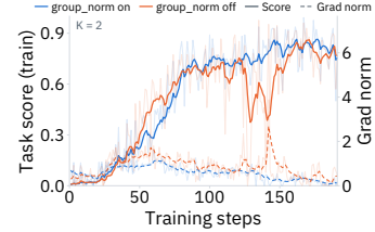
Figure 8: Ablation on group normalization. Normalization suppresses spikes in gradient norms and stabilizes late training.
