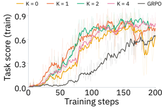
Figure 6: Ablation on forecast horizon K . All K \geq 1 settings outperform GRPO; K = 2 achieves the highest score.
