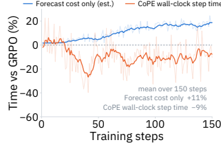
Figure 4: Analysis on wall-clock efficiency. Forecasting adds 11% per-step cost, while end-to-end step time decreases by 9%.
