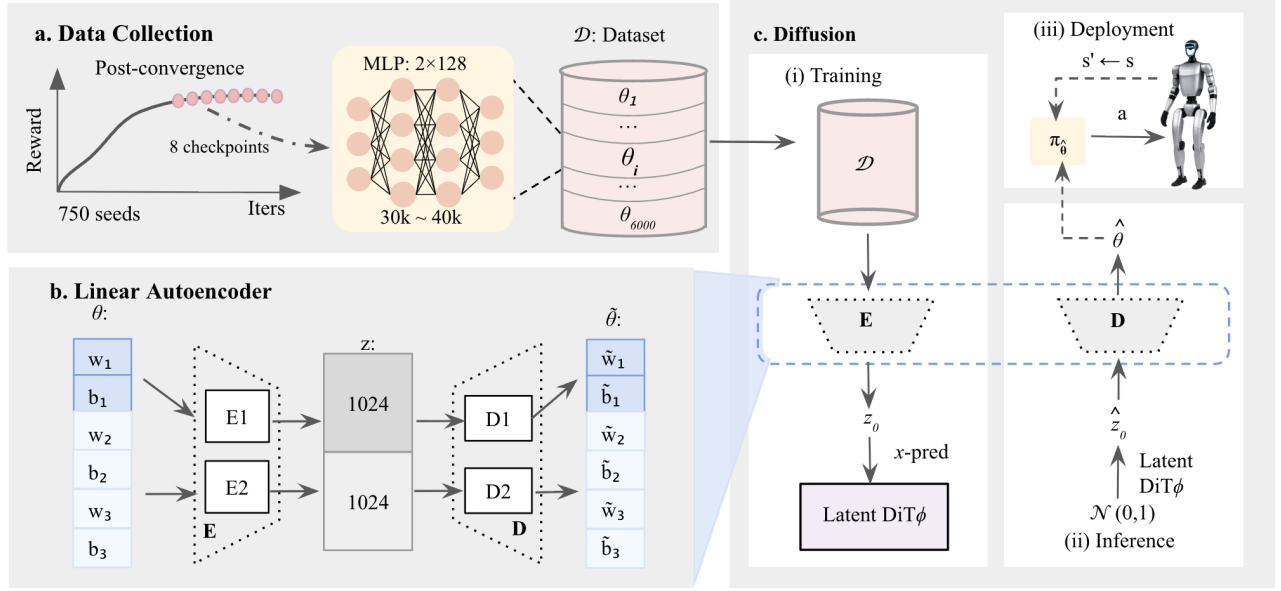
Fig. 2: Method overview. (a) We collect actor weights from 750 training runs with random seeds and retain eight post-convergence networks from each run. Each network is a three-layer MLP. (b) The cluster-wise linear autoencoder is implemented using single-layer encoders and decoders. (c) A diffusion transformer is trained with x -pred loss to model the latent distribution. During inference, the model generates novel network weights that can be deployed in the real world.
