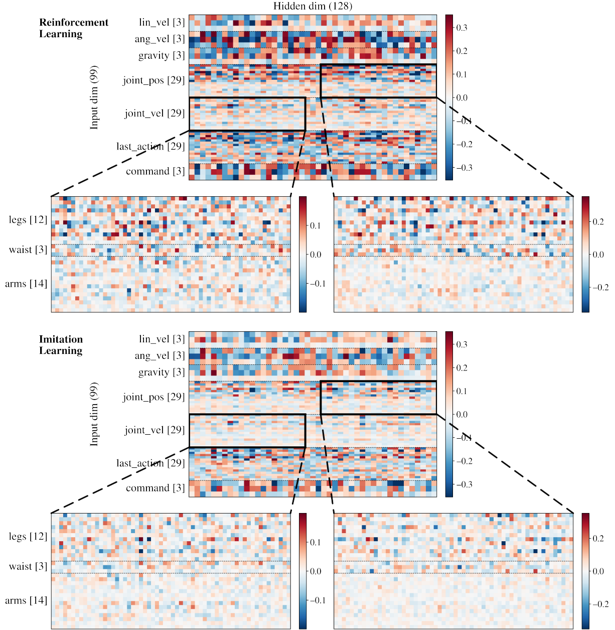
Fig. 5: First-layer weight comparison between RL and IL for walking. Top: RL-trained weight heat map. Bottom: IL-trained weight heat map, distilled from the top RL network. While trained via different optimization objectives, they both exhibit kinematic prior in the first-layer weights.
