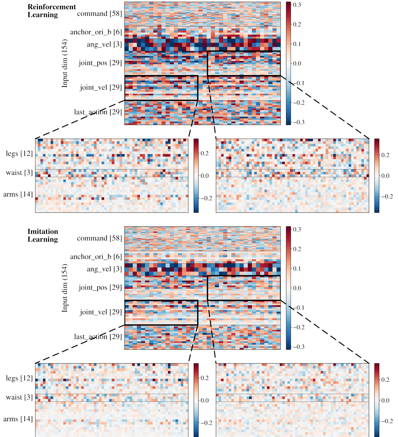
Fig. 11b: First-layer weight comparison between RL and IL for spin kick.
