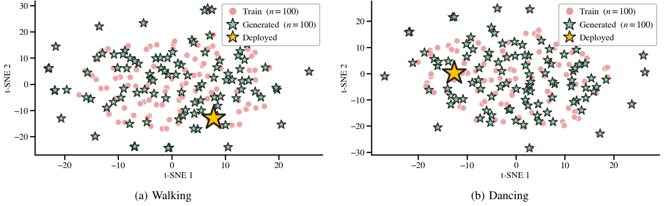
Fig. 8: t-SNE Visualization. Training, generated and deployed network weights for the walking and dancing motions.
