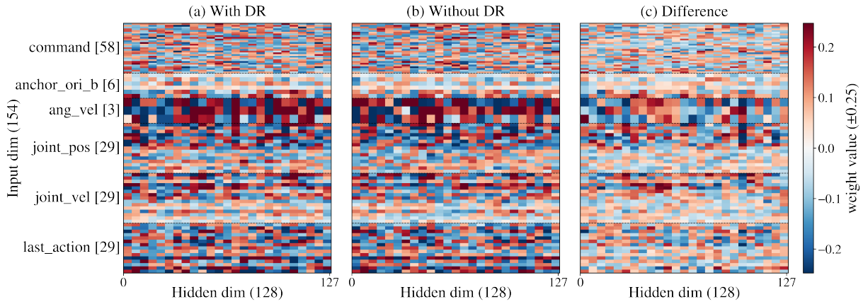
Fig. 7: Effect of domain randomization on first-layer weights for dancing. First-layer weight heat maps of RL networks trained from the same initialization (a) with DR and (b) without DR, together with (c) their element-wise difference. Despite their overall similarity, the structured weight difference resembles the RL-trained weights.
