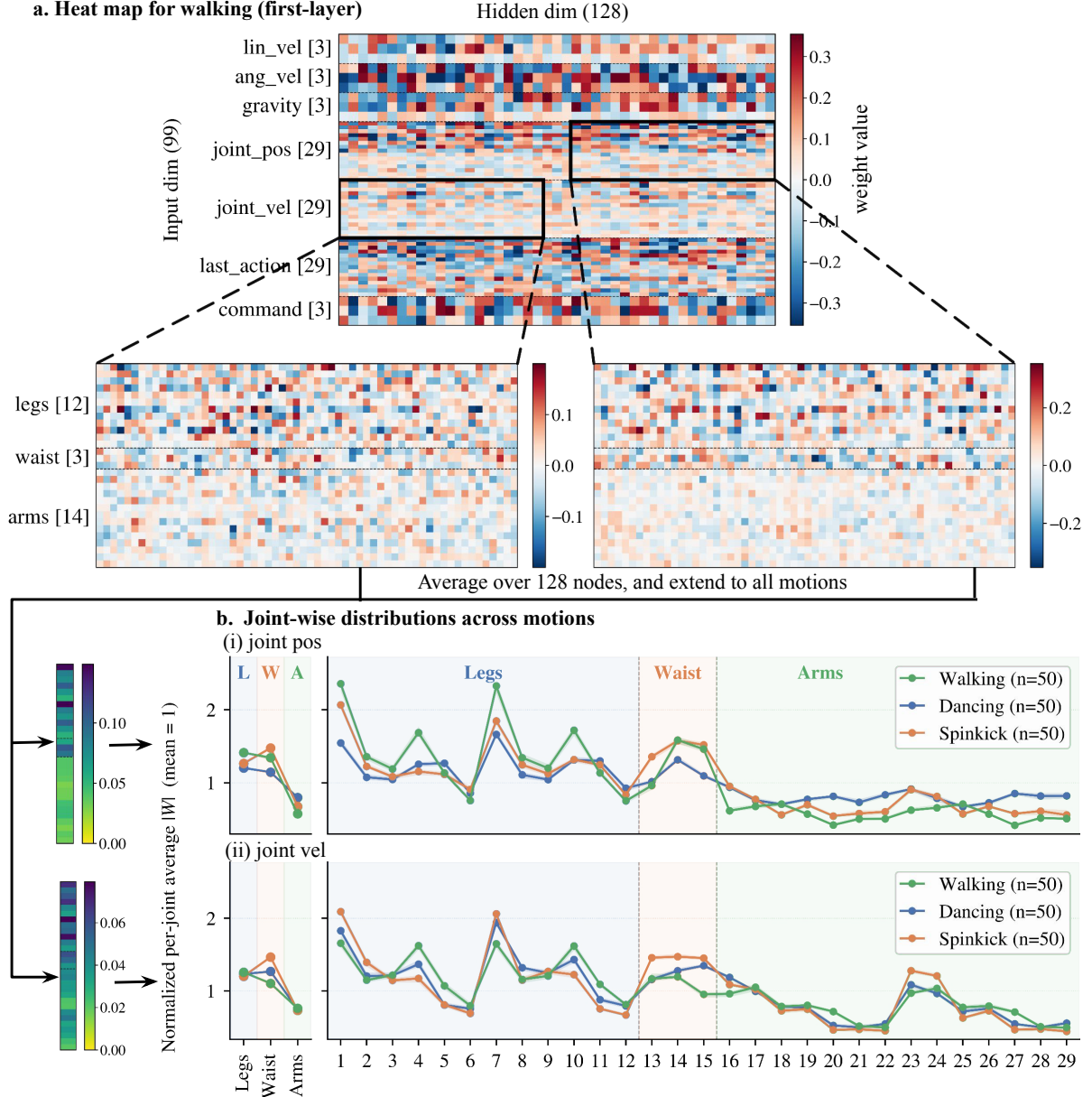
Fig. 4: Kinematic prior in weights. (a) A visualization of the first-layer weight heat map for the walking motion, which reveals a structural principle that certain input regions exhibit larger weight magnitudes. (b) Joint-wise weight distributions across motions demonstrate that hip pitch, knee, and waist joints are assigned higher importance, suggesting the presence of a kinematic prior.
