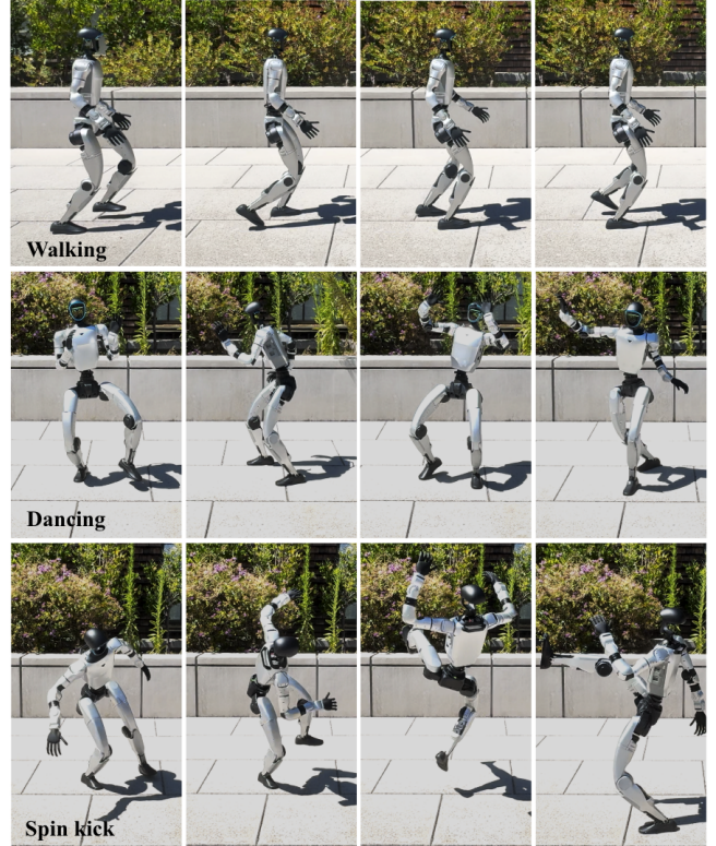
Fig. 1: Real-world deployment of networks with generated weights. Top: A walking motion. Middle: A dancing motion. Bottom: A spin kick motion. For each motion, the corresponding network weights are denoised by a motion-specific diffusion model and subsequently deployed zero shot in the real world.
