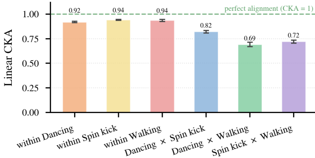
Fig. 9: Subspace similarity across motions. Applying linear CKA to measure subspace similarity on shared inputs across motions, we observe near-perfect alignment within each motion, indicating stable knowledge extraction. Cross motion similarity also remains high, suggesting substantial shared knowledge with minor motion-specific adaptation.
