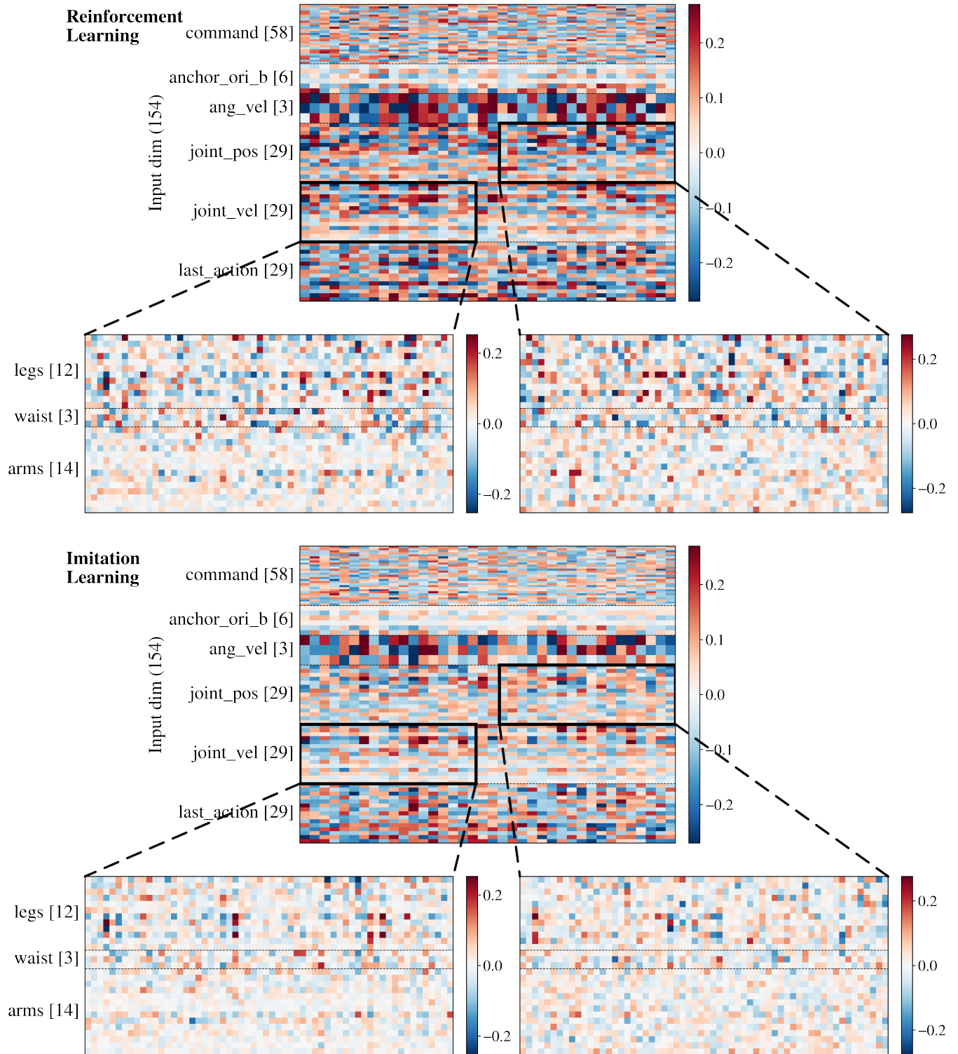
Fig. 11a: First-layer weight comparison between RL and IL for dancing.
