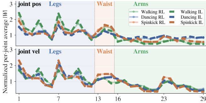
Fig. 6: Kinematic prior for both RL and IL networks. For each motion, the dashed and solid curves largely overlap after distillation, indicating that the first-layer kinematic prior is preserved in the IL network.
