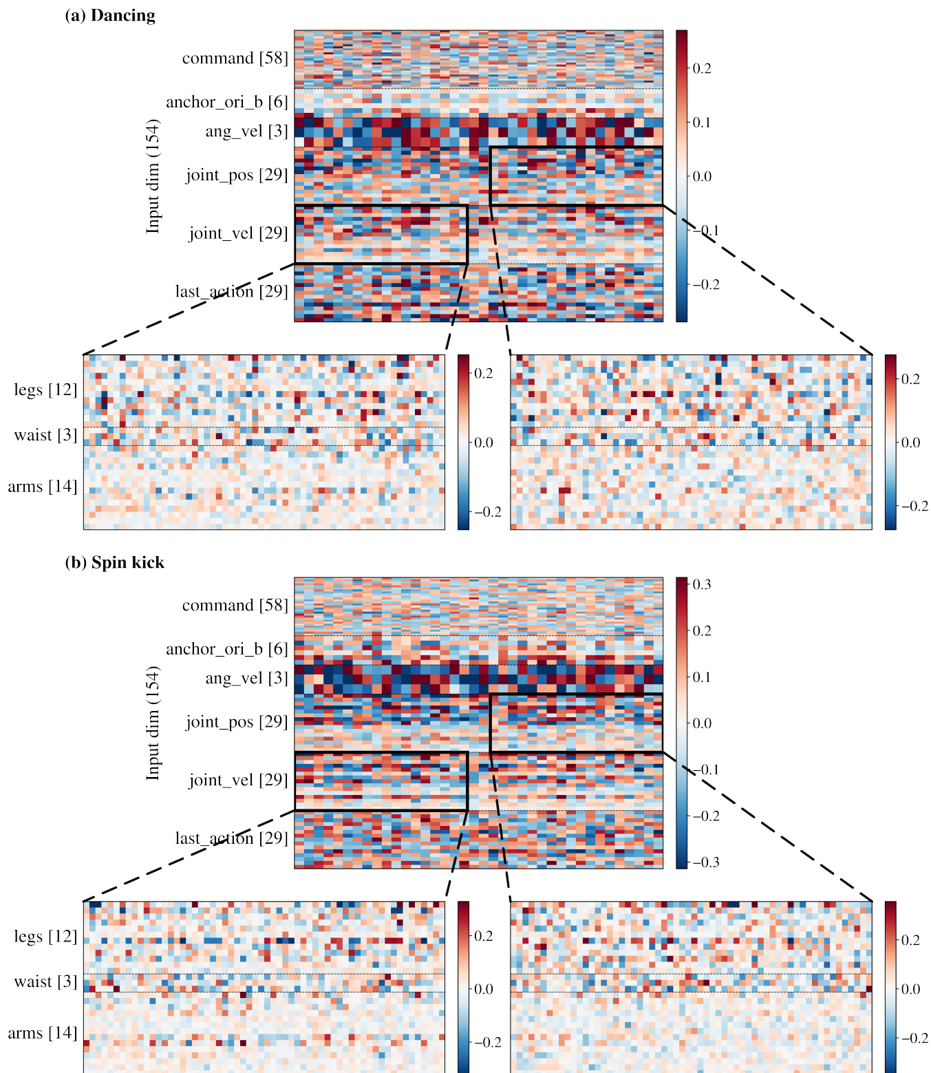
Fig. 10: First-layer heat maps. (a) Dancing weight heat map. (b) Spin kick weight heat map. The first-layer weights consistently exhibit the structural principle across joints.
