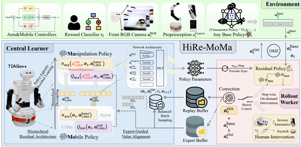
Figure 2: HiRe-MoMa Framework enables policy-agnostic real-world fine-tuning of mobile manipulators through an asynchronous residual reinforcement learning paradigm. (Right) Shared-Control Rollout: an on-board rollout worker augments a frozen base policy with learnable residuals; sparse human interventions during critical or hazardous phases are stored in an expert buffer. (Left) Asynchronous Central Learner: the residual policy is optimized along two pillars: a) a Hierarchical Residual Architecture (Sec. 4.1) that decouples the residual into mobile and manipulator heads with unidirectional conditioning, embedding the platform’s physical hierarchy directly into the policy; and b) an Expert-Guided Value Alignment loss (Sec. 4.2) that fuses sparse environment rewards with sparse human corrections to reshape the critic toward expert-preferred behaviors.
