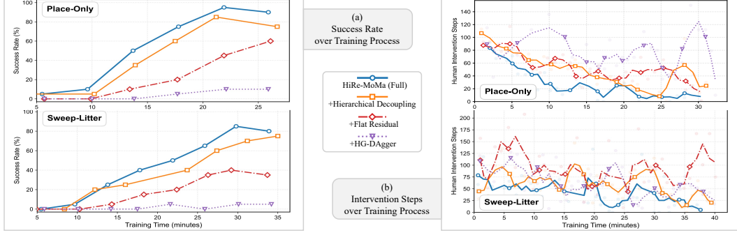
Figure 4: Training Dynamics. Comparison across methods over training time, where we construct the figure along the actual training time. (a) Success rate: HiRe-MoMa(full) attains a consistently higher success rate throughout training, validating the effectiveness of our design combining hierarchical residual architecture and alignment. (b) Human intervention steps: HiRe-MoMa requires fewer human interventions and converges faster than the baselines, and the comparison with and without alignment ( +Hierarchical Decoupling ) demonstrates the effectiveness of the extra alignment loss.
