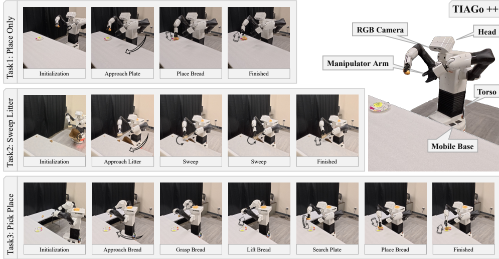
Figure 3: Real-World Experimental Tasks. Our evaluation encompasses three tasks, Place Only , Sweep Litter , and Pick Place , that demand varying levels of inter-module coordination. These tasks are particularly challenging for mobile manipulators as they require the simultaneous optimization of base positioning and arm reaching, where minor misalignments in the platform’s pose propagate as significant errors at the end-effector.
