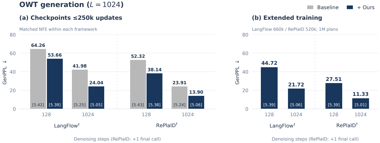
Figure 2 | Generation results on OWT ( L = 1024 ). (a) Baseline and LANGDiT at 128/1,024 denoising steps using checkpoints within 250k updates. The LangFlow comparisons use 250k checkpoints at 128 NFE and 180k checkpoints at 1,024 NFE. RePlaID compares 40k versus 150k at 128 steps and 220k versus 250k at 1,024 steps, so these pairs do not match training progress; the latter also differs in planned budget. (b) Extended-training checkpoints: LangFlow 660k and RePlaID 520k from 1M-update plans. RePlaID requires one final denoiser call beyond the displayed step count. Bars show GenPPL; bracketed values show mean per-sample unigram entropy. All results use 1,024 samples and EMA weights; † denotes our implementation (Table 3).
