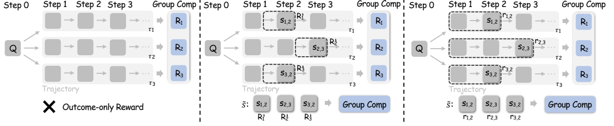
Figure 1: Comparison of credit assignment in deep search agents. Left: GRPO uses episode-level advantages from terminal rewards ( R_1, R_2, R_3 ) without intermediate feedback. Middle: GiGPO matches environment states ( \tilde{s} ) but suffers from severe fragmentation under heterogeneous observations. Right: KnowGPO abstracts heterogeneous states into knowledge states ( s_{i,t} ) and computes step-level advantages from incremental knowledge gains ( r_{i,t} ).
