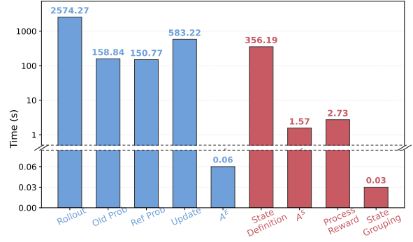
Figure 4: Per-iteration training time breakdown. Blue bars represent shared RL operations common to both GRPO and KnowGPO; red bars represent KnowGPO-specific components.
