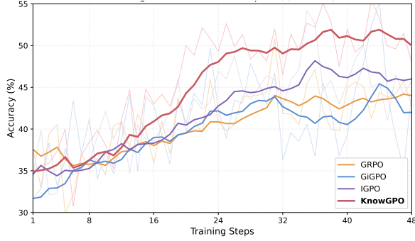
Figure 3: Training curves comparing GRPO, GiGPO, IGPO, and KnowGPO on our Qwen3-8B-SFT.
