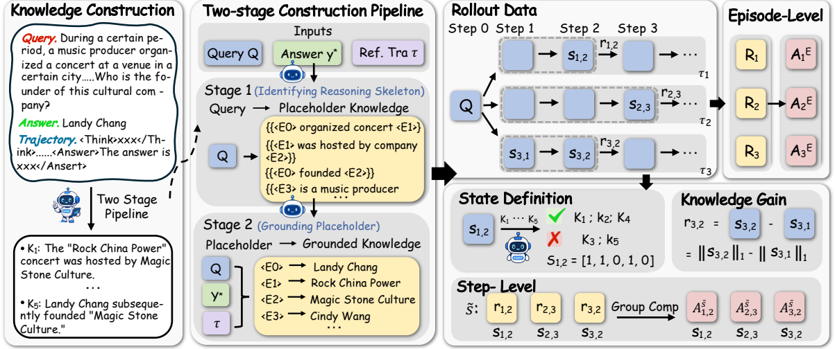
Figure 2: Overview of the KnowGPO framework. Left: Knowledge condition construction via a two-stage pipeline, illustrated with an example. Right: Rollout trajectories are grouped by matched knowledge states; step-level advantages are computed from incremental knowledge gains via group-relative comparisons.
