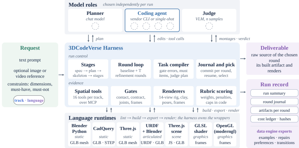
Figure 7: Components and model roles. A planner, a judge, and a coding agent are configured modularly per run; the harness orchestrates stage progression, iterative refinement, and candidate selection while providing deterministic spatial tools, verification gates, multi-view renderers, and rubric aggregation. Agent programs execute across seven isolated language runtimes; dashed circles indicate pluggable model interfaces.
