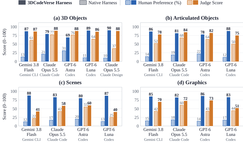
Figure 4: Main results of 3DCodeVerse Harness across four 3D coding tasks. Panels show (a) 3D objects, (b) articulated objects, (c) scenes, and (d) graphics. Blue bars report Human Preference (%), and orange bars report Judge Score (0–100; failed generations receive a score of zero). Hatched bars denote each backbone’s native harness, while solid bars denote 3DCodeVerse Harness. The final group in (a) compares Claude Design with 3DCodeVerse Harness, both using Claude Opus 5.5.
