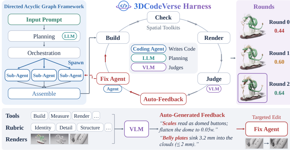
Figure 3: Overview of the 3DCodeVerse Harness. Given an input prompt, an LLM planner defines the target asset, and a DAG coordinates sub-agents to code and assemble a 3D program (left). Execution checks, spatial measurements, and rubric-guided VLM judgments provide automated feedback (center) for targeted code revisions by a fix agent (bottom). The right panel illustrates successive refinement rounds, with the highest-scoring program selected as the final output.
