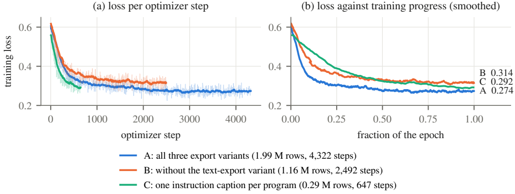
Figure 14: Training loss dynamics of the three Qwen3.8-27B data-scale runs. (a) Cross-entropy loss per optimizer step; faint curves show raw 5-step logs and solid curves show an exponential moving average ( \tau = 50 steps). (b) Smoothed loss trajectories plotted against epoch fraction to align cosine learning-rate schedules, annotated with terminal smoothed losses. Each trajectory tracks in-distribution optimization across its respective representation mixture from 293 K to 1.99 M rows.
