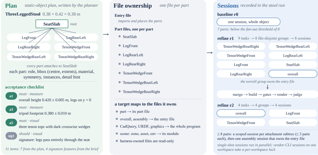
Figure 8: From structural plan to file scopes and coding sessions , illustrated on the recorded trajectory of §A.6. The planner decomposes the prompt into named parts with metric bounding boxes, materials, attachment relations, and an acceptance checklist; each target maps to its owned source files, and refinement tasks sharing files are grouped into file-disjoint sessions. In Round 1, nine revision tasks partition into eight file-disjoint groups; in Round 2, four tasks form four groups.
