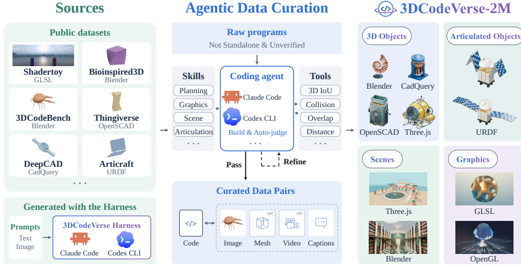
Figure 2: Curation and composition of 3DCodeVerse-2M. Left: We collect programs from public datasets and generate more with our harness. Middle: Our 3D coding harness, equipped with modeling skills and inspection tools (e.g., 3D IoU, collision checks), builds each program, judges the output, and refines it until it passes. Each verified program is paired with rendered images and captions, plus meshes and videos when available. Right: The resulting corpus covers 3D objects, articulated objects, scenes, and graphics across multiple programming languages and engines.
