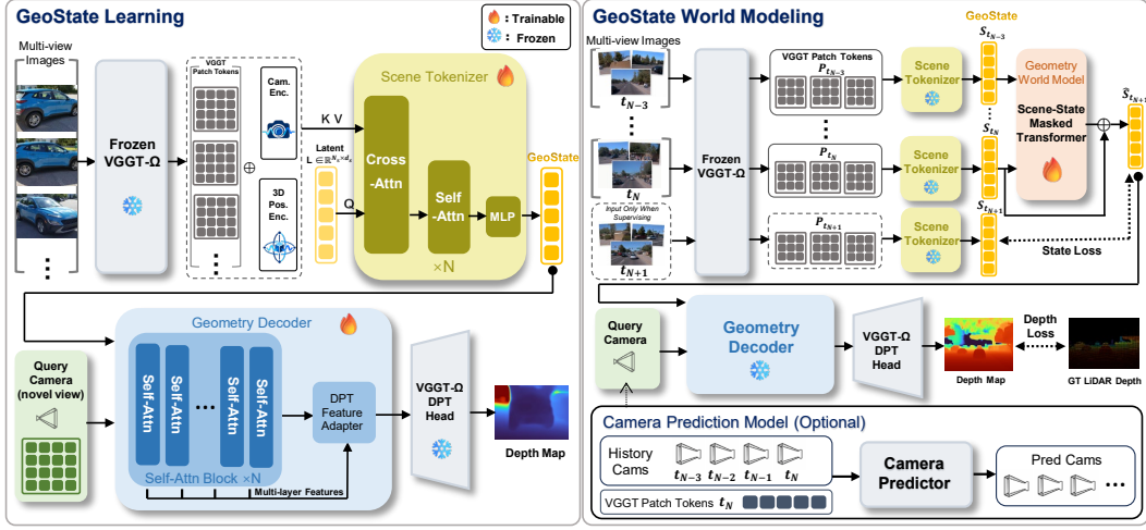
Figure 1: Overview of GeoState. GeoState Learning constructs view-decoupled scene states with a scene tokenizer and query-conditioned geometry decoder. GeoState World Modeling predicts future states directly in this representation space.
