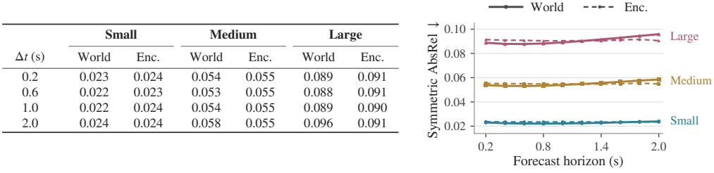
Figure 3: Cross-query geometric consistency on Waymo. We evaluate symmetric reprojection AbsRel ( \downarrow ) across perturbation levels.
