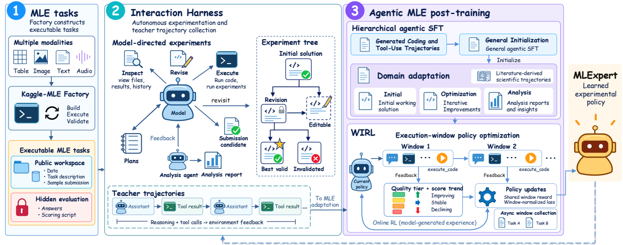
Figure 2 | Overview of MLEExpert training for autonomous MLE. The Kaggle-MLE Factory constructs executable tasks, and the interaction harness supports model-directed experimentation and trajectory collection. Hierarchical agentic SFT learns from demonstrations, while WIRL further optimizes the policy from execution feedback collected during online interaction.
