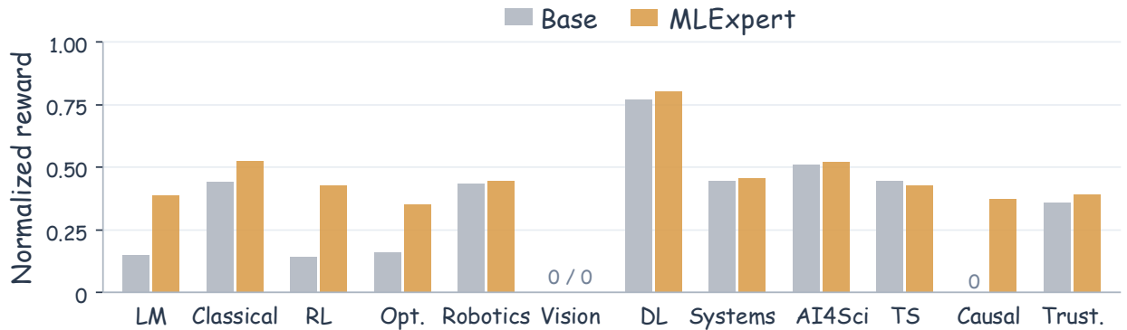
Figure 4 | Algorithm-component optimization on 12 selected MLS-Bench-Lite tasks. Bars show normalized verifier rewards for Base and MLExpert.
