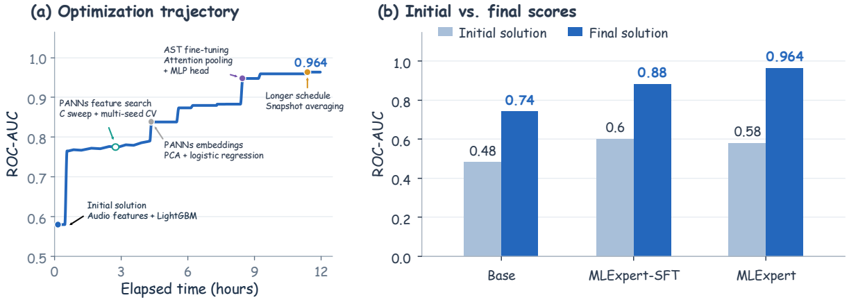
Figure 3 | Long-horizon optimization on MLSP 2013 Birds. (a) Representative optimization progress of MLExpert. (b) Initial and final ROC-AUC for Base, MLExpert-SFT, and MLExpert.
