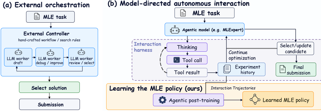
Figure 1 | Decision making in long-horizon MLE optimization. (a) External orchestration organizes optimization through predefined workflows and search rules. (b) In model-directed interaction, the model selects subsequent actions based on experimental states and execution feedback.
