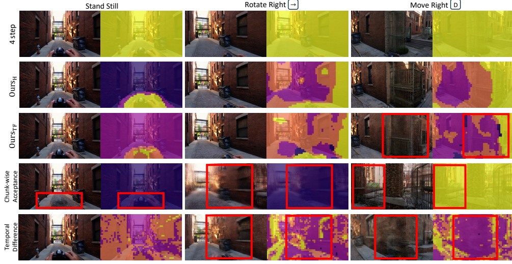
Figure 5: Qualitative ablations of verification and commitment granularity. Our learned verifier handles distortions that challenge training-free verification. Premature chunk-wise acceptance propagates errors to later chunks, while motion-based verification struggles to distinguish camera-induced changes from distortions.
