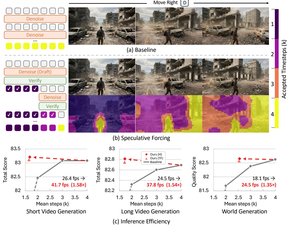
Figure 1: Compared with full-step sampling (a), Speculative Forcing treats intermediate token estimates as drafts, accepts those that have converged, and refines only the rest (b), achieving comparable quality with fewer denoising steps and higher throughput (c).
