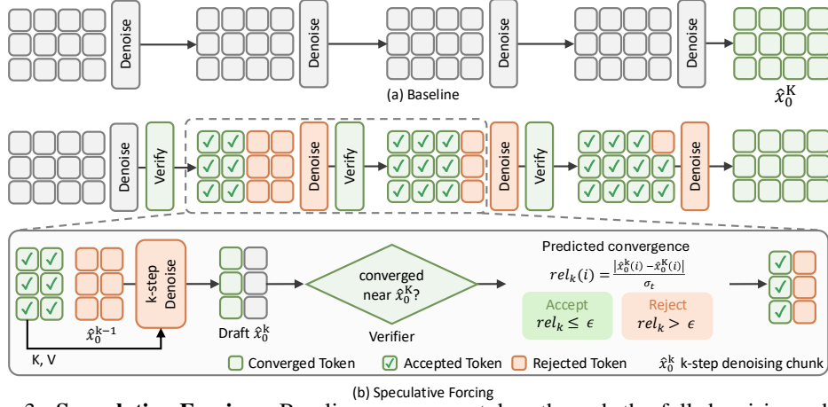
Figure 3: Speculative Forcing. Baseline runs every token through the full denoising schedule. Speculative Forcing instead treats each token’s intermediate clean estimate as a draft and asks a verifier to predict its remaining gap rel_k(i) to the full-step output. Tokens predicted to have converged are accepted and committed, after which they enter the next step only as keys and values, so the following denoising pass is computed for the rejected tokens alone.
