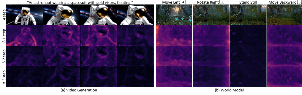
Figure 2: Token-wise convergence during denoising. We visualize latent differences between each chunk’s k -step prediction and the baseline four-step output. (a) In video generation, background and object regions that remain similar to history tend to converge early, while other regions continue to change. (b) In world generation, previously observed regions often converge early, whereas newly revealed regions tend to require further denoising.
