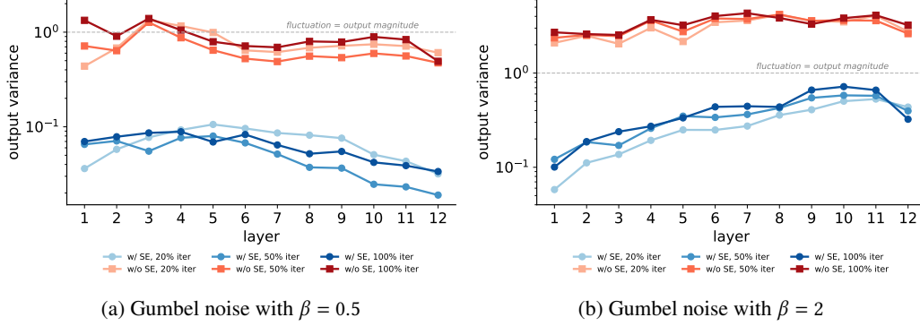
Figure 6: Router variance under different levels of Gumbel perturbation.
