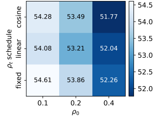
Figure 5: Hyperparameters.
