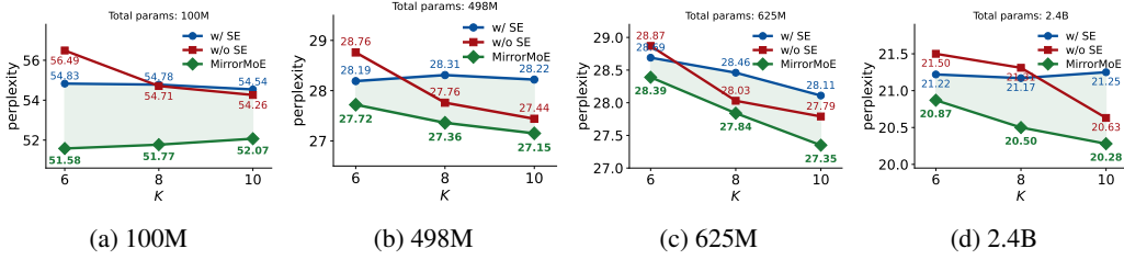
Figure 1: Comparison of MoEs with and without shared experts (SE) and the proposed MirrorMoE. MirrorMoE consistently i) achieves the best performance, ii) realizes the expressiveness gains from larger K , and iii) enables shared-expert MoEs to outperform their non-shared counterparts.
