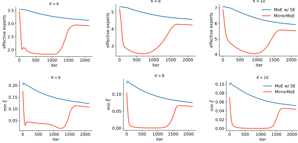
Figure 4: Preview of how MirrorMoE in Alg.1 actively suppresses experts on a 100M MoE model. The rebound in K_{\text{eff}} results from annealing \rho .
