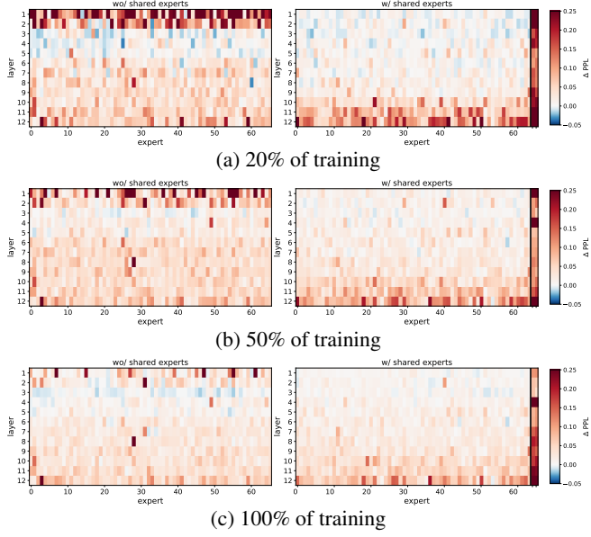
Figure 2: Perplexity increase after ablating individual experts. In the right subplot, the two rightmost columns, separated by a solid line, correspond to shared experts.
