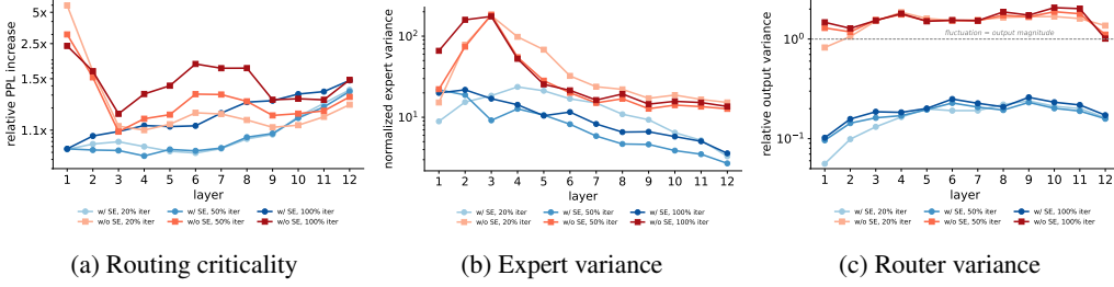
Figure 3: Shared experts make MoE routing less exploratory.
