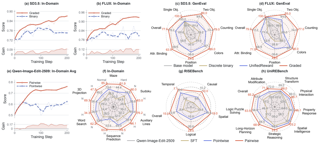
Figure 1: Panels (a)–(d) highlight the advantages of the graded verifier over the binary verifier as a generative reward model, while panels (e)–(h) show that pairwise verification provides more reliable and accurate feedback signals than pointwise verification.
