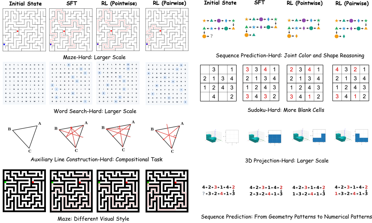
Figure 4: Qualitative visualization of rule-governed world-modeling tasks.
