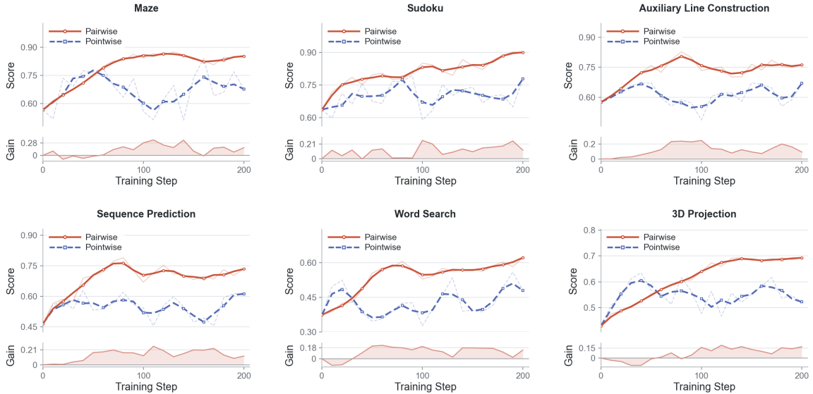
Figure 5: Training dynamics of pairwise and pointwise verification across six rule-governed tasks. Each panel shows validation scores and the score gap between the two methods.
