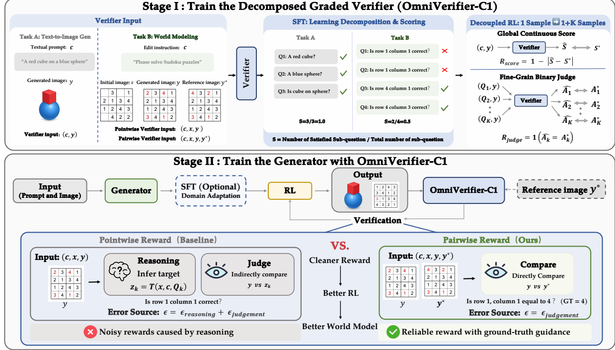
Figure 2: Overview of our training pipeline. Stage 1 trains the Decomposed Graded Verifier with decoupled reinforcement learning to produce fine-grained continuous rewards. Stage 2 introduces a pairwise judgment paradigm that provides cleaner and more reliable reward signals for generative model reinforcement learning.
