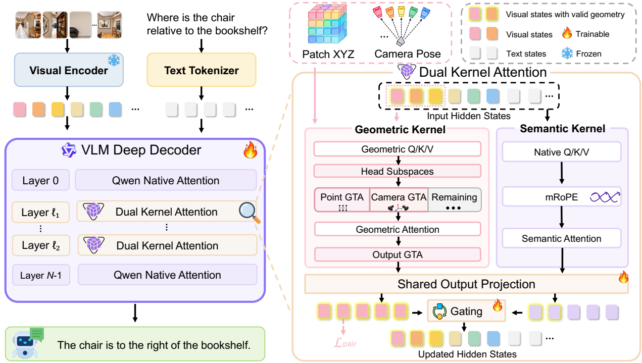
Figure 2. Geometry as Position via Dual-Kernel Attention. Selected decoder layers retain the backbone-native semantic kernel and introduce a geometric kernel over geometry-valid visual tokens. A learned gate fuses both outputs into the shared residual stream, while \mathcal{L}_{\text{pair}} directly supervises the pre-fusion geometric representation during training.
