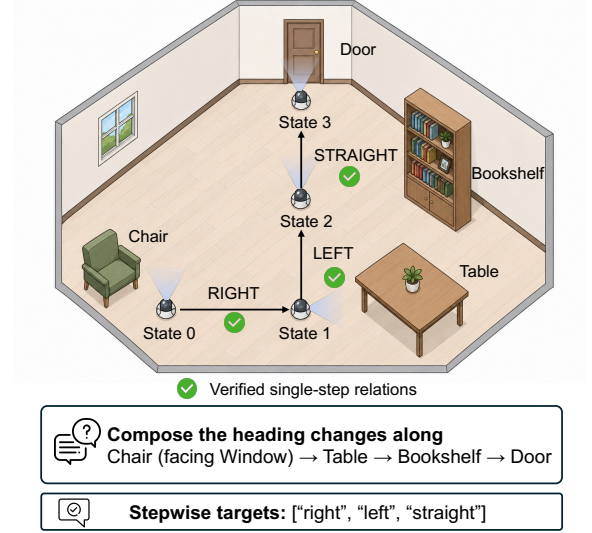
Figure 3. Reference-frame composition. Verified single-step relations sharing end-points form a training chain with stepwise turn targets.
