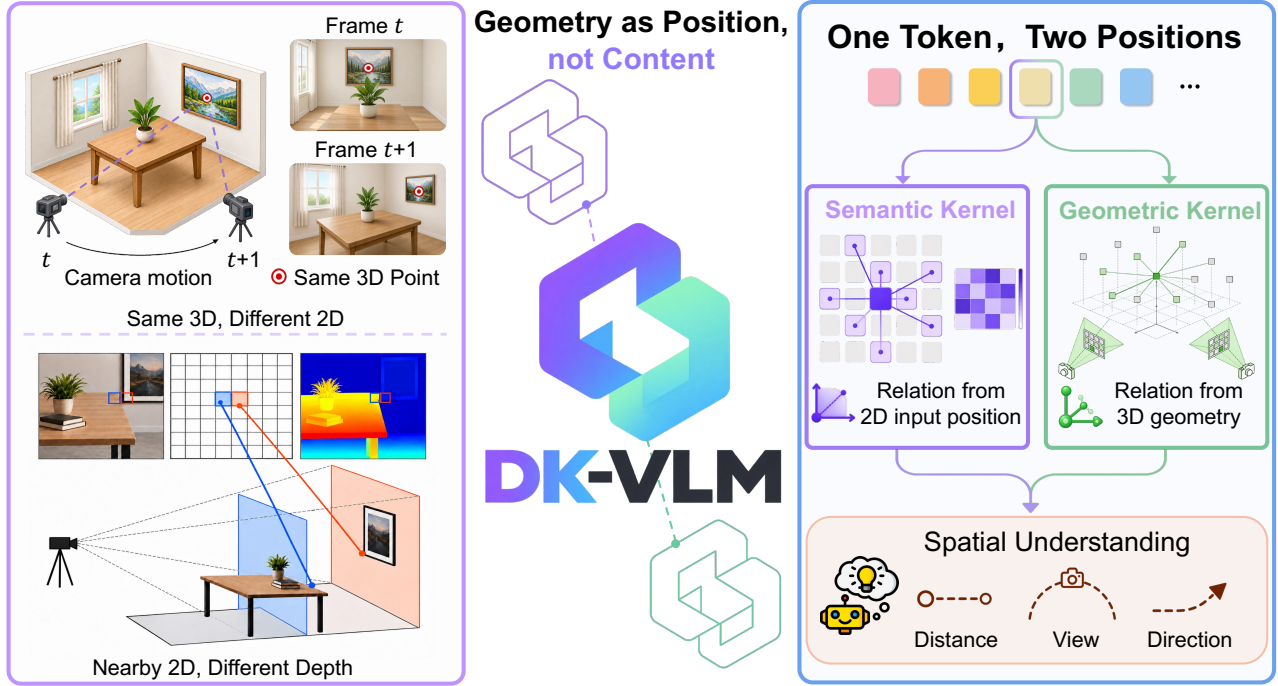
Figure 1. Geometry as position in DK-VLM. Left: 2D input positions do not fully capture 3D relations. Right: DK-VLM retains the native positional encoding and introduces scene geometry into attention as position.
