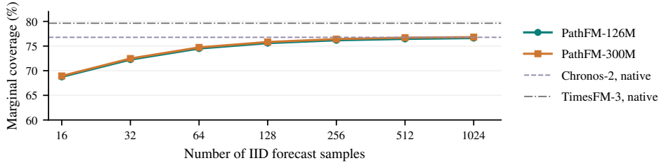
Figure 11: Marginal 80% interval coverage versus the number of forecast samples on fev-bench. Both model sizes use iid sampling. Horizontal references use the native 10th and 90th percentile outputs of Chronos-2 and TimesFM-3.
