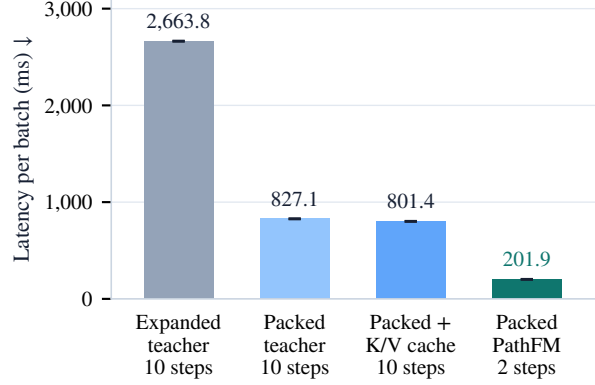
Figure 12: Inference speedup breakdown on an A100 at batch 16, context 2,048, and horizon 480. The teacher uses ten Euler evaluations; the student uses two. All configurations use float32 weights with bfloat16 autocast.
