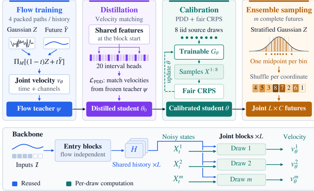
Figure 2: Training, post-training, and sampling with PathFM. Flow matching learns a joint velocity field; distillation matches frozen-teacher velocities at student-proposed states. Calibration maps eight iid draws through one fused step of trainable G_\theta to samples scored by fair CRPS, together with PDD supervision. Sampling uses stratified initial noise to improve coverage of the noise distribution with a small ensemble. Below: Flow enters after the flow-independent prefix, and history attention values are computed once and reused by separate packed future states.
