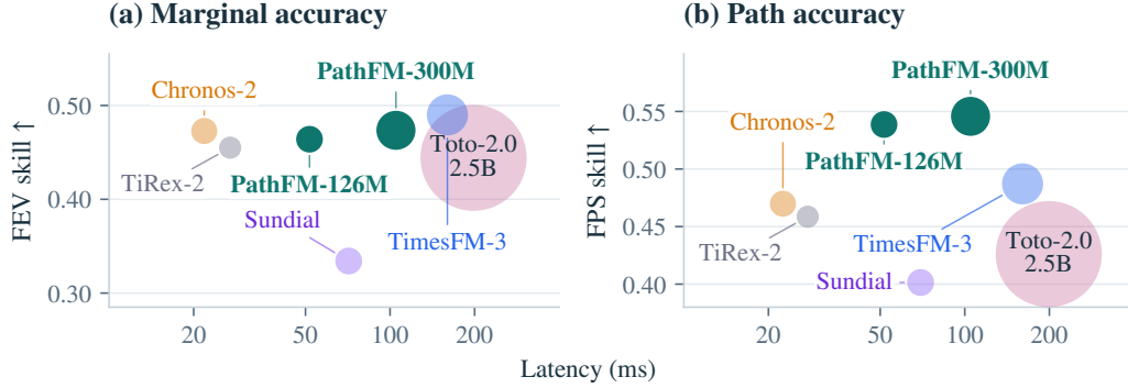
Figure 10: Accuracy, latency, and model size with the 300M PathFM variant. Circle area denotes parameter count. Latency is the median time to return nine quantiles (a) or forecast paths (b) for one query on an NVIDIA L4 at context 2,048 and horizon 288. Accuracy uses the native benchmark settings.
