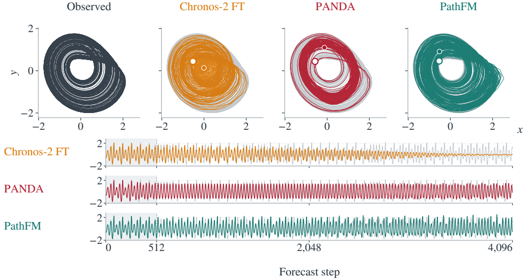
Figure 15: Full 4,096-step Lorenz and Rössler continuations. All panels use the same initial conditions. Gray curves show the observed continuation; circles mark the first and last forecast states, and shading marks the first 512 steps.
