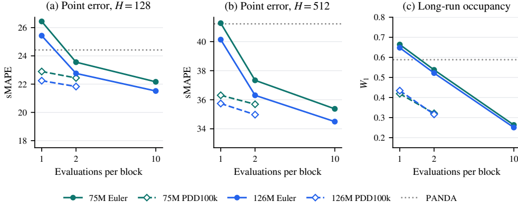
Figure 14: Accuracy versus sampler budget for both model sizes. Point errors average all 480 source groups; W_1 averages all 135 systems and uses 4,096-step sampled continuations. The dotted horizontal line marks PANDA; lower is better.
