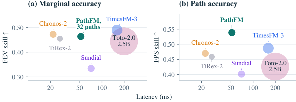
Figure 4: Accuracy, latency, and model size across six forecasting models. Area denotes parameter count. Latency is the median time to return nine quantiles (a) or forecast paths (b) per query on an NVIDIA L4, with history and forecast lengths fixed across models. Quantile models use their better aggregate completion from Section 4.
