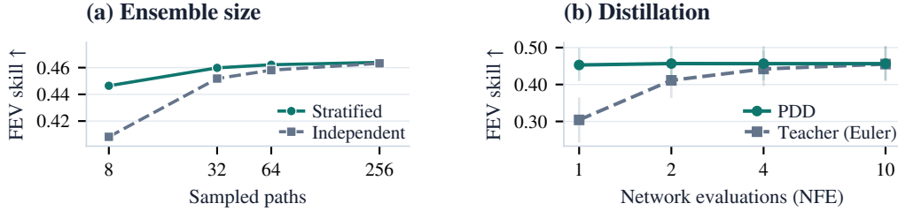
Figure 5: Ensemble size and distillation on fev-bench tasks. (a) Calibrated 126M model with different sampling strategies at NFE=1 (Section C.1.2). (b) Its matched teacher and PDD student. Thin bars in (b) show pointwise 95% task-bootstrap intervals (Section B.3).
