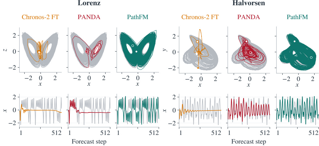
Figure 7: Lorenz and Halvorsen continuations; PathFM uses one sampled path. Each column shows a full 4,096-step portrait above its first 512 x -coordinate steps. Gray curves show the observed continuation; open and filled circles mark the first and last forecast states.
