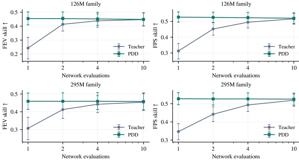
Figure 8: Teacher–student accuracy at different evaluation budgets. Rows show teacher–student pairs from the 126M and 295M families; columns show FEV and six-component FPS skill, with higher values preferred. NFE uses a logarithmic horizontal axis. Thin vertical bars show pointwise 95% task-bootstrap intervals from 2,000 resamples.
