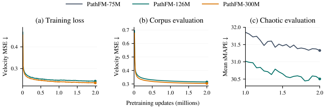
Figure 6: Pretraining progress on general and chaotic time series. (a) Training velocity MSE; (b) EMA velocity MSE on fixed corpus windows for PathFM-126M and PathFM-300M; (c) EMA mean validation sMAPE for the 75M and 126M chaotic models at horizon 256, zoomed to 1M–2M updates.
