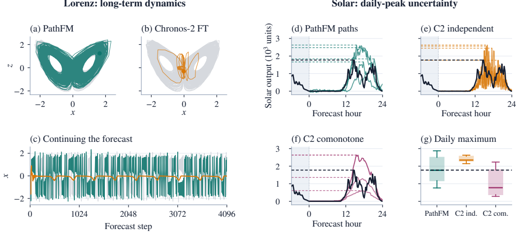
Figure 1: Two advantages of trajectory generation. Left: a sampled Lorenz rollout sustains variability and a two-lobe structure, while the fine-tuned Chronos-2 trace contracts. Both use the dynamical models in Section 6. Gray Lorenz curves show the observed continuation. Right: solar-output paths from PathFM and independent (ind.) and comonotone (com.) completions of the Chronos-2 (C2) quantiles. Horizontal dashed lines marks each solar path’s daily maximum; black denotes the observed future. In (g), boxes show medians and interquartile ranges across 32 paths, whiskers show the 10–90% range, and the dashed line marks the observed maximum.
