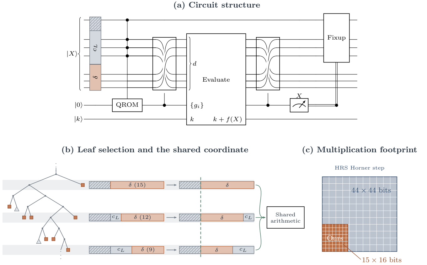
FIG. S3 Co-designed HHL rotation-angle circuit. (a) Complete reversible dataflow: a dyadic lookup selects a local quadratic and a cyclic shift, the input is mapped into a shared local coordinate, and the quadratic is accumulated directly into k . The inverse shift restores X ; measurement and a shared phase correction clear the consumed coefficients without reversing the lookup. (b) Dyadic leaves and the shared coordinate. Power-of-two-aligned leaves are selected by the leading input bits. Shifting each leaf’s varying bits \delta to a common scale allows leaves of different widths to feed one 15-bit polynomial-evaluation stage without subtraction or arithmetic rescaling. (c) Arithmetic consequence: the circuit multiplies the 15-bit coordinate by a 16-bit slope, compared with 44 \times 44 bits for each multiplication in the general HRS Horner polynomial-evaluation stage.
