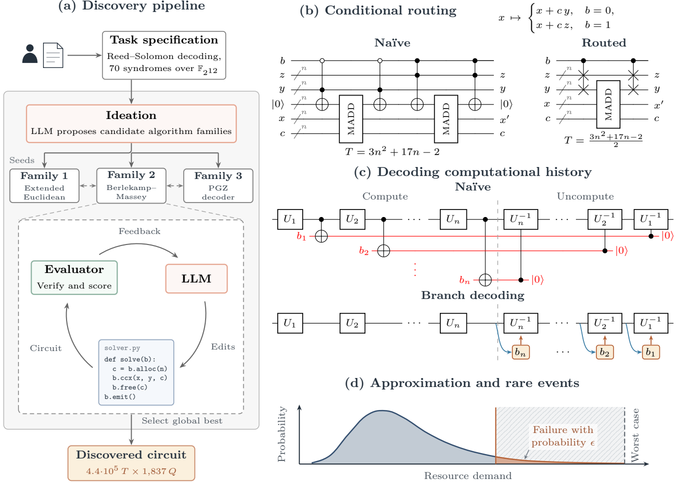
FIG. 1 Overview of the circuit-discovery framework. (a) A hand-written task specification defines the circuit design task (for example, Reed-Solomon decoding) and is given to an LLM. The LLM proposes architecturally different approaches ( algorithm families ; here extended Euclidean, Berlekamp-Massey, and Peterson-Gorenstein-Zierler (PGZ) decoders), which are then developed and optimized in parallel. Strong candidates are periodically shared between families to allow for cross-pollination of useful ideas. (b) Conditional routing reduces the cost of coherent control flow: for instance, two controlled multiply-adds (MADDs) become inexpensive controlled swaps and one shared arithmetic block. (c) Branch decisions that a naïve reversible computation stores during the forward pass (red) can instead be decoded from the current state during uncomputation. (d) When an application permits bounded error, allowing rare failures on atypical, costly inputs reduces resource requirements.
