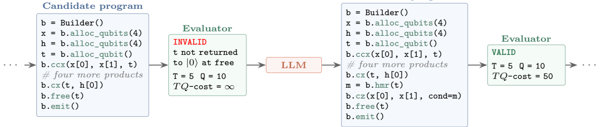
Extended Data Figure 1 Sample inputs and outputs for inversion in \mathbb{F}_{2^4} . (a) During ideation, the LLM is given the complete task specification but no prior implementation and returns distinct candidate architectures. (b) During evolution, the input additionally contains a selected parent program, its evaluator feedback, and limited archive context; the LLM returns a proposed rewrite. (c) One such rewrite computes the inverse with five nonlinear products but fails to return an ancilla to |0\rangle , so the evaluator rejects it. Seeing this feedback, the LLM adds MBU; the resulting circuit is valid with T = 5 , Q = 10 , and a TQ -cost of 50.
