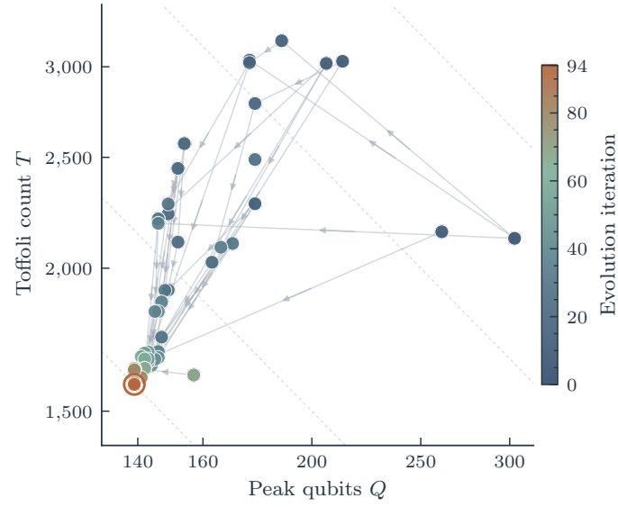
Extended Data Figure 2 Search lineage for the Gaussian circuit in the resource plane. Each marker is a distinct valid circuit, colored by the iteration in which it was discovered; arrows point from each parent to its mutated child. Dashed curves are contours of constant TQ -cost, which decreases toward the lower left. The ring marks the discovered circuit at T = 1,583 and Q = 139 .
