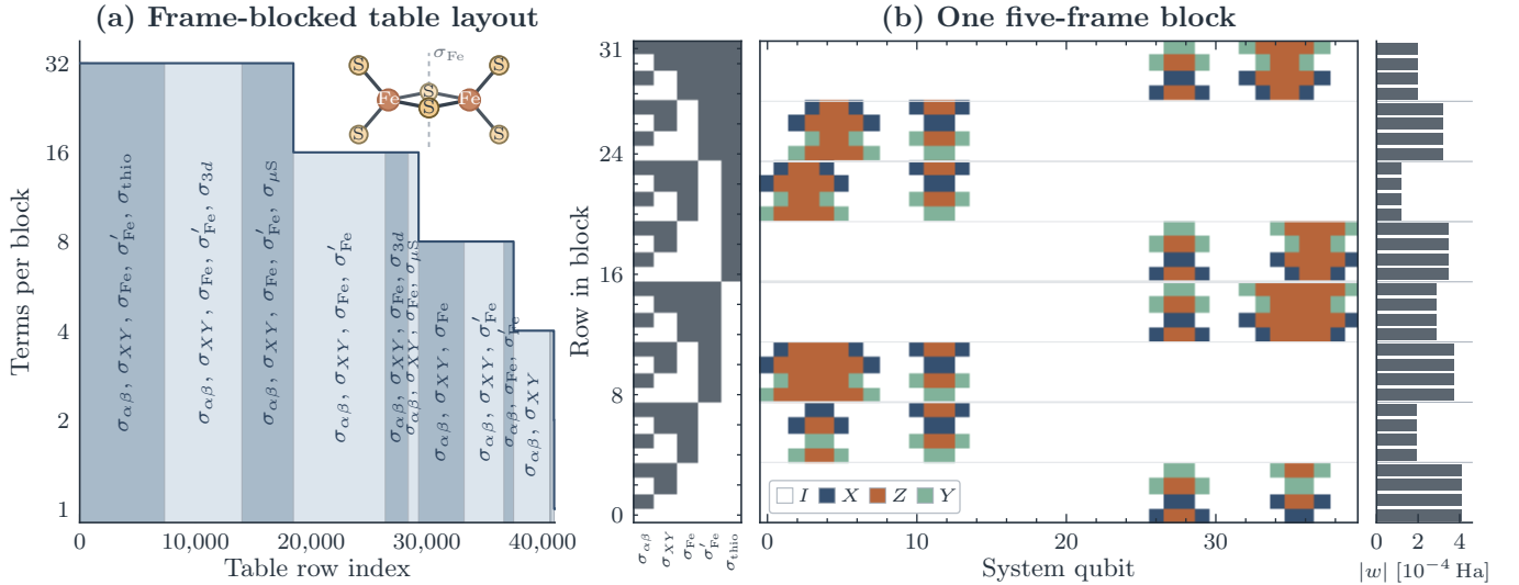
FIG. S4 Frame structure of the Fe 2 S 2 alias table. (a) The preprocessing places Pauli operators related by fixed Clifford frames into contiguous blocks. This groups the 41,052 table rows into 3,221 blocks that SELECT handles as units. Band height gives the number of terms in each block, and the labels give the frames used to generate them. Inset: the Fe 2 S 2 cluster core (thiolate substituents omitted); the dashed line marks the iron-site reflection \sigma_{Fe} . (b) One block of 32 Pauli operators generated from a representative operator using five frames. Each row of the left matrix specifies which frames are applied; a dark cell means that the frame named below its column is included. The center shows the resulting Pauli operator on the 40 system qubits, and the bar on the right gives its coefficient magnitude. The spin frames \sigma_{\alpha\beta} and \sigma_{XY} , shown in the first two columns, preserve coefficient magnitudes and therefore produce equal-weight groups of four. The other three frames need not preserve the coefficients.
