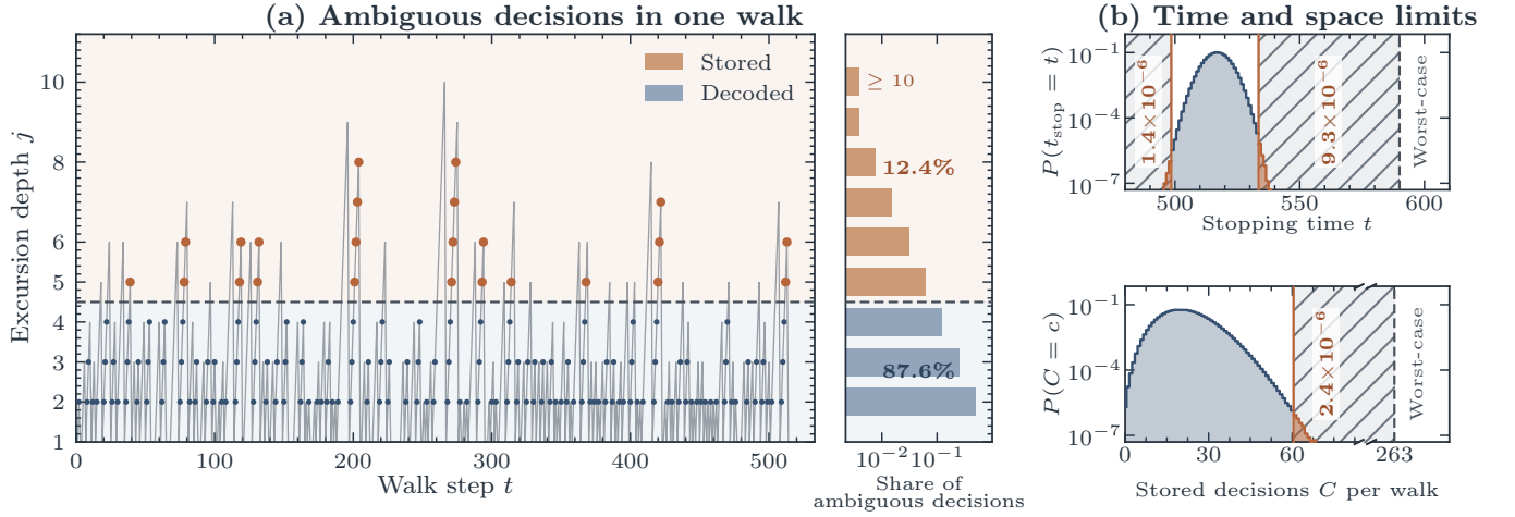
FIG. 3 Making divsteps reversible with minimal overhead. (a) Excursion depth j in one representative walk. Dots mark ambiguous decisions. We use a cutoff j_{\text{store}} = 5 , so all ambiguous decisions with j \geq 5 are stored rather than decoded. The histogram shows the distribution of excursion depths over uniformly sampled walks: only 12.4% of ambiguous decisions reach j \geq 5 . (b) Empirical stopping-time and history-size distributions. The discovered circuit assumes that every walk terminates between steps 499 and 533; this assumption fails with probability \sim 10^{-5} . It also allocates enough qubits to store at most 60 branch decisions, which is sufficient for all but a 2.4 \times 10^{-6} fraction of walks.
