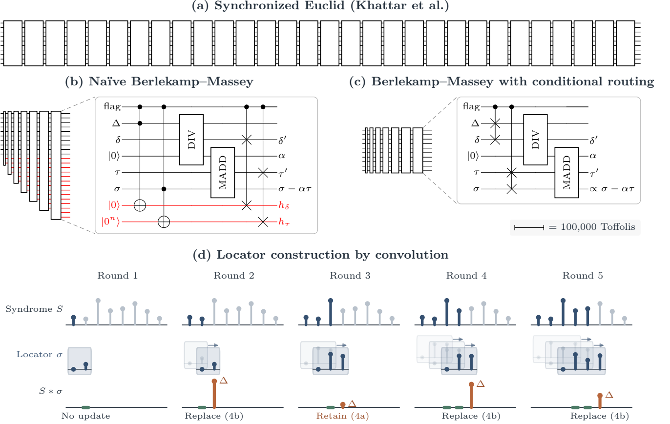
FIG. 2 Reversible Reed–Solomon decoding. (a) The synchronized extended-Euclidean construction of Khattar et al. [13] requires approximately 1.9 million Toffolis for the locator solve. (b) Berlekamp–Massey reduces this cost to approximately 140,000 Toffolis but naïvely accumulates intermediate information (red). DIV forms \alpha = \Delta/\delta , MADD applies the multiply-add, and the flag marks the replace case. (c) Conditional routing preserves this arithmetic advantage while avoiding most history storage. Block widths are proportional to Toffoli count. (d) Locator construction as convolution with the syndrome sequence. The discrepancy \Delta is the convolution at the next syndrome; a nonzero value requires updating the locator.
