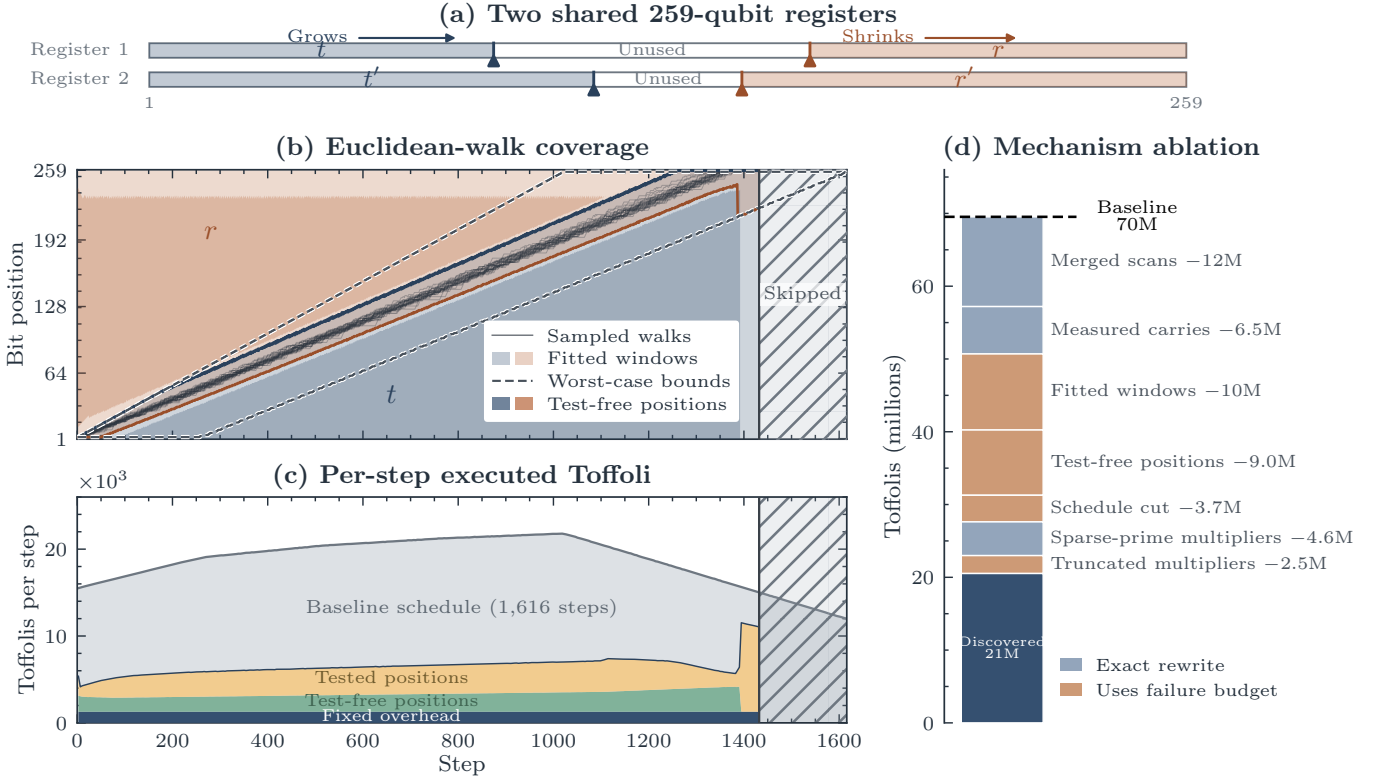
FIG. S2 Specializing the Euclidean schedule and its contribution to the Toffoli reduction. (a) Two 259-qubit registers store coefficients t, t' from their low ends and remainders r, r' from their high ends. Four counters mark the boundaries of these values as the coefficients grow and the remainders shrink. (b) Each thin curve traces the moving boundary between the shrinking remainder r and growing coefficient t for one sampled walk. Light shading shows the fitted windows retained by the discovered circuit, dashed curves show the exact worst-case bounds, and dark shading marks the test-free positions, processed without first testing the counters. The hatched region is removed by the schedule cut from 1,616 to 1,432 steps. (c) Executed Toffolis per step. The gray profile is the baseline schedule; the discovered circuit's profile splits into the fixed overhead of a step, arithmetic at test-free positions, and arithmetic at tested positions. (d) Cumulative ablation from 70 million to 21 million Toffolis. Blue changes are exact, whereas brown changes count against the failure budget.
