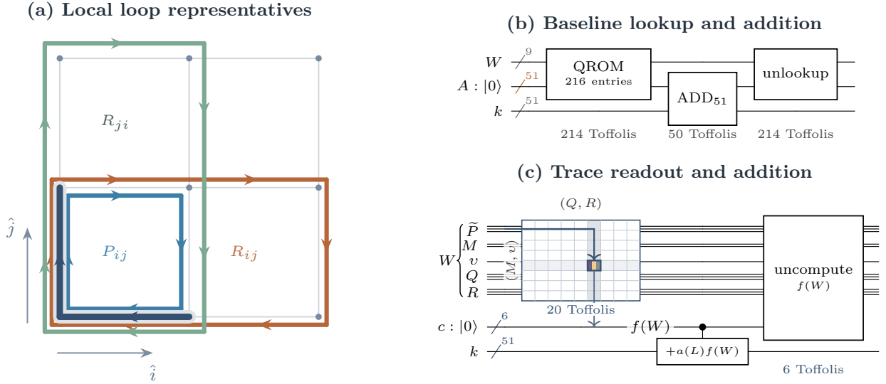
FIG. S5 Loop geometry and trace accumulation in the nonabelian lattice-gauge circuit. (a) The blue, orange, and green paths are cyclic or inverted representatives of P_{ij} , R_{ij} , and R_{ji} whose trace values equal those of Equation (76) by Equation (86); the dark segment is shared after these symmetry choices. (b) The baseline lookup, modular addition, and unlookup for a completed loop product. (c) The trace readout, drawn as a truth table over the coordinates (\tilde{P}, M, v, Q, R) of the specialized representation, followed by the controlled addition. Rows encode (M, v) , columns encode (Q, R) , and the highlighted cell and stripes show how (M, v, Q, R) and then \tilde{P} determine the trace value.
