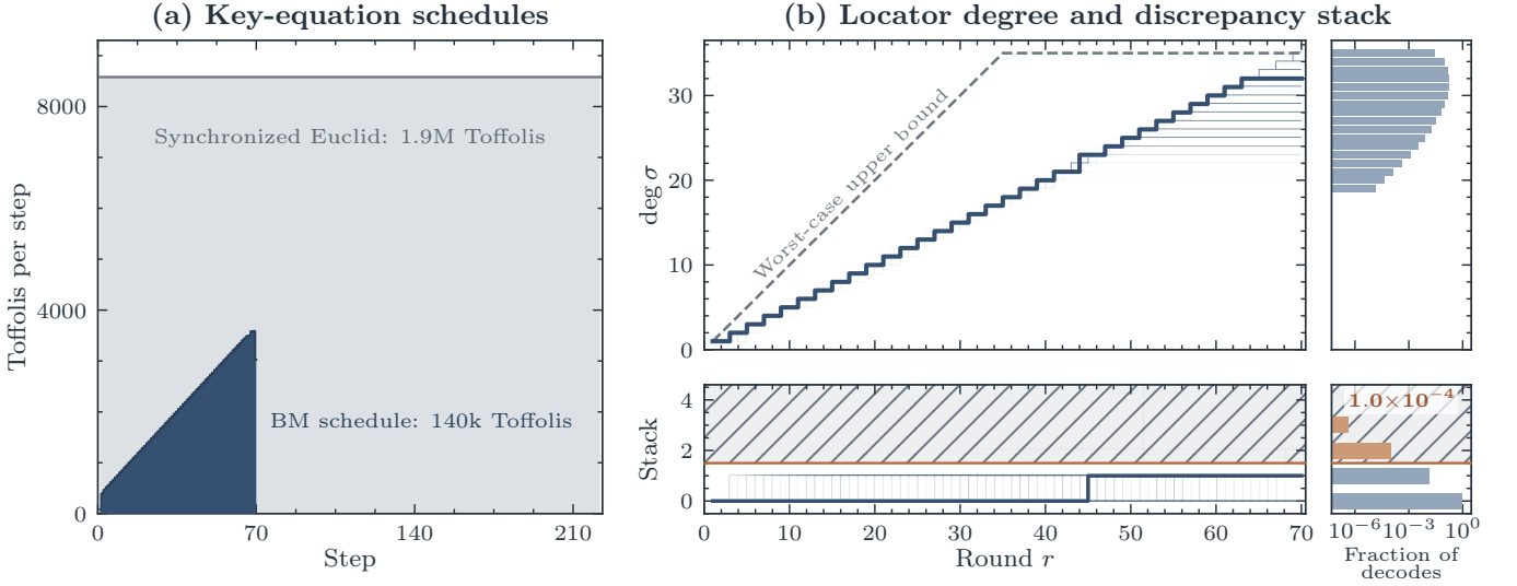
FIG. S1 The Reed–Solomon decoder. (a) Measured forward Toffoli cost per step: one cycle of the 222-cycle synchronized EEA baseline of Khattar et al. [13], or one round of our 70-round BM decoder. (b) Locator degree (top) and number of stored discrepancies (bottom) by round, across 20,000 samples drawn from the DQI input distribution, with one sample highlighted; the dashed line is the worst-case degree bound \min(r, 35) . The right-hand panels show the final locator-degree distribution and the distribution of maximum discrepancy-stack depth. Inputs in the hatched region need more than the one allocated stack entry and may produce a wrong sign; this occurs with probability 1.0 \times 10^{-4} .
