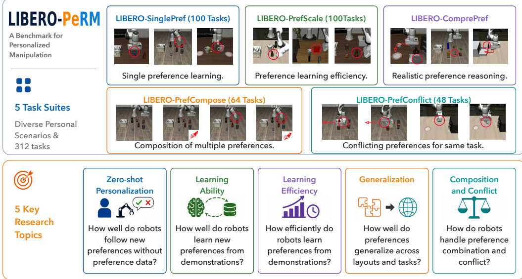
Figure 1: Top: LIBERO-PeRM contains five procedurally generated task suites with pipeline-generated, human-reviewed demonstrations. Bottom: we investigate five key research questions in personalized manipulation.
