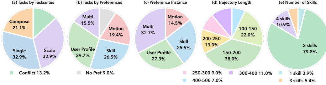
Figure 2: LIBERO-PeRM dataset statistics. (a) Distribution of tasks by task suite. (b) Distribution of tasks by preference type; No Preference denotes generated tasks from LIBERO-PeRM. (c) Distribution of preference instances by preference type. (d) Trajectory length distribution. (e) Distribution of skill numbers in a task.
