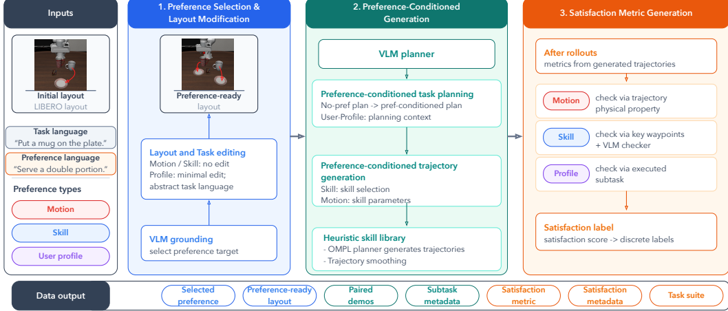
Figure 3: Data generation pipeline for personalized manipulation. Building on the LIBERO framework, the pipeline first generates preference-conditioned data, including preferences, conditions, subtasks, and trajectories, and then derives preference metrics and metadata.
