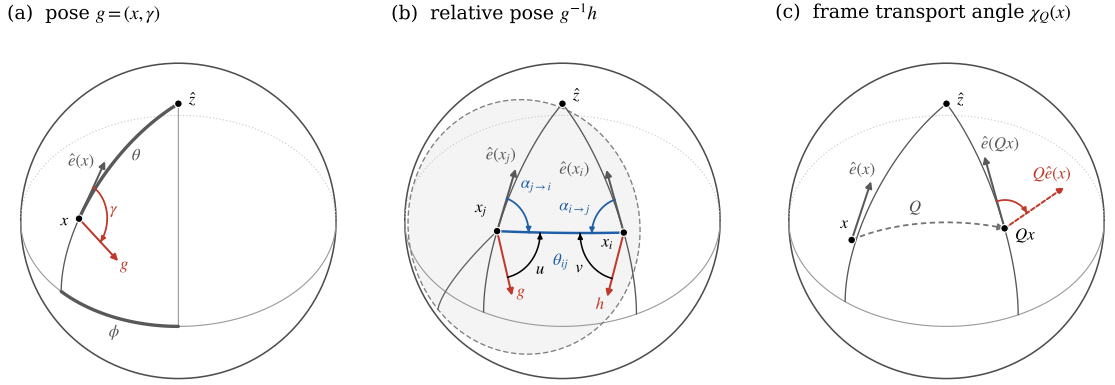
Figure 2: Coordinates of the SO(3) convolution: a pose, the relative pose of two points, and the transport angle.
