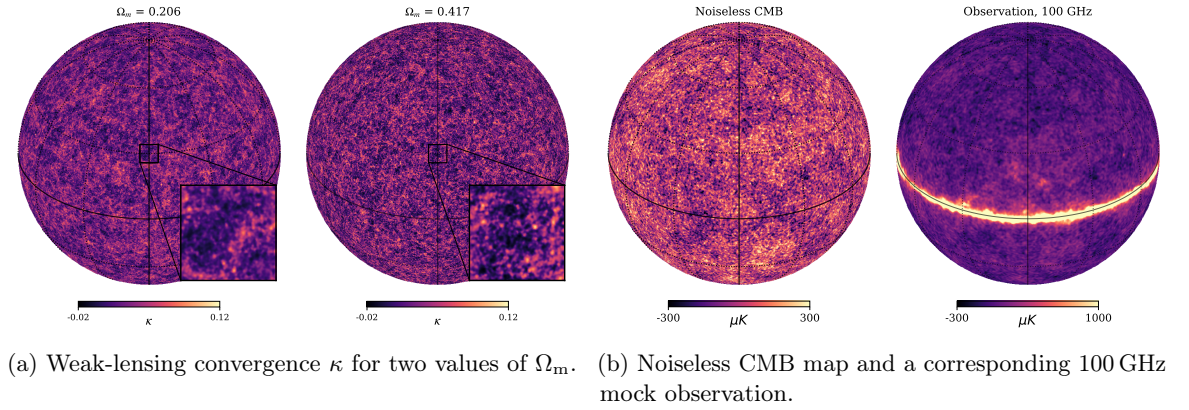
Figure 1: Spherical data from cosmology for the benchmark tasks.
