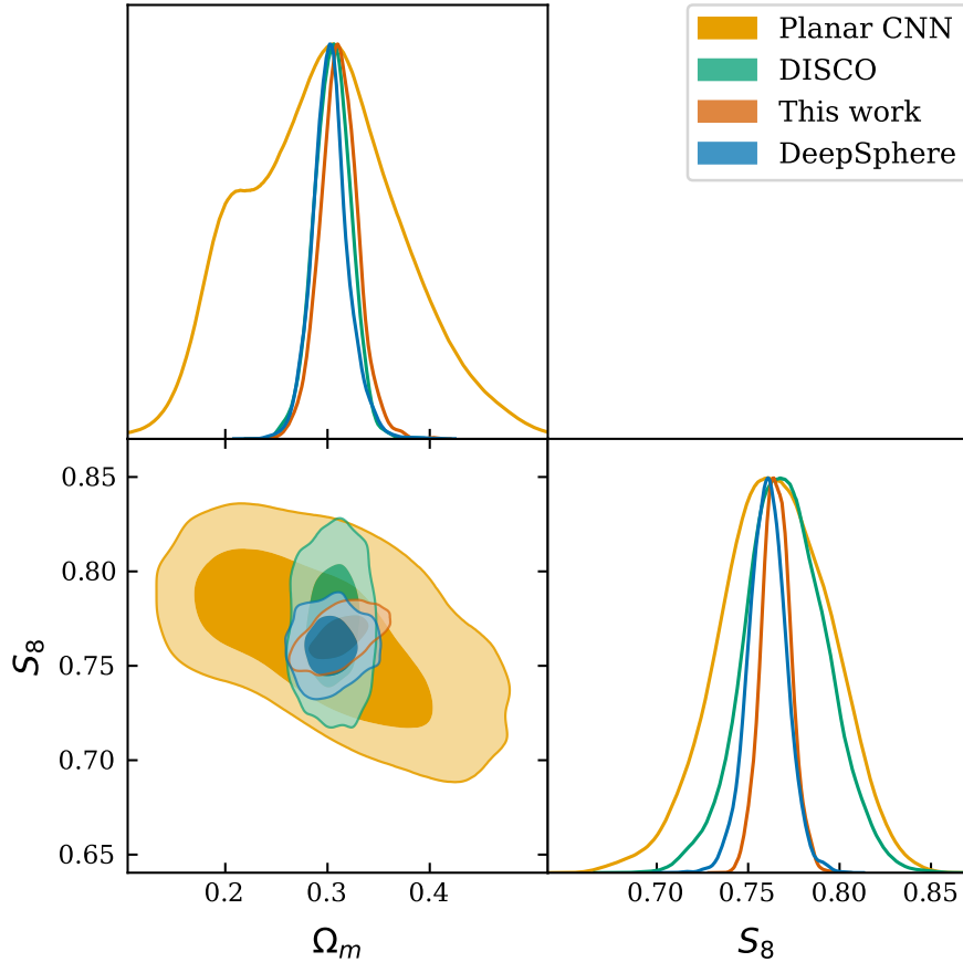
Figure 3: Cosmological parameter \Omega_m – S_8 posteriors from simulation-based inference with lensing data, comparing a CNN from this work with a planar CNN, DISCO and DeepSphere compressors (i.e. embeddings) using the same number of expensive training simulations. The poor results from models not optimised for spherical data (especially the Planar CNN) given a fixed simulation budget forces a user to rely on imperfect simulators to increase the simulation count – our method avoids this by including a spherical symmetry as inductive bias.
