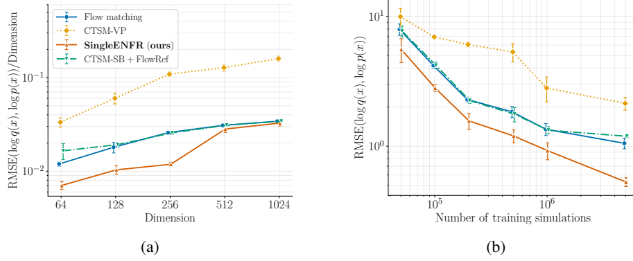
Figure 2: Scaling of density-estimation accuracy with (a) data dimensionality and (b) number of training simulations on the Gaussian mixture model of Appendix A.1, for which the true density is known analytically. We report the RMSE between estimated and true log-density over 200 held-out test points. In (a) the simulation budget is fixed at 5 \times 10^6 ; in (b) the dimensionality is fixed at 64. The line shows the mean across three trained models and the errorbars show the estimated standard deviation. SingleENFR (orange) improves on the flow it is built on (blue) at every point and is the most accurate of all estimators considered, while CTSM-VP (yellow) is consistently the least accurate.
