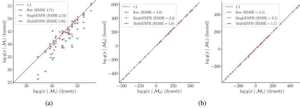
Figure 3: (a) Evidence estimation for noisy observations of an ODE driven time series using flow matching and our ENFR models. MultiENFR outperforms the other models. (b) Diffusion drift application of standard flow matching and our ENFR networks. MultiENFR shows the best performance and good evidence estimation over a large dynamical range.
