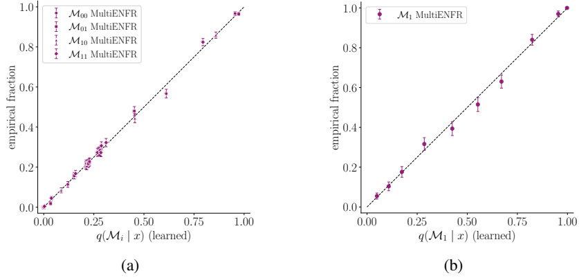
Figure 4: Blind coverage testing for the simulation-based applications for (a) the Hodgkin-Huxley application, and (b) the Galaxy assembly bias application. As we do not have access to a likelihood-based evidence estimate for our simulation based models we test whether the resulting Bayes factors are well calibrated. We find that our MultiENFR architecture is well calibrated in both cases. The error bars show 2\sigma binomial errors.
