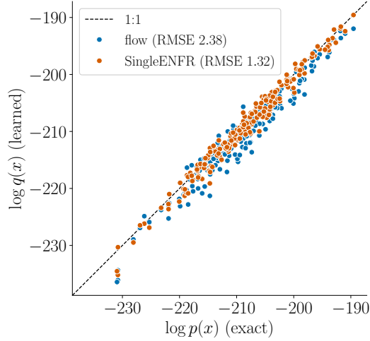
Figure 6: The performance on test points in 128 dimensions for the flow and SingleENFR.
