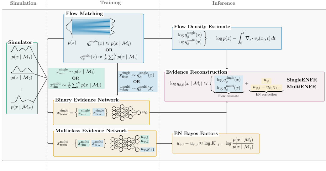
Figure 1: A visualization of our proposed SingleENFR and MultiENFR architectures. Given simulated data from one or multiple models, we train flow matching once over all models. In a second step, we use the simulated data and samples from the flow to train an evidence network classifier, which learns all Bayes factors. Those can be combined with the evaluated flow density to obtain the evidence under a given model.
