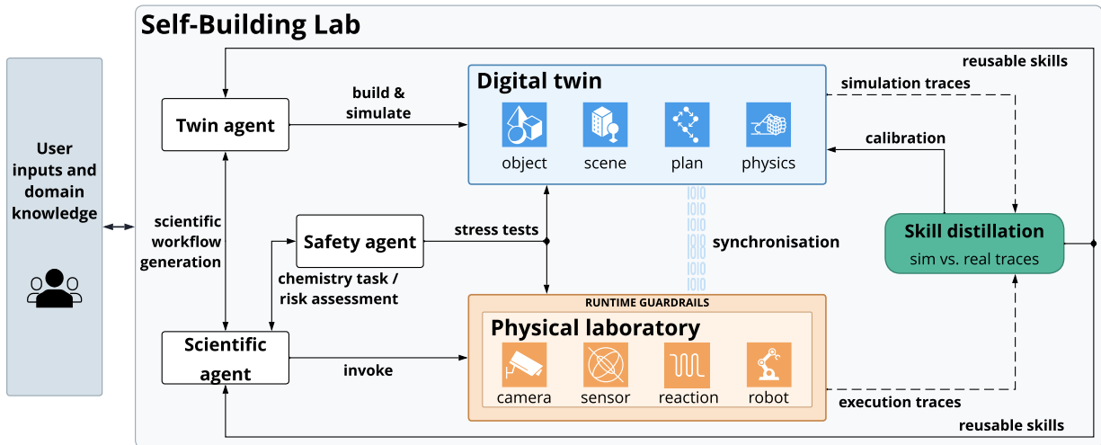
Figure 2 Architecture of the self-building laboratory. The scientific agent translates user goals into experimental plans, while the twin agent constructs a digital twin , develops task-relevant skills, and validates workflows in simulation. The safety agent uses the twin for scenario analysis and generates runtime guardrails through which all physical laboratory commands pass. The scientific agent invokes the physical laboratory through this layer. Physical state feedback supports twin calibration and subsequent simulation, while simulation and physical execution traces support skill distillation and the retention of experience as agent memory. Reusable skills and memories inform subsequent tasks.
