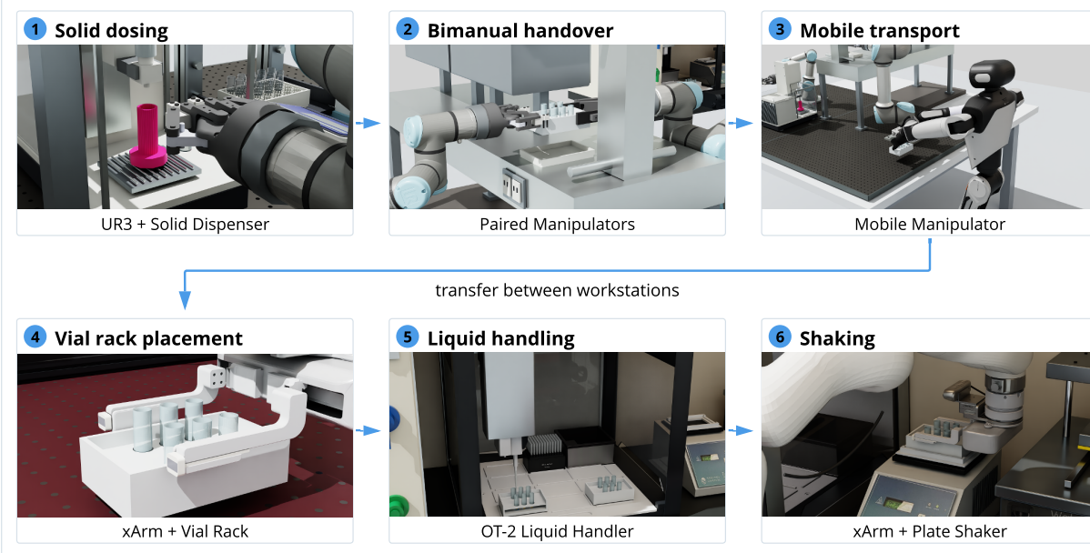
Figure 6 Scaling self-building laboratories across robots and workstations. The reconstructed simulation layout (top) integrates a UR3/UR5 solid-handling workstation, a mobile manipulator, and an xArm-based liquid-handling workstation. Given a high-level buffer-preparation goal, SBL generates a coordinated workflow (bottom) in simulation, and also generates task-relevant powder and fluid simulation models for solid and liquid handling.
