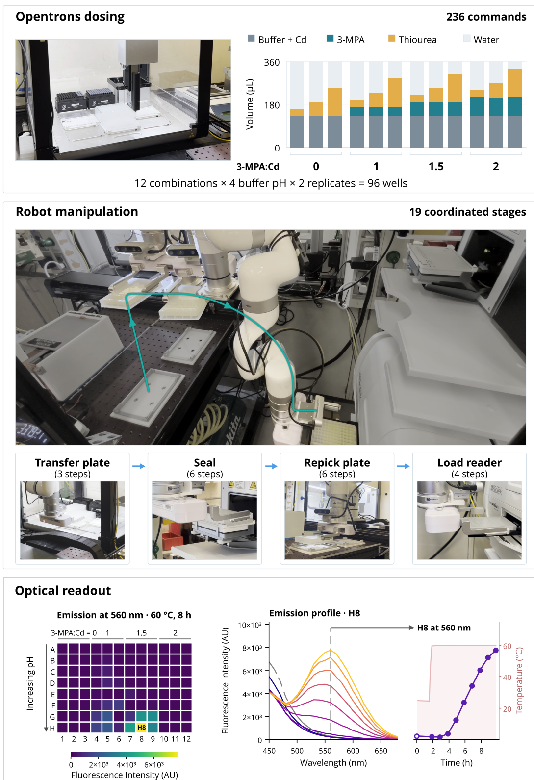
Figure 5 SBL-coordinated CdS synthesis and optical readout. SBL executed 236 OT-2 commands to prepare a 96-well plate, followed by 19 robotic stages for transfer, sealing, re-grasping, and reader loading. Overlaid video frames and teal arrows illustrate plate handling. The heatmap shows fluorescence intensity at 560 nm after 8 h, with well H8 highlighted. The adjacent plots show the evolution of the H8 emission spectrum and its fluorescence intensity at 560 nm alongside the temperature trace.
