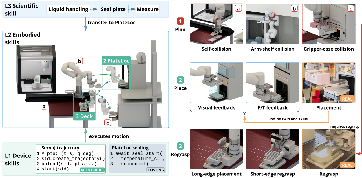
Figure 4 Scientific tasks drive laboratory skill development. A plate-sealing task drives the development and integration of embodied and device skills. Digital-twin planning and feedback from physical execution guide refinement of the twin and skills, connecting scientific requirements to executable laboratory capabilities.
