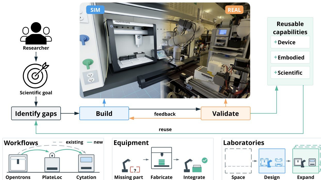
Figure 1 Concept of a self-building laboratory (SBL). Scientific goals guide the identification of capability gaps, development in a digital twin, and validation in the physical laboratory. Feedback and reuse support continued capability development across workflows, equipment, and entire laboratories. The image combines SDL2 at the Acceleration Consortium, University of Toronto, Canada, with its digital twin built by the SBL and rendered in Isaac Sim in a blue wireframe style.
