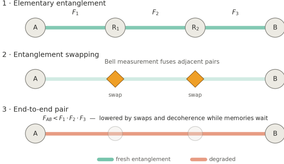
Fig. 1. Entanglement distribution along a repeater path. Elementary links are generated probabilistically and then fused by Bell-state measurements at intermediate repeaters. The final end-to-end fidelity is affected not only by the elementary-link qualities, but also by swap imperfections and memory decoherence accumulated while neighboring links wait.
