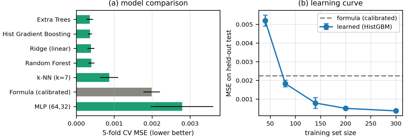
Fig. 3. Learning the expected fidelity. a) Five-fold cross-validated error of six regressors against the per-fold-calibrated formula; tree ensembles cut the error \sim 5\text{--}6\times . b) Learning curve: the surrogate overtakes the formula after \sim 80 configurations and keeps improving.
