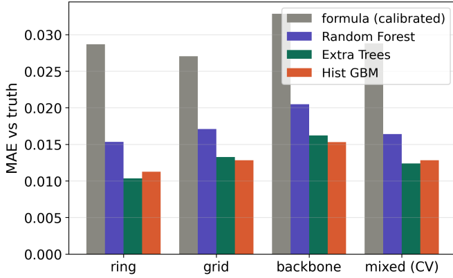
Fig. 4. Generalization to unseen path regimes. Leave-one-family-out error over 270 paths (90 per family; train on two of ring/grid/backbone, test on the third) beside pooled-interpolation error; every model beats the formula on each unseen family, and extrapolation is close to interpolation.
