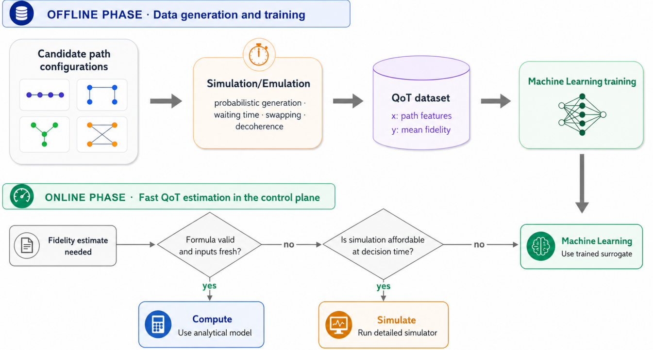
Fig. 2. Decision-aware machine-learning workflow for quantum QoT estimation. The upper part shows the offline training workflow: candidate path configurations are evaluated with a quantum-network simulator to produce fidelity labels, build a QoT dataset, and train a machine-learning surrogate. The lower part shows the online decision flow: a fidelity-estimation request is mapped to analytical computation when the formula is valid and its inputs are fresh, detailed simulation when runtime allows, or the trained machine-learning surrogate when repeated simulation is too costly at decision time.
