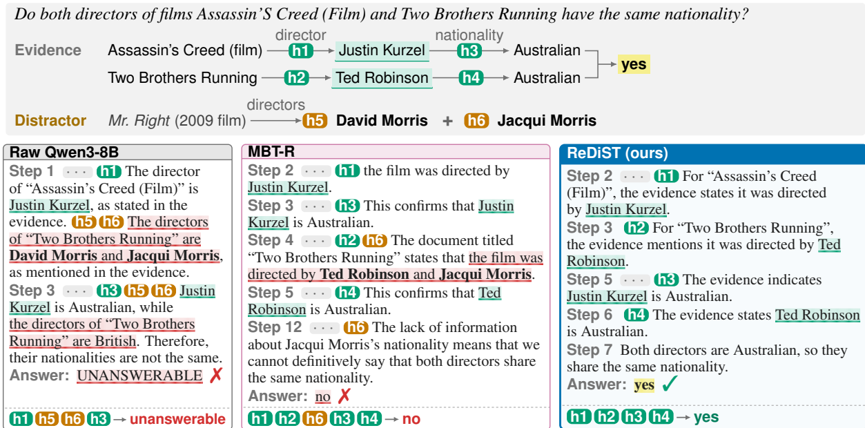
Figure 3 Evidence use in a selected 2Wiki example. Test-time reasoning excerpts from raw Qwen3-8B and Qwen3-8B students trained with MBT-R or REDiST. MBT-R identifies the relevant directors but introduces an unsupported co-director. In contrast, the REDiST output uses the relevant film–director–nationality links and answers correctly. Quoted model text is reproduced verbatim, with ellipses marking omissions, while highlights, correctness markers, and notes are author annotations.
