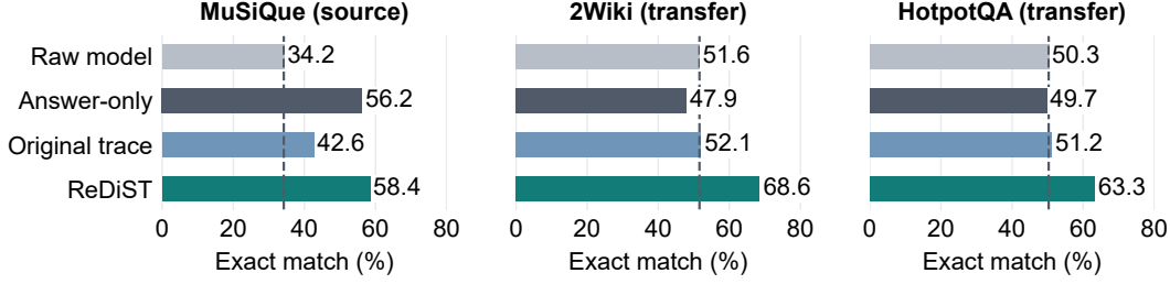
Figure 1 Source-task accuracy and cross-benchmark transfer respond differently to supervision. Qwen3-8B before task-specific training (Raw) and after training on MuSiQue with answer-only supervision, original student traces, or ReDiST. MuSiQue measures source-task performance, while 2Wiki and HotpotQA measure cross-benchmark performance. Dashed lines mark each benchmark’s raw-model EM. Values are EM point estimates from Table 1. Comparisons between trained variants reflect complete training recipes.
