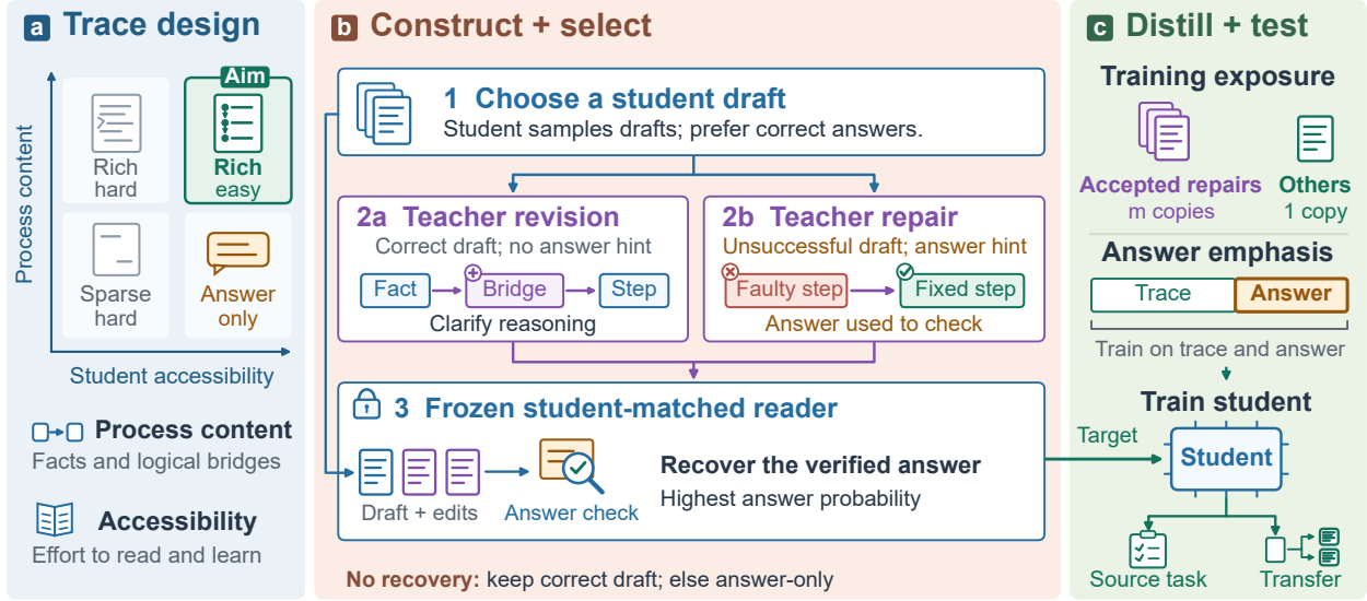
Figure 2 ReDiST: student-conditioned trace construction and distillation. (a) Process content and student accessibility guide the design. (b) A rewrite model revises answer-correct student drafts against the supplied evidence and repairs unsuccessful drafts with additional guidance from the verified answer. A frozen student-matched reader screens and ranks original and edited candidates using answer recovery and verified-answer probability, given the question, evidence, and candidate trace. (c) Repair exposure m and auxiliary answer-loss weight \alpha control how selected targets enter training. Teaching utility is evaluated through the trained student’s source-task and cross-benchmark performance.
