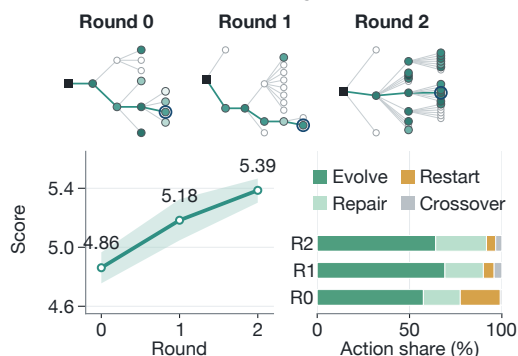
(b) RSI shifts evolutionary behavior
