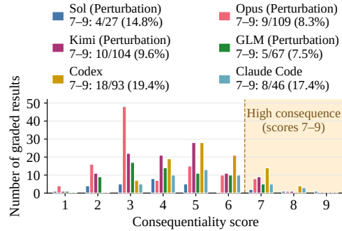
Figure 3: GPT-5.6 Sol consequence scores for analyses of published papers; shading marks scores 7–9.
