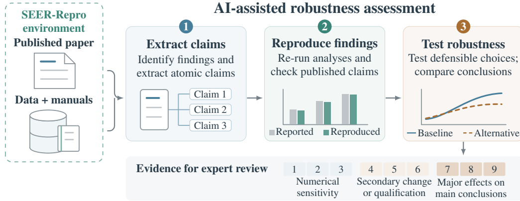
Figure 1: AI-assisted robustness assessment pipeline to support expert review.
