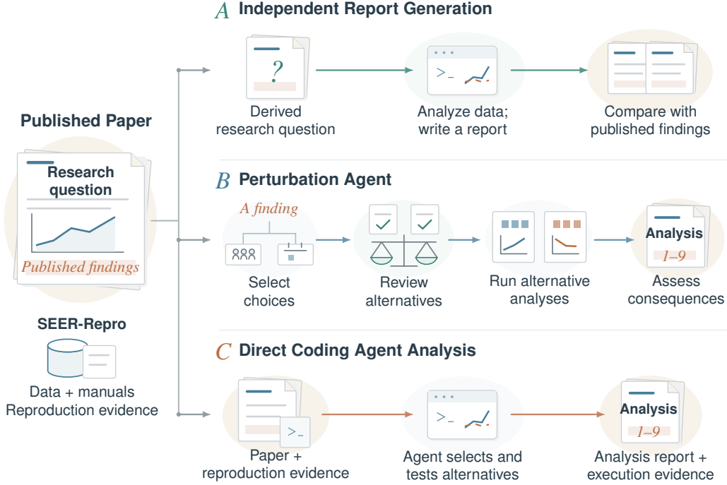
Figure 2: AI-driven analytical robustness with 3 complementary methods discussed in Sec 3.2
