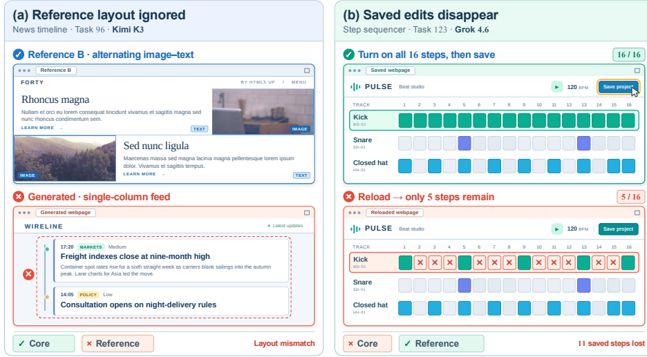
Figure 4: Two failure cases identified by RefCraft: one in reference following and the other in core functionality.
