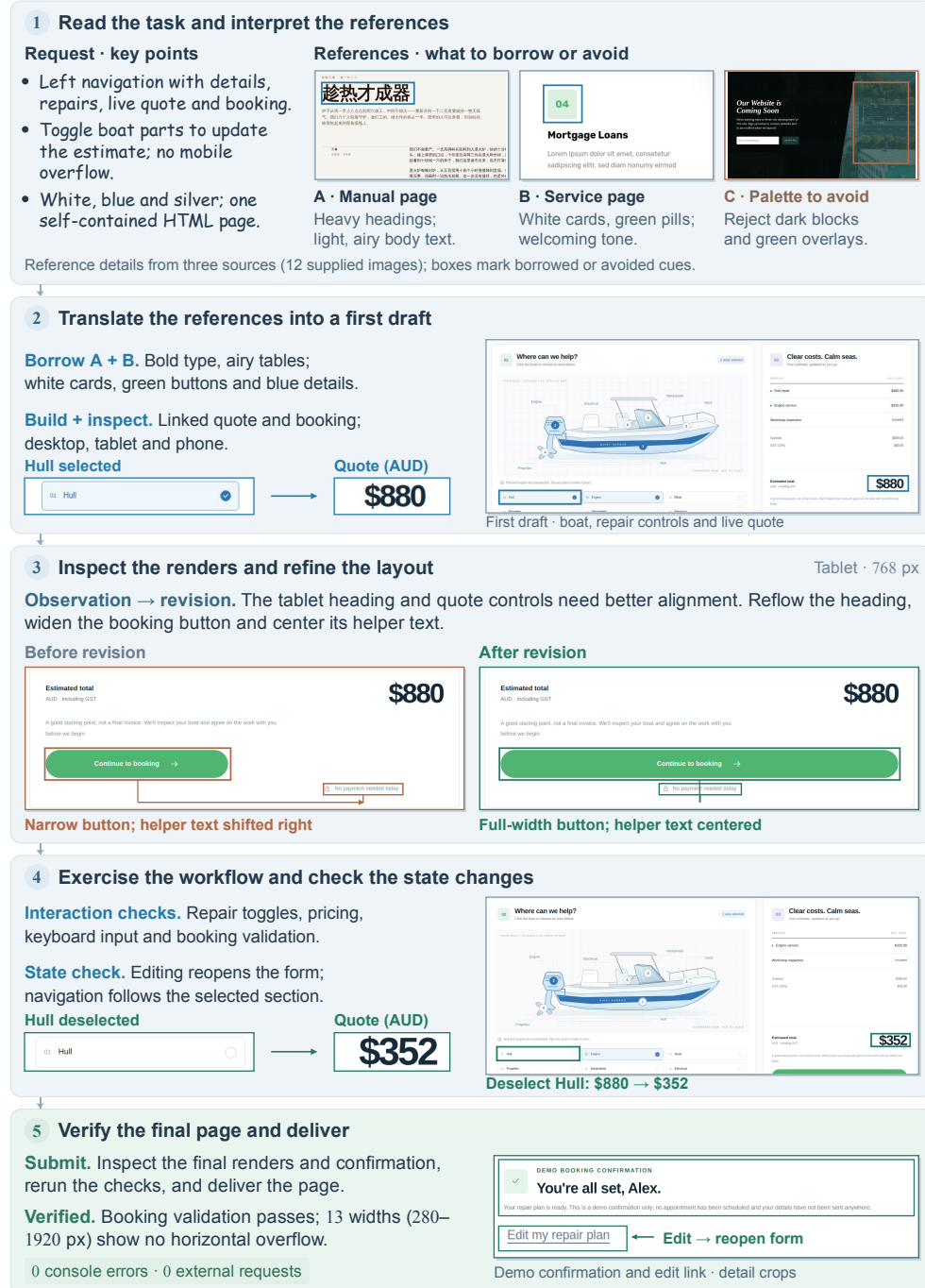
Figure 9: An end-to-end development trajectory on Task 163. Boxes and enlarged screenshot crops highlight reference cues, responsive-layout revisions, and changes in the quote and booking state.
