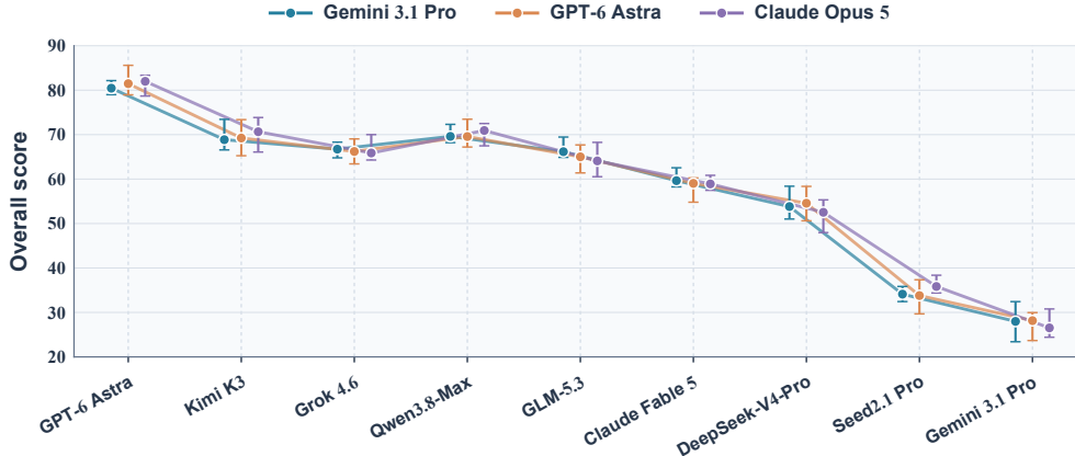
Figure 6: Judge sensitivity on the fixed 32-task sample. Colored points and connecting lines show scores assigned by Gemini 3.1 Pro, GPT-6 Astra, and Claude Opus 5. Whiskers indicate illustrative uncertainty intervals. Relative scoring patterns are broadly consistent across the three models.
