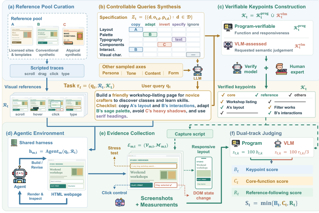
Figure 2: Construction and evaluation of RefCraft. (a) Reference webpages are captured across interaction states. (b) A specification spanning six visual dimensions and five requirement types guides natural-language query synthesis. (c) Task requirements are decomposed into program-verifiable and VLM-assessed keypoints. (d) Given the query and reference images, agents iteratively build, render, inspect, and revise a webpage in a shared harness. (e) Keypoints guide evidence collection from generated artifacts. (f) Complementary programmatic and VLM judges produce the base keypoint score B , core-function score C , and reference-following score R .
