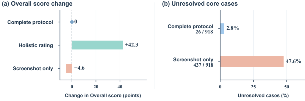
Figure 7: Protocol sensitivity and evidence coverage. (a) Changes in Overall score relative to the complete protocol: +42.3 under holistic rating and -4.6 under screenshot-only evaluation. (b) Observed rates of unresolved core cases across matched artifacts.
