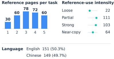
Figure 5: Composition and diversity of RefCraft.
