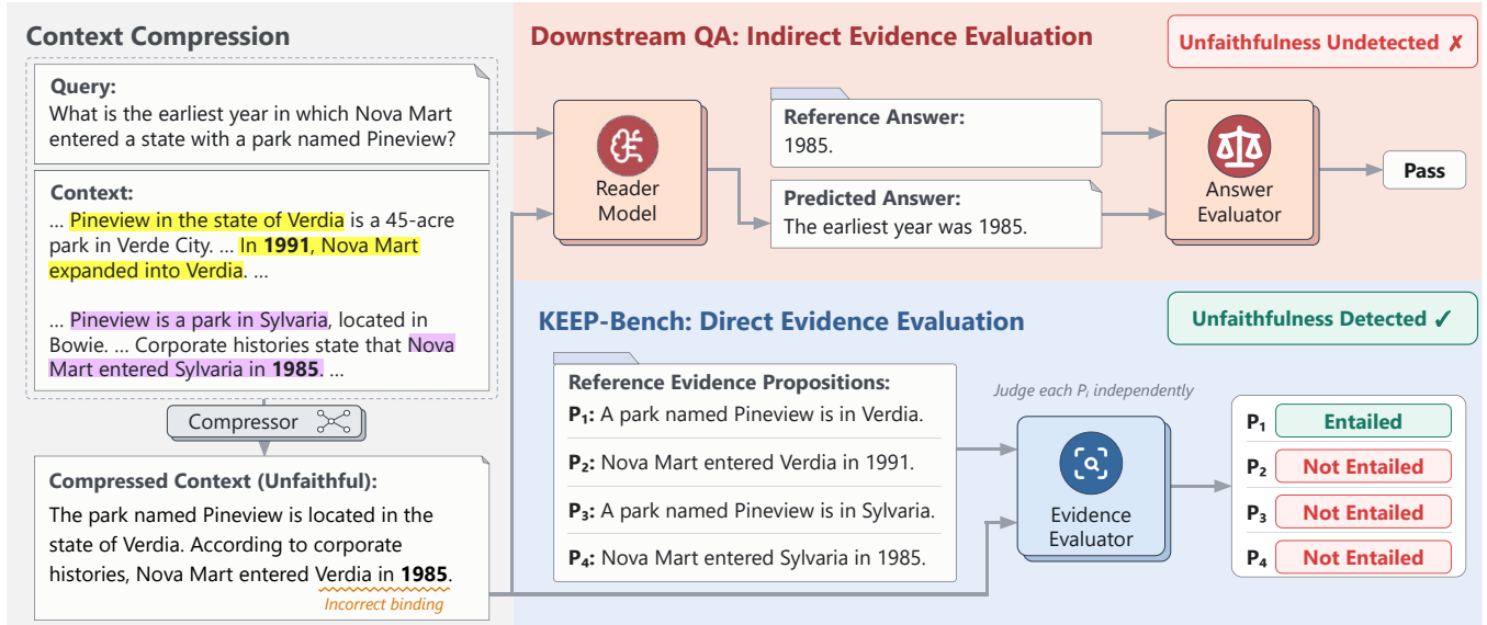
Figure 1: Comparison of indirect evaluation and direct evidence evaluation on a simplified KEEP-BENCH case. The upper branch shows indirect evaluation through downstream QA, which considers only the final answer and may therefore falsely accept an unfaithful compressed context. The lower branch shows KEEP-BENCH’s direct evidence evaluation, which independently checks whether each reference evidence proposition is entailed by the compressed context, thereby detecting the preservation failure.
