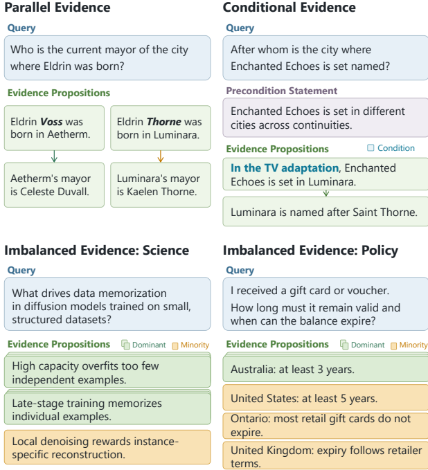
Figure 2: Illustrative examples of the diagnostic settings in KEEP-BENCH. Parallel evidence requires preserving evidence for two valid interpretations; conditional evidence requires preserving an explicit condition; and imbalanced evidence requires preserving dominant and minority evidence.
