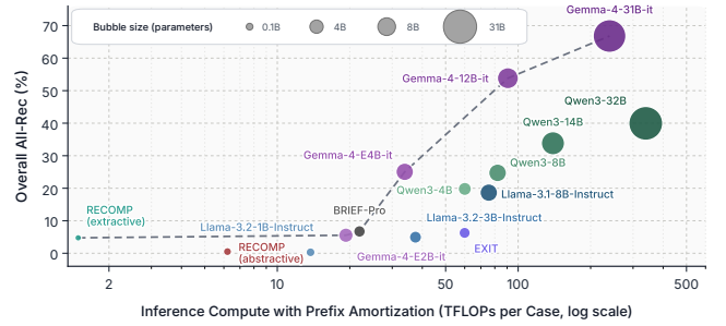
Figure 3: Computation cost and evidence preservation under the default compression budget. Overall All-Rec versus average TFLOPs per case on a log scale. Circle area represents model size; the dashed line marks the Pareto frontier.
