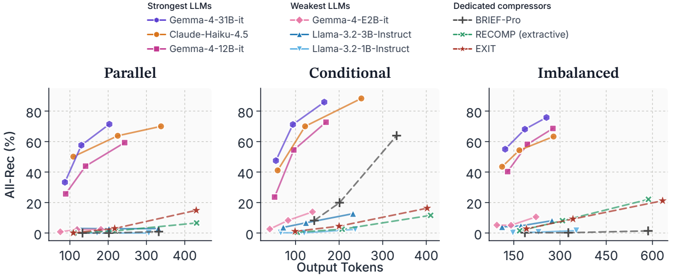
Figure 4: All-Rec under different compression budgets across the three evidence settings. Middle points correspond to the default budget in the main results; left and right points use 0.5\times and 2\times its target sentence count, and the x-axis shows the resulting average output tokens. Shown are the three strongest and three weakest general LLMs by All-Rec at the default budget and the three dedicated compressors with explicit length control (dashed lines). Panels share the same y-axis.
