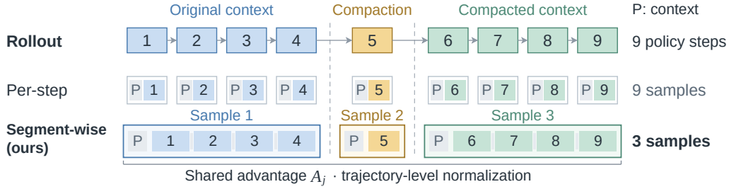
Figure 7: Segment-wise training across compaction. Colors denote maximal prefix-consistent segments, and step 5 performs compaction. Gray blocks indicate masked input context. Segment samples share the trajectory advantage A_j and trajectory-level loss normalization. A 9-step rollout with one compaction event at step 5 yields 9 independent samples under per-step training but only 3 segment samples under our approach.
