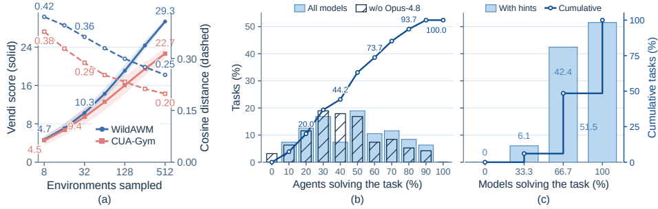
Figure 3: (a) Environment diversity using Qwen3-Embedding-8B (Zhang et al., 2025b) representations of environment artifacts. Shaded bands are 95% intervals of the Vendi score (Friedman & Dieng, 2022). (b) Task solvability across 24 model-harness configurations: the three models and six harnesses in Sec. 3.2 (Rollouts & Judgments), plus Opus-4.8. (c) Solvability with hints w/o Opus-4.8.
