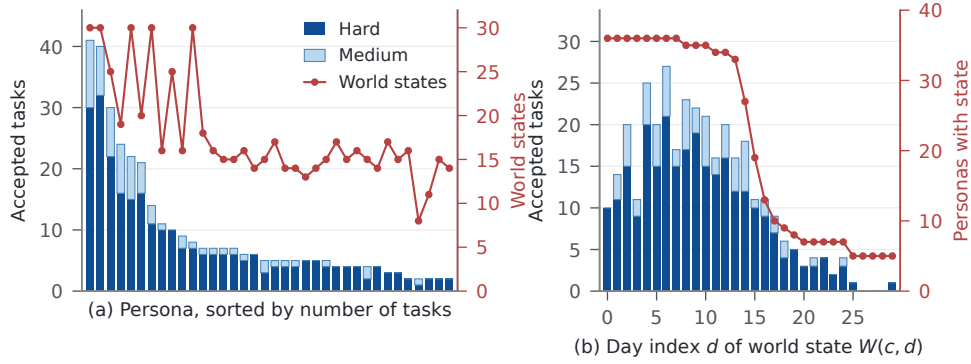
Figure 6: Distribution of the 341 accepted XAI tasks. (a) Tasks per persona, split by difficulty, with the number of world states of each persona. (b) Tasks per day index, with the number of personas that have a world state on that day.
