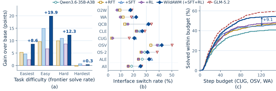
Figure 5: Behavior analysis of base model, WildAWM and its variants (+RFT, +SFT, and +RL, i.e., RL without SFT), and GLM-5.2. (a) Pass-rate gain over the base model on OOD tasks, split into four equal quartiles by how many of frontier models solve each task. (b) Fraction of consecutive tool calls that switch between interface families (e.g., GUI \rightarrow CLI). (c) Tasks solved within a step budget.
