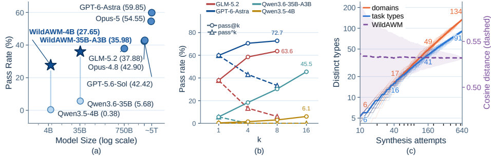
Figure 4: (a)/(b) Performance on WildAWM validation set, and proprietary model sizes are estimated. (c) Rarefaction of the 341 accepted tasks by LLM-classified task types and domains.
