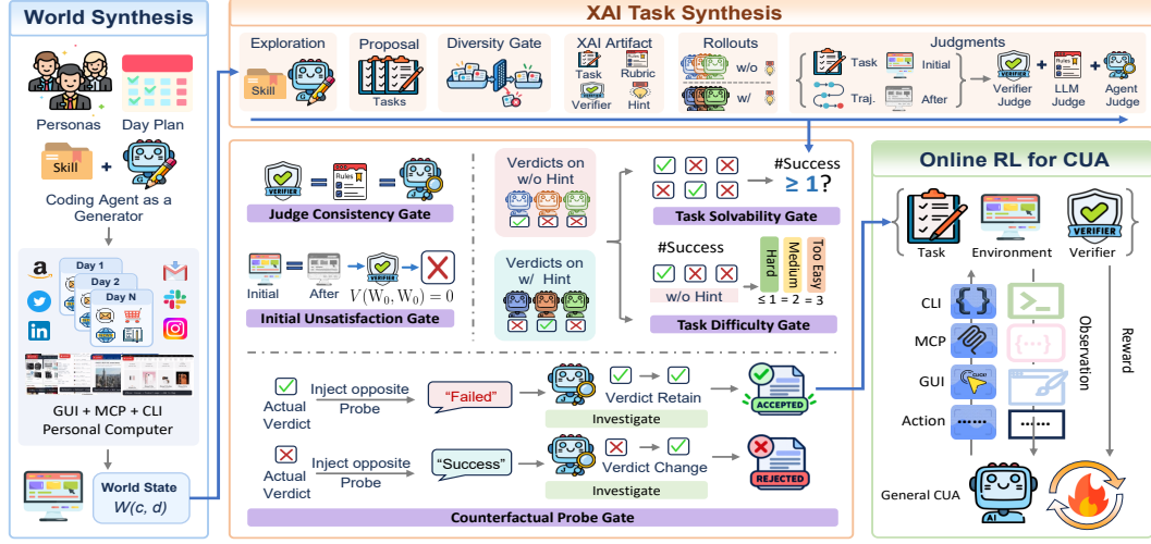
Figure 1: Overview of WildAWM. The synthesis pipeline includes two stages: (1) World Synthesis , where we use the coding agent to construct persona-driven, multi-day world states for computer environments that expose GUI, MCP, and CLI interfaces. (2) XAI Task Synthesis , where we generate cross-interface tasks through 5 designed quality gates for task solvability, difficulty, and verifier reliability. The synthesized \{\text{task}, \text{environment}, \text{verifier}\} triplet enables training general CUA.
