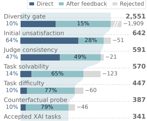
Figure 2: Progression of XAI task candidates. Direct denotes sketches that pass on the first attempt, while After feedback denotes sketches that pass after at least one feedback-driven revision at any stage of the whole synthesis, thus the funnel is monotonic.
