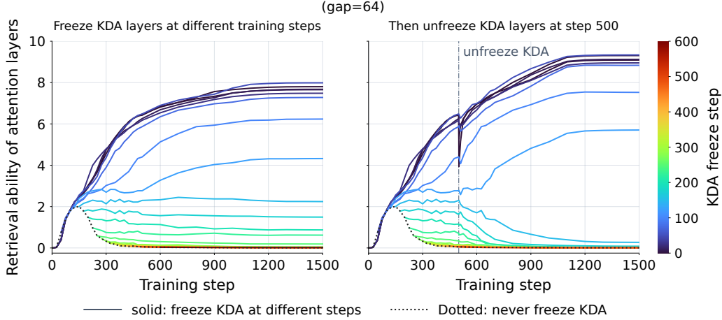
Figure 10: Attention retrieval ability under KDA freezing and unfreezing at g = 64 , using the same setup as in Figure 4.
