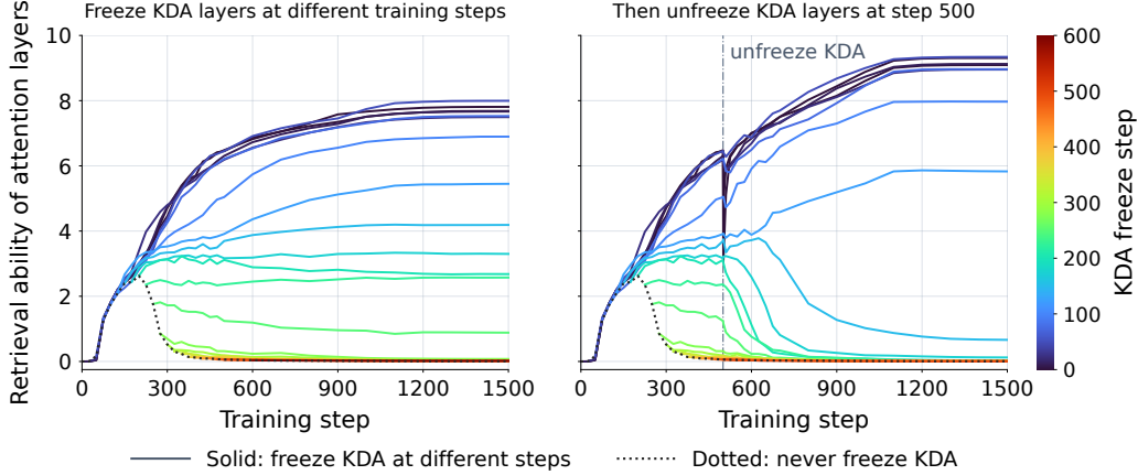
Figure 4: Demonstration of Competing Learning. The curves indicate the retrieval ability of attention layers in a hybrid model consisting of attention and recurrent layers (KDA), trained on our retrieval task, Spaced Retrieval (Section 3.1).
