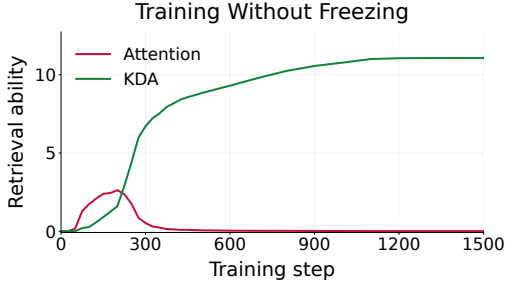
Figure 2: The average retrieval ability of the two types of layer in a hybrid model trained on Spaced Retrieval.
