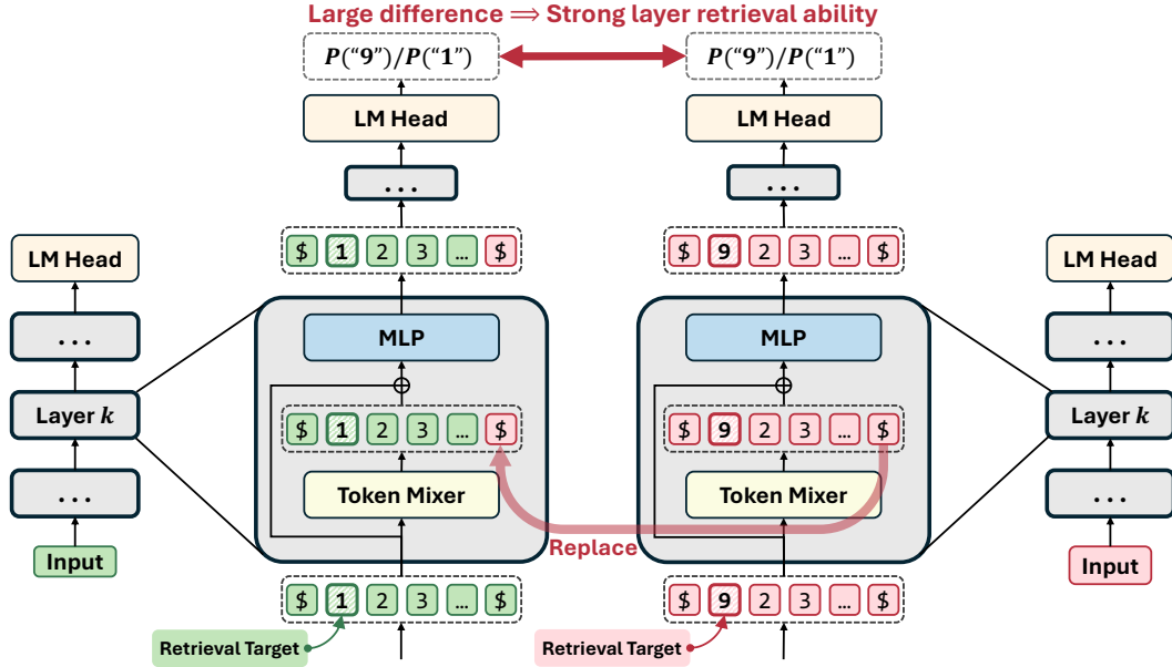
Figure 1: Illustration of our layer retrieval ability estimation method (described in Section 3.2). As an example, the sequence to copy is “123”, and the layer under inspection is layer k . The difference in probability change tells us the contribution of layer k in retrieving the target token “9”.
