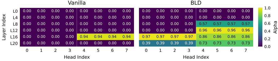
Figure 9: The \alpha values of attention heads. With GQA, query heads 0–3 and 4–7 share a KV head within each group and therefore share the same KV-head-level \alpha value. Greater \alpha values indicate heads that are important for long-distance retrieval.
