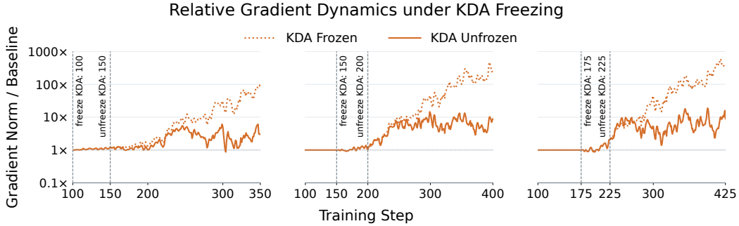
Figure 5: Relative gradient magnitude changes in the Attention layers compared to the baseline without KDA freezing. KDA is frozen at steps 100, 150, or 175, with an unfreezing branch introduced 50 steps later. Across these timings, keeping KDA frozen progressively amplifies attention gradient norms relative to the baseline, whereas unfreezing KDA substantially attenuates this amplification.
