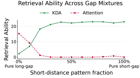
Figure 3: The retrieval ability of the two different kinds of layer in a hybrid model, trained on Spaced Retrieval with different data mixtures.
