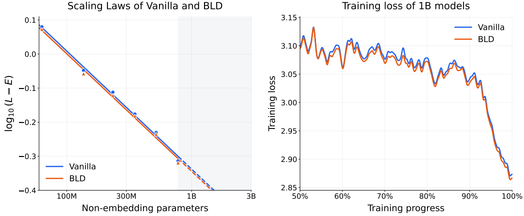
Figure 8: Left: Loss as a function of non-embedding model size, fitted with power-plus-constant scaling laws. Right: The training-loss curve of the 1B vanilla and BLD models.
