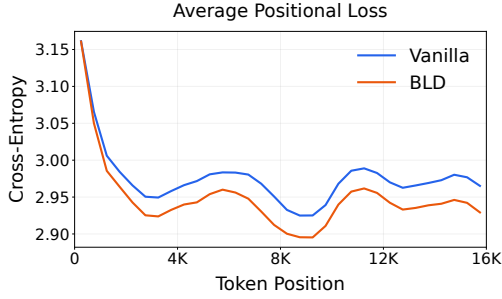
Figure 6: Average position-wise loss of 510M BLD/vanilla model across all examples.
