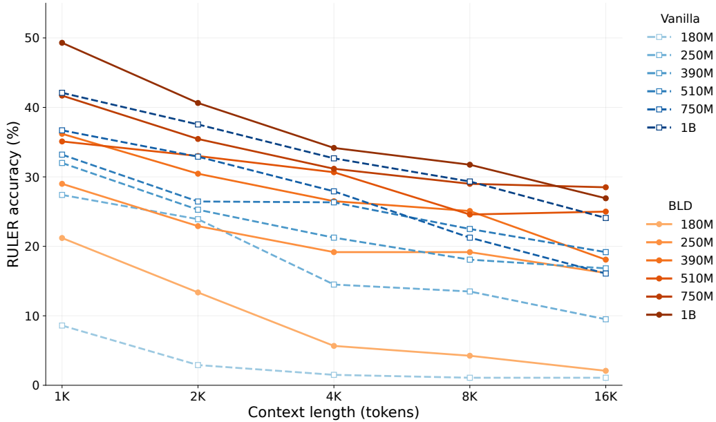
Figure 11: RULER accuracy by context length for six KDA model sizes. Blue dashed lines denote Vanilla; orange solid lines denote BLD. Darker shades indicate larger models. Each point averages the tasks evaluated at that length.
