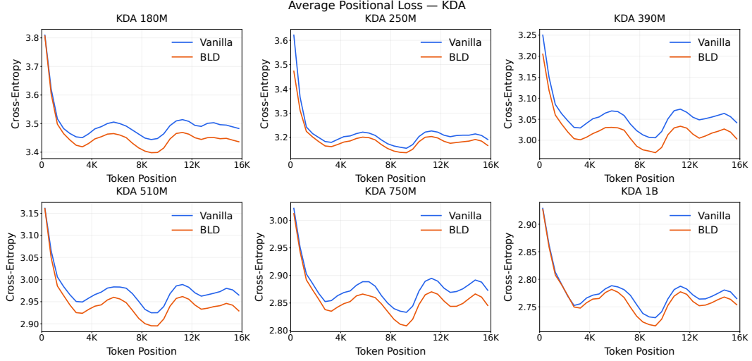
Figure 12: Average loss of KDA hybrid models of different scales, as functions of token positions.
