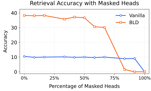
Figure 7: The retrieval accuracy when masking a fraction of the heads.
