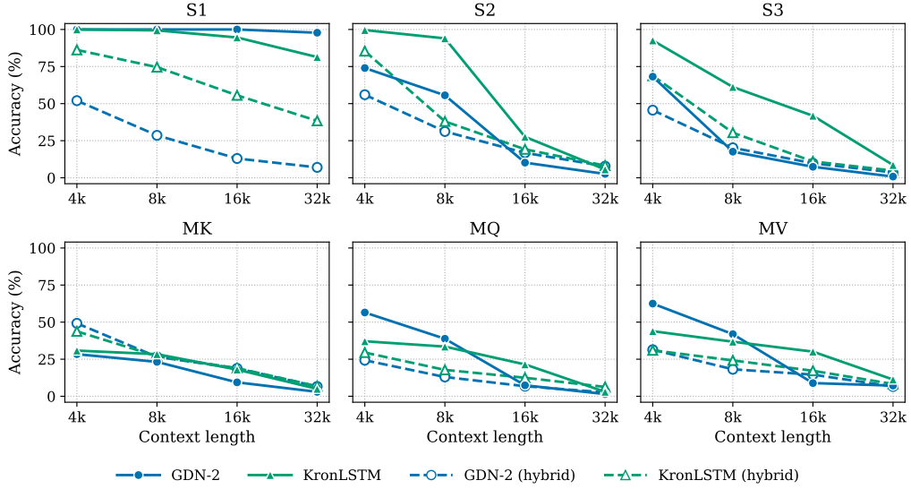
Figure 4: GDN-2 and KronLSTM results on NIAH for 32k context extension for linear and SWA-hybrid models.
