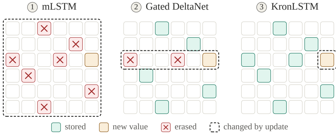
Figure 1: Representation of the memory matrix state revision for mLSTM, Gated DeltaNet, and KronLSTM. Interference with stored values: mLSTM affects all values, Gated DeltaNet affects those with overlapping keys, and KronLSTM affects only those with overlapping key and value pairs.
