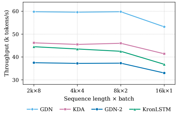
Figure 6: Training throughput of KronLSTM against baselines on a single H100-80GB.
