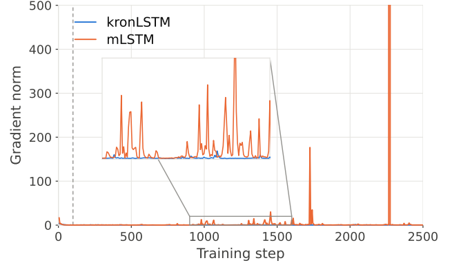
Figure 2: Stress test with high learning rates for the same mLSTM and KronLSTM architectures on language modeling. Learning becomes unstable for mLSTM as the gradient norm spikes show, while KronLSTM yields stable learning.
