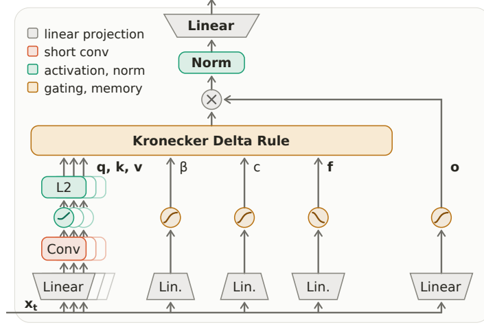
Figure 3: Architecture of the KronLSTM block.
