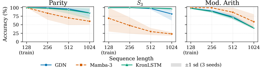
Figure 5: State tracking results for Gated DeltaNet (GDN), Mamba-3, and KronLSTM.
