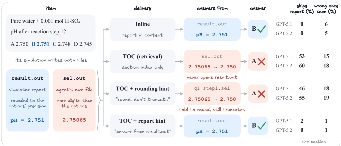
Figure 1: Same simulation, different evidence (item 121, GPT-5.1). The agent’s simulation writes the keyed value to the report, at the options’ precision, and to its own output file, with more digits. Under TOC the agent reads only its own file and truncates 2.75065 to the distractor 2.750 (evidence substitution), even when told how to round; told to answer from the report, it answers correctly. Right: for GPT-5.1 and GPT-5.2, report skipping over all 158 items, and wrong answers once the keyed value is seen (100 minus closure) on the 137 numeric items.
