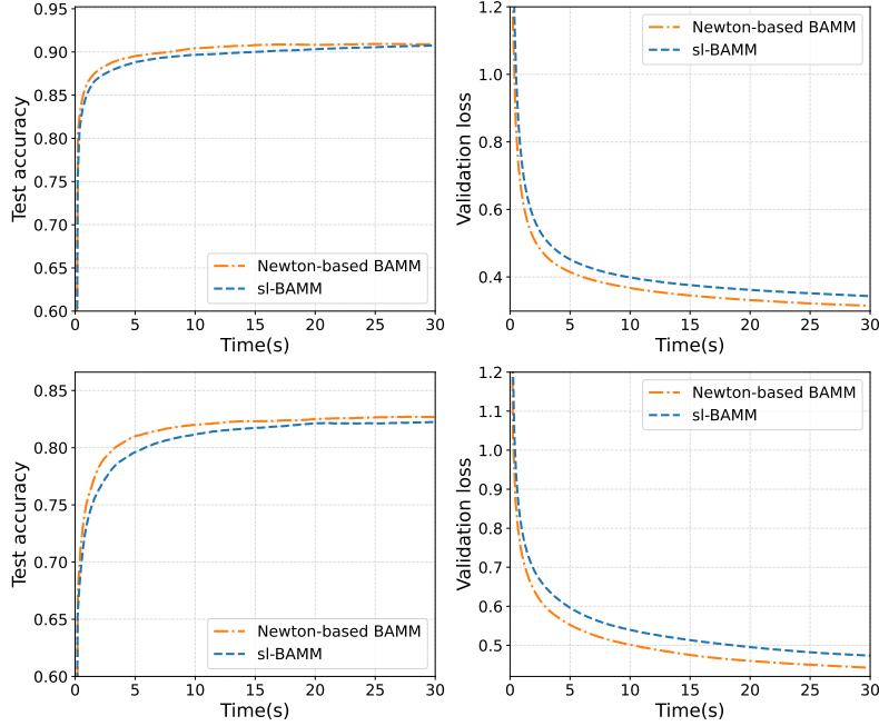
Figure 5: Data hyper-cleaning with linear models. Comparison of sl-BAMB and Newton-based BAMB on MNIST (upper) and FashionMNIST (lower).
