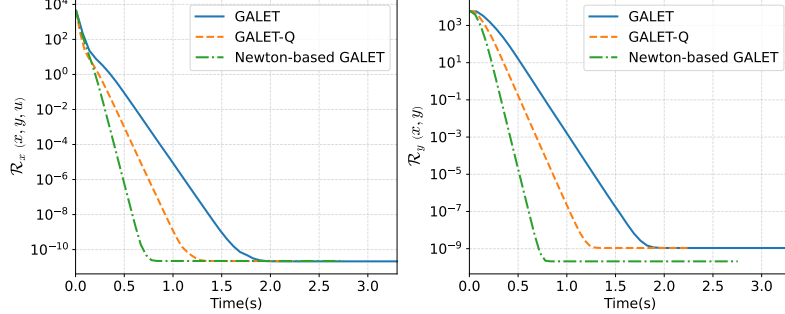
Figure 1: GALET, GALET-Q, and Newton-based GALET on (12) with \zeta = 1 . Left: \mathcal{R}_x . Right: \mathcal{R}_y .
