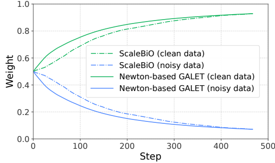
Figure 7: Clean and corrupted data weights for ScaleBiO and Newton-based GALET, averaged over five random seeds.
