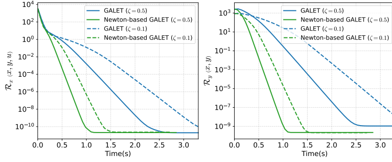
Figure 3: GALET and Newton-based GALET on (12) with \zeta = 0.5, 0.1 . Left: \mathcal{R}_x . Right: \mathcal{R}_y .
