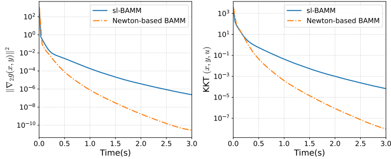
Figure 4: Newton-based BMM and sl-BMM on (13), with stepsizes chosen according to Case 1 of Theorem 3.2.
