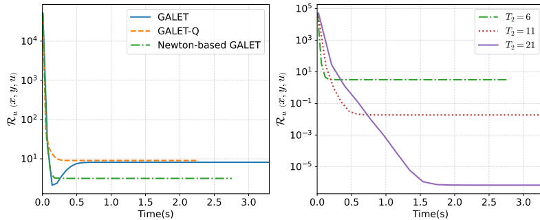
Figure 2: Results on (12) with \zeta = 1 . Left: \mathcal{R}_u for GALET, GALET-Q, and Newton-based GALET. Right: \mathcal{R}_u for Newton-based GALET with T_2 = 6, 11, 21 .
