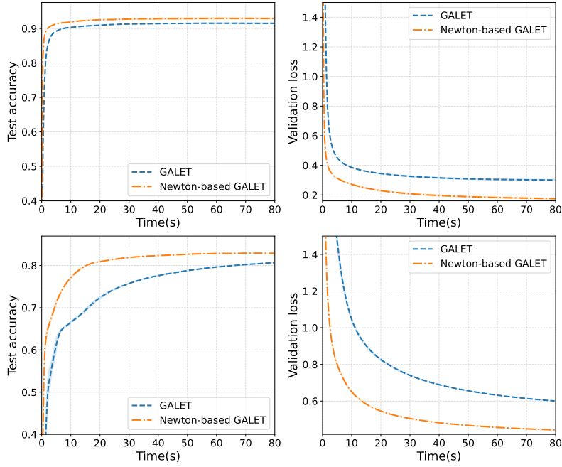
Figure 6: Data hyper-cleaning with two-layer MLPs. Comparison of GALET and Newton-based GALET on MNIST (upper) and FashionMNIST (lower).
