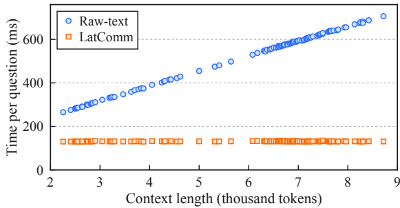
Figure 7: Receiver time per question against the context length on QuALITY. Each point is one article.
