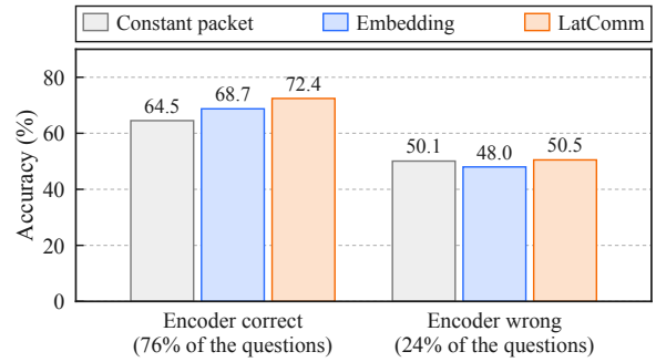
Figure 6: Accuracy on the test questions that the Qwen3.5-4B encoder answers correctly or wrongly from the full text. Embedding uses BGE-Gemma2.
