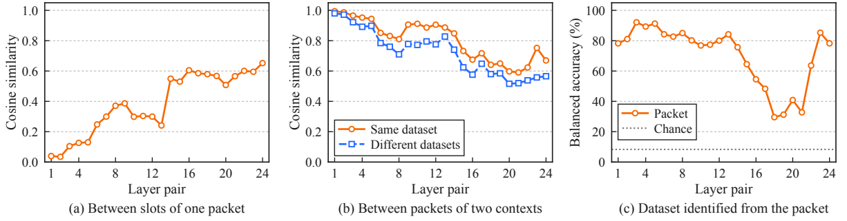
Figure 9: Packets of the default pair at each layer pair. (a) Mean cosine similarity between two slots of one packet. (b) Mean cosine similarity between the packets of two contexts from the same dataset or from different datasets. (c) Balanced accuracy of identifying the source dataset of a context from its packet.
