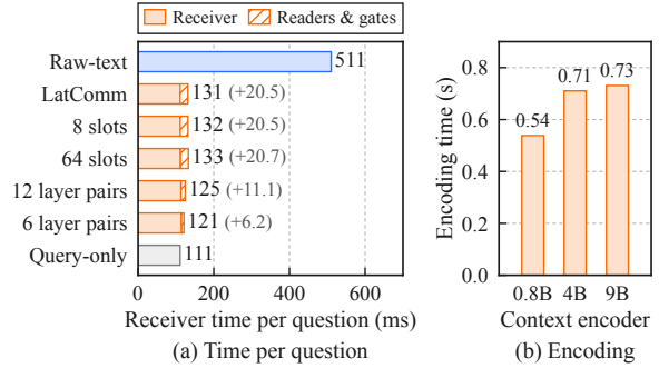
Figure 4: Reuse cost on QuALITY. (a) Receiver time per question for Raw-text, five LatComm settings, and Query-only. The hatched part of a bar is the time added by the readers and gates. (b) Encoding time per context for three context encoders.
