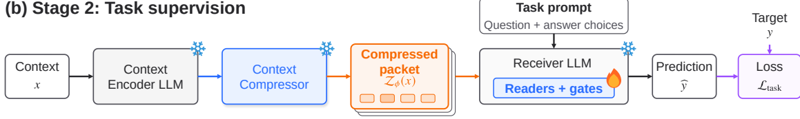
Figure 3: Two-stage training of LatComm. (a) In Stage 1, the receiver gets an instruction to reproduce the context x and can read it only from the packet \mathcal{Z}_\phi(x) . The reconstruction loss \mathcal{L}_{\text{rec}} trains the compressors, readers, and gates. (b) In Stage 2, the receiver gets the question with its answer choices, and the task loss \mathcal{L}_{\text{task}} on the answer y trains only the readers and gates. The compressors are fixed, so the packet of each training context is computed once and stored. Both LLMs stay frozen in both stages.
