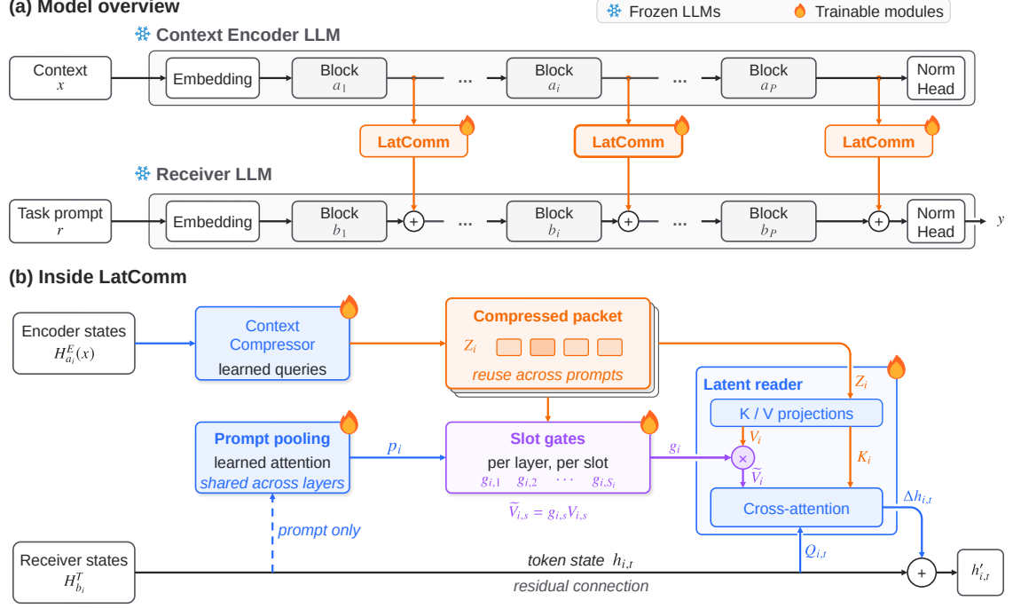
Figure 2: LatComm overview. (a) The encoder reads the context; the receiver reads a task prompt. LatComm connects selected layers and adds context information after each paired receiver block. Both LLMs remain frozen. (b) For one layer pair, a context compressor produces reusable slots Z_i . The gates compare a summary of the receiver’s prompt states with the compressed slots. The reader combines the gated slot values and adds the result to the receiver state.
