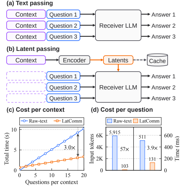
Figure 1: Text passing vs. latent passing. (a) The receiver reads the context again for every question. (b) The context is encoded once and reused. (c, d) Measured cost on QuALITY.
