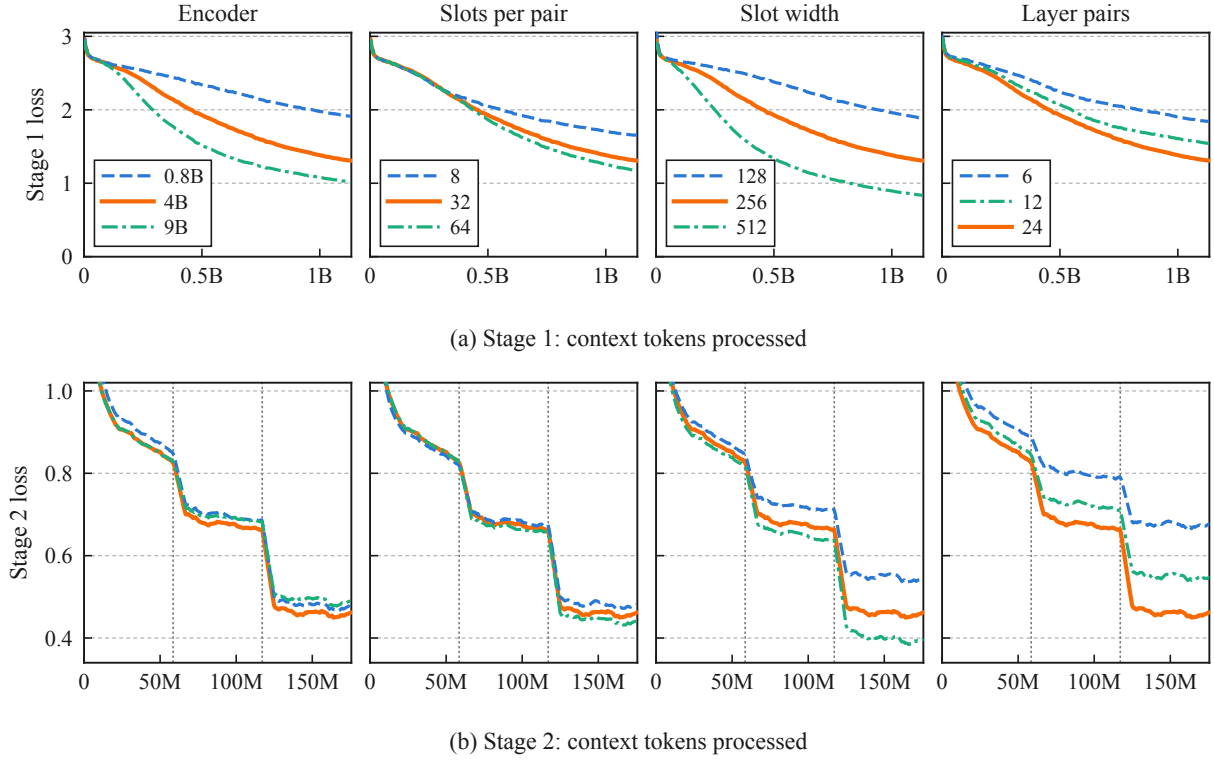
Figure 5: Training loss of (a) Stage 1 and (b) Stage 2 against the number of context tokens processed, for the configurations of Table 10. Each column changes one setting, and the solid orange line is the default configuration. The token count is the number of processed examples times the mean context length of the training set. The curves are running means over 50 updates in Stage 1 and 100 updates in Stage 2. Dotted lines mark the ends of the first and second epochs of Stage 2.
