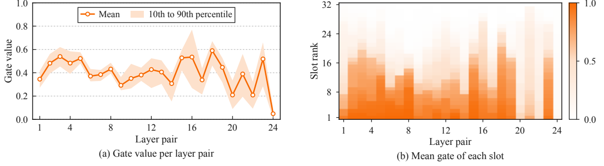
Figure 8: Gate values of the default pair on 5,386 test questions. (a) Mean over the 32 slots of each layer pair. The band covers the 10th to 90th percentile of the questions. (b) Mean gate of each slot. The slots of a layer pair are sorted from the highest mean gate to the lowest.
