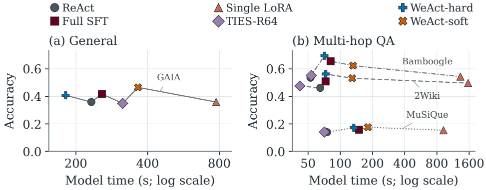
Figure 8: Accuracy versus model-path time on General and Multi-hop QA. Points pair Table 1 accuracy with historical mean cumulative time, including retries. Colors and markers identify methods; line styles group benchmarks. Time axes are logarithmic in seconds.
