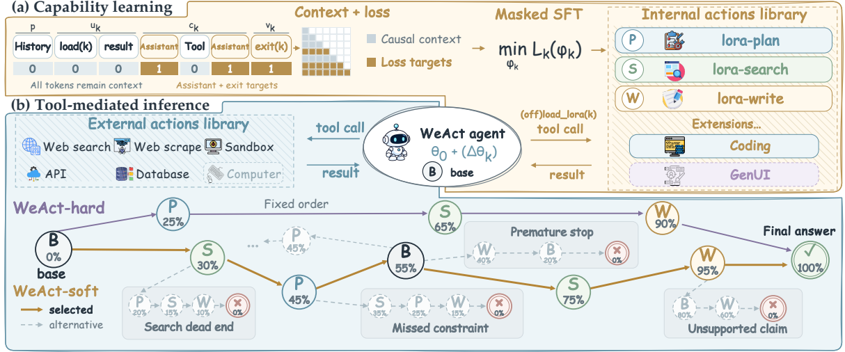
Figure 2: WeAct overview. (a) Capability learning builds the adapter library. (b) Tool-mediated inference switches adapters through internal tool calls and interacts with the environment through external tools. B/P/S/W nodes denote base/Plan/Search/Writing states; solid and dashed arrows indicate selected and alternative execution paths.
