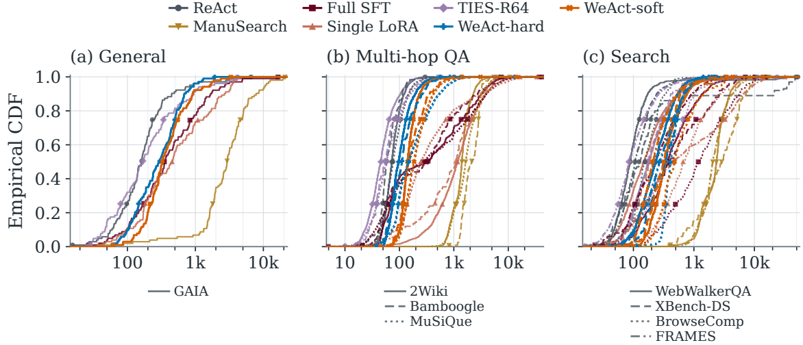
Figure 9: Historical task-record wall-clock distributions. Colors and markers identify methods; line styles identify benchmarks. Each panel uses its own logarithmic time axis in seconds and retains all tails. Curves include all valid task-record times and saved retries, regardless of correctness; logged wall time can include post-answer judging.
