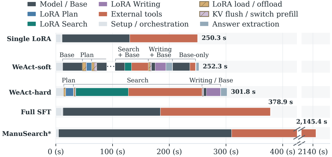
Figure 10: Runtime decomposition on WebWalkerQA with 50 runs per method. Bars show stage-aligned means. The ellipsis denotes repeated capability switching; all durations are retained. ManuSearch* is a historical reference with unmatched deployment and tool conditions.
