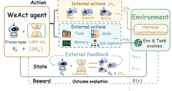
Figure 1: Internal actions extend the agent’s action space. WeAct selects LoRA adapters internally and interacts with the environment through external actions.
