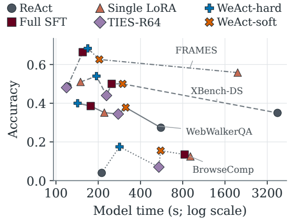
Figure 5: Accuracy versus historical mean cumulative model-path time on four Search benchmarks. Times include saved retries.
