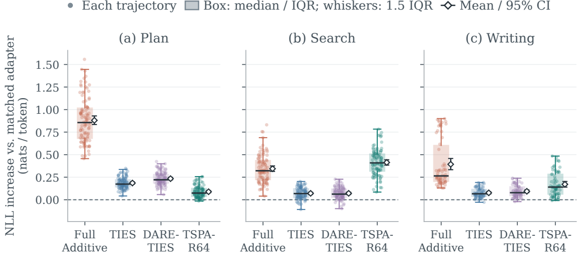
Figure 14: Paired target-token NLL gaps relative to Individual. Points show validation records, boxes show medians and interquartile ranges, and diamonds mark means with 95% confidence intervals.
