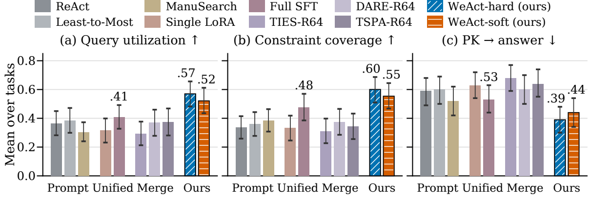
Figure 4: SearchAtlas trace diagnostics. Query utilization: fraction of queries supporting the answer; constraint coverage: fraction of question constraints covered by those queries; PK→answer: share of answers with unsupported content attributed to prior knowledge. Error bars are 95% task-bootstrap intervals.
