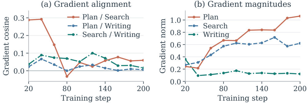
Figure 12: Gradient alignment and magnitude in the Single-LoRA pilot. (a) Pairwise cosines and (b) gradient norms at ten checkpoints of a rank-96 Single-LoRA run on frozen QWEN3-32B. Most pairwise cosines are positive, while gradient magnitudes differ across capabilities.
