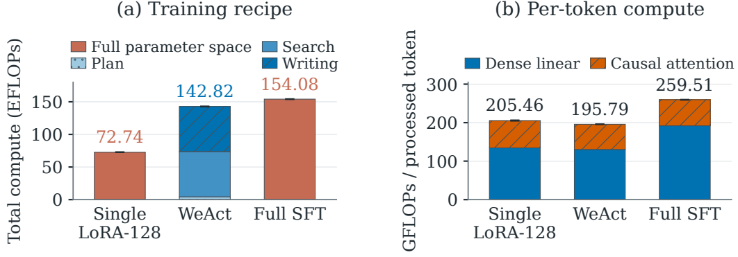
Figure 7: Nominal training compute. (a) Total recipe compute, with WeAct split by capability. (b) Dense and causal-attention FLOPs per token. Error bars show length-statistic uncertainty (details in text).
