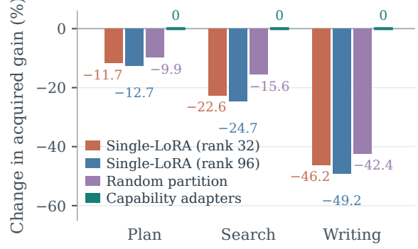
Figure 3: Capability retention under sequential training. Detailed results are reported in Appendix Table 7.
