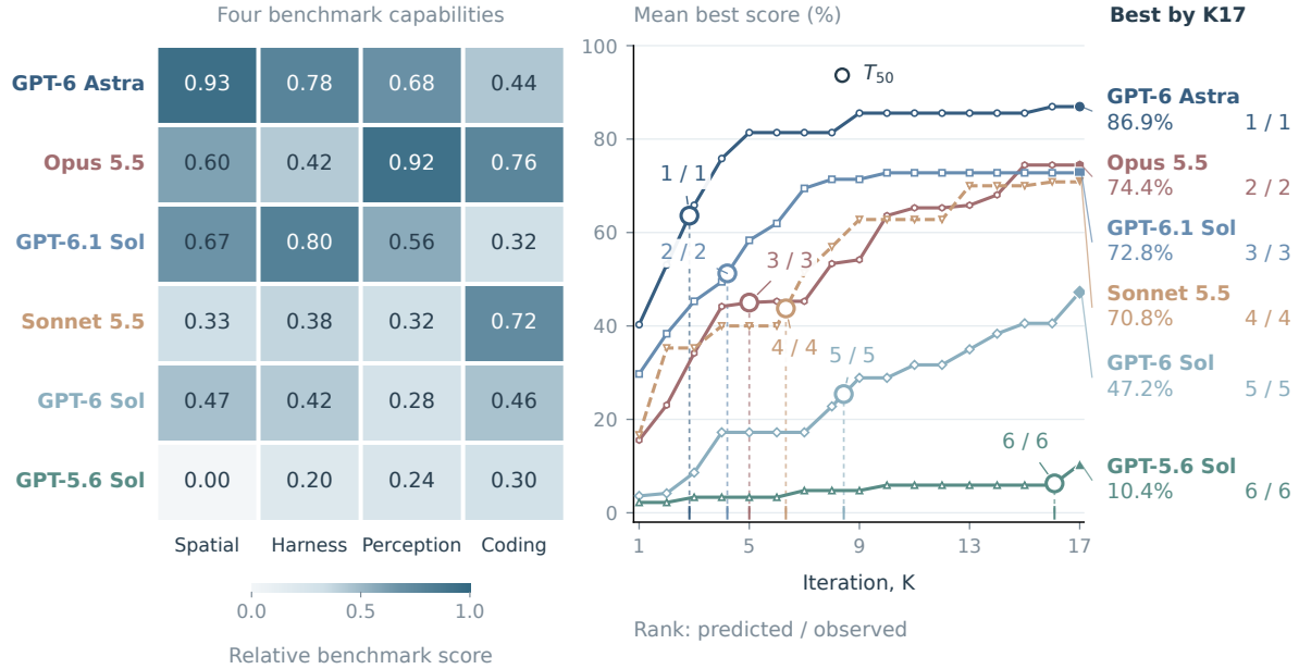
Figure 7 Predicting the timing of gains from public capability profiles. Left: four capability profiles of each system, computed from 17 public benchmarks as normalized ranks among the six systems. Right: best mean score \bar{q}_k on the 18 tasks. Circles mark T_{50} , the first round at which \bar{q}_k reaches half of its K1–K17 gain. Labels give predicted / observed ranks: T_{50} beside the circles and best score reached by K17 on the right. Each pair of systems is predicted from the other four.
