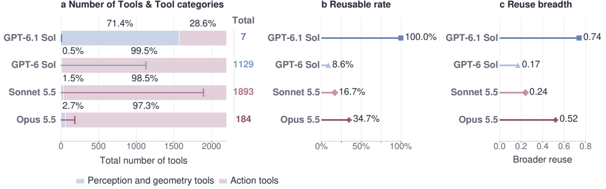
Figure 10 Tool Libraries and Reuse across Models. (a) Total tool counts and the proportions of perception and geometry tools versus action tools. (b) Fraction of tool lineages reused in subsequent rounds, among those with later rounds available. Reuse includes direct use, modification and derivation of existing tools. (c) Reuse breadth, defined as one minus the share of subsequent calls accounted for by the top 10% of reused lineages. Higher values indicate reuse distributed across more lineages. Astra is omitted because it creates very few tools, used only for verification. GPT-6.1 Sol’s estimates reflect a small library of seven tools.
