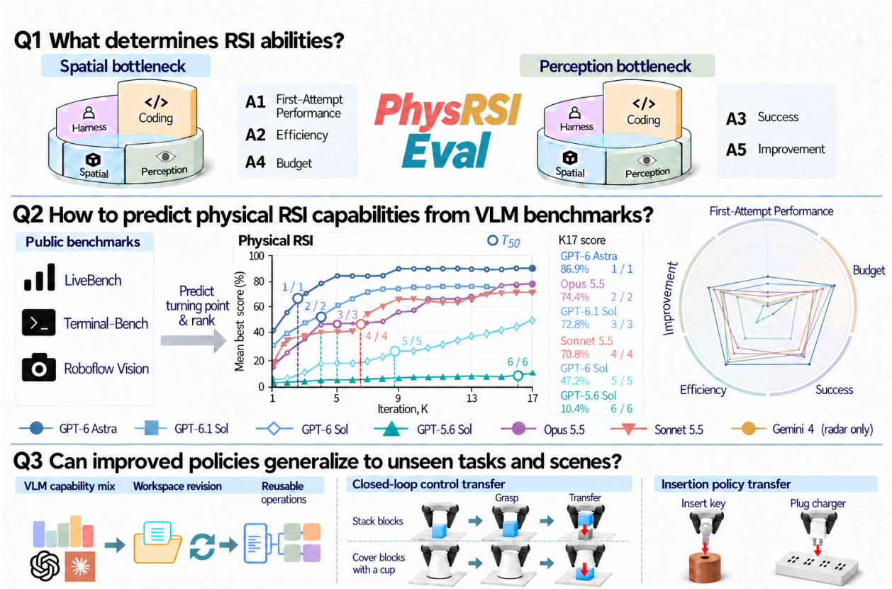
Figure 1 PhysRSI-eval at a glance. (Q1) Capability sources and the Physical Barrel Hypothesis. (Q2) Five-axis quantification and observational scaling of performance, gain timing and model rankings. T_{50} is the half-gain round, the first round at which the best mean score reaches half of its K1-K17 gain. (Q3) Overfitting and generalization across tasks and scenes.
