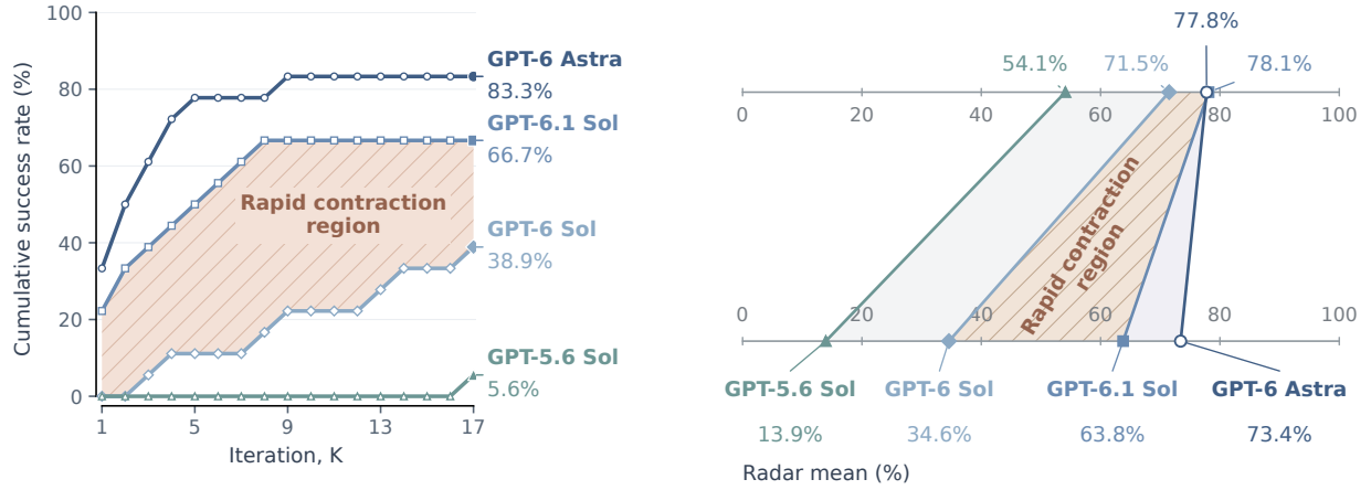
Figure 6 Public capability and physical RSI separate differently. Left: cumulative success during refinement on 18 tasks; the shaded region marks the gap between GPT-6.1 Sol and GPT-6 Sol. Right: mean public score over 17 selected benchmarks versus 100 \times (A_1 + A_2 + A_3 + A_4 + A_5)/5 . The physical summary is an arithmetic mean, not radar area.
