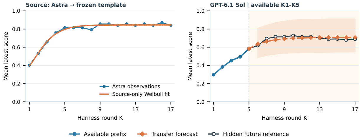
Figure 8 Forecasting GPT-6.1 Sol from Astra’s improvement shape. Left: Astra’s mean score and the Weibull template fitted to it. Right: GPT-6.1 Sol with K1–K5 available. The template is calibrated on these rounds and forecasts the hidden rounds through K17; shading shows the 90% paired-task bootstrap band. All 18 tasks are used.
