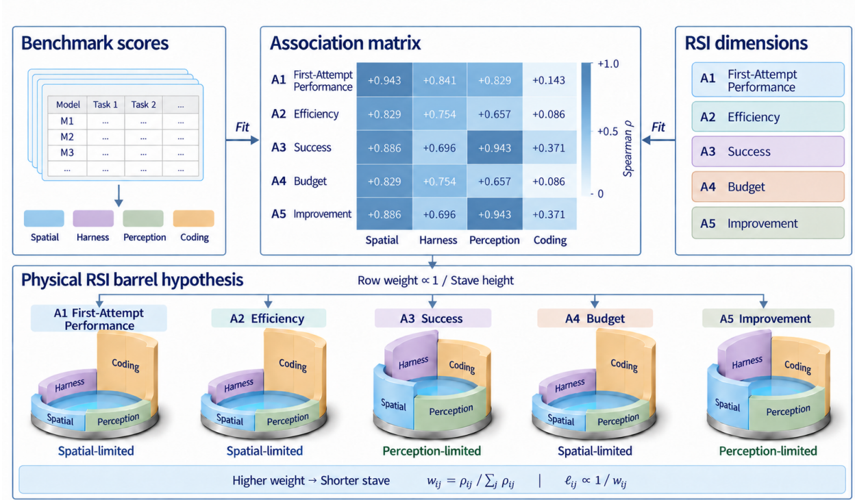
Figure 4 Capability associations and the barrel hypothesis. The matrix reports exploratory rank associations across six systems on the 18 tasks. Each barrel represents one RSI axis, with a stave per capability group. Stave heights illustrate a proposed bottleneck interpretation of the associations.
