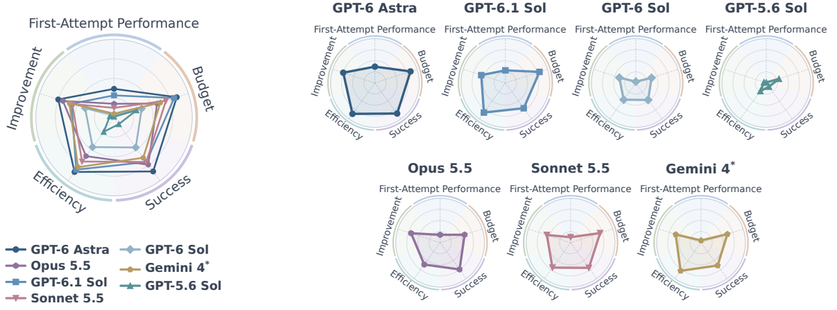
Figure 5 Five-axis profiles. Left: seven overlaid profiles. Right: one panel per system. Axes clockwise from the top are First-Attempt Performance (A1), Budget (A4), Success (A3), Efficiency (A2) and Improvement (A5), on a shared 0–1 scale. The six reference systems use all 18 tasks, as in Table 1; *Gemini 4 uses its ten evaluated tasks (Section 3.3).
