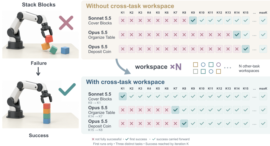
Figure 9 Cross-task workspace transfer. Top: original self-improvement trajectories for tasks first solved at K6 or later. Bottom: trajectories initialized from a workspace pooled from all other tasks, excluding the target task. First success advances from K9 to K1 for Sonnet 5.5 on Cover Blocks, from K14 to K7 for Opus 5.5 on Organize Table, and from K15 to K8 for Opus 5.5 on Deposit Coin. These examples illustrate faster adaptation with transferred workspaces. Red crosses indicate unsuccessful attempts, dark checks mark first success, and pale checks carry success forward without additional evaluation.
