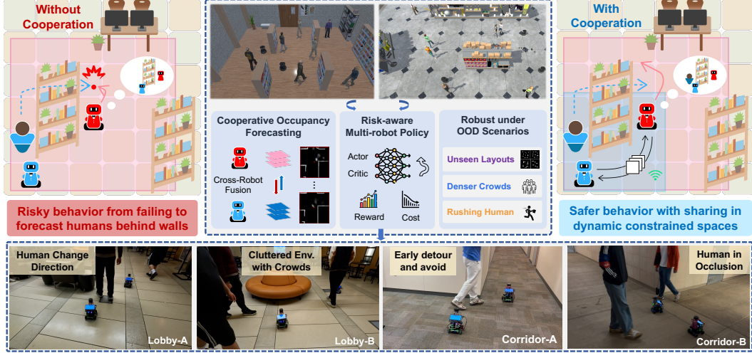
Figure 1: The single-agent approach relies only on the robot’s own observations and misses an incoming pedestrian behind the obstacle. In contrast, CoopUQ fuses shared information, anticipates dynamic motions under uncertainty, and plans a safe trajectory. Closed-loop experiments in Unity-3D simulation demonstrate robustness in OOD scenarios, and the learned policy transfers directly to various real-world environments, achieving safe navigation across diverse crowds and layouts.
