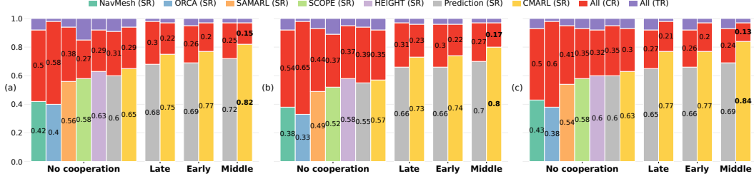
Figure 3: OOD test results in (a) unseen layouts, (b) denser crowds, and (c) rushing pedestrians.
