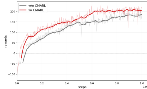
Figure 7: Training reward comparison with and without CMARL. The CMARL policy achieves faster convergence and higher final rewards, indicating that cost constraints do not merely improve safety but also facilitate efficient policy learning.
