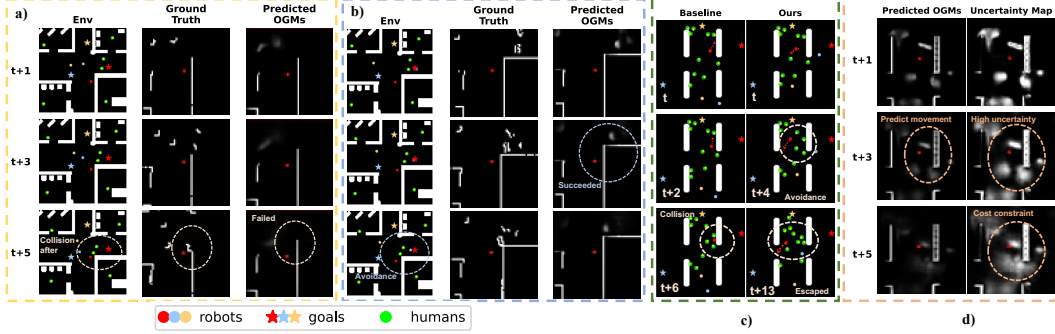
Figure 4: (a) Prediction w/o cooperation: The red robot reacts only after the human fully emerges into its view, resulting in a sharp brake and collision. (b) Prediction w/ cooperation: The red robot decelerates and changes direction earlier to avoid a collision. (c) Key frames of navigation w/o and w/ cooperation. (d) Prediction and uncertainty map from ours at step t . The red ego robot proactively avoids entering high-uncertainty areas due to cost constraints, thus preventing potential collisions.
