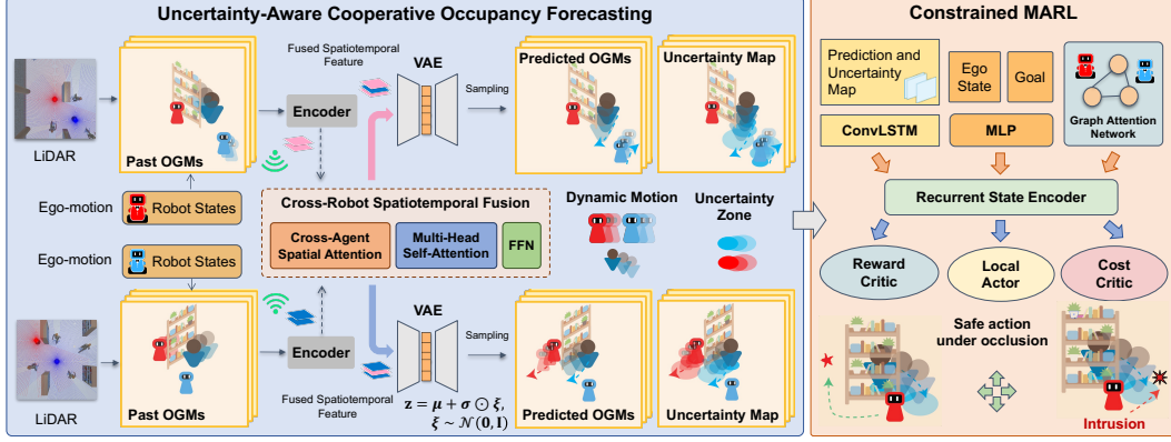
Figure 2: The overall architecture of the CoopUQ for multi-robot social navigation.
