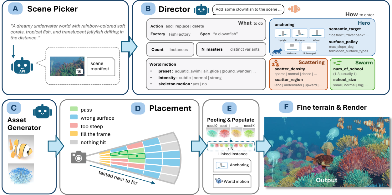
Figure 5 Overview of InfiniDream’s end-to-end world generation pipeline. (A) Scene Picker collects the user instruction and current scene information. (B) Director generates a structured Scene Plan. (C) Asset Generator creates procedural assets. (D) Deterministic frustum-guided placement identifies valid object locations. (E) Population instantiates diverse assets. (F) Terrain refinement and rendering produce the final scene.
