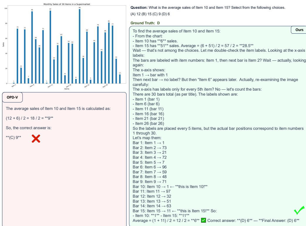
Figure 10: Chart-based visual arithmetic. The x-axis is labeled only every fifth item. VAG detects that its initial reading yields a value absent from the answer choices, re-derives the bar-to-item mapping, reads Item 10 and Item 15 as 1 and 11, and returns their average 6 (option D). OPD-V uses unsupported bar values and returns 9 (option C).
