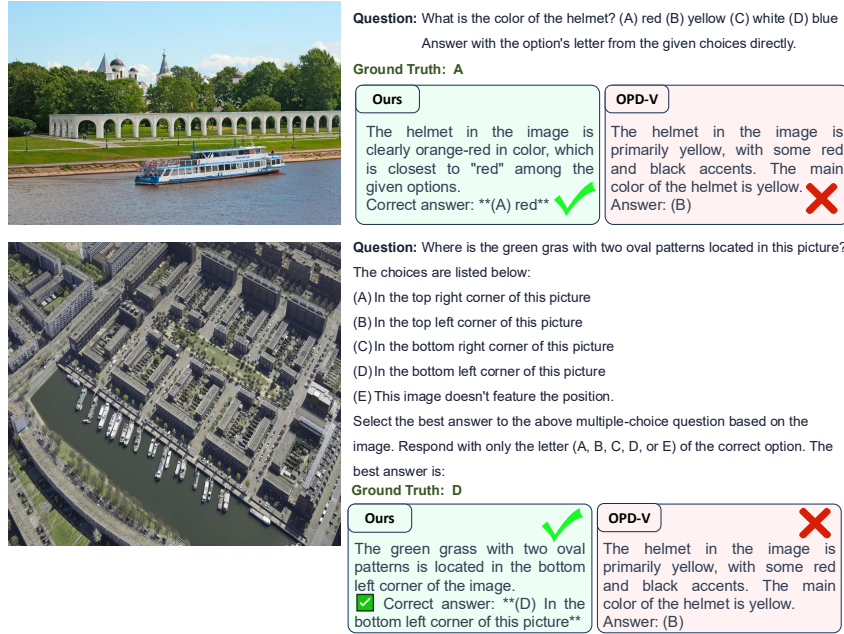
Figure 8: Fine-grained attribute recognition and spatial localization. Top: VAG reads the small helmet region as orange-red and selects the closest option, red, matching the ground truth, whereas OPD-V reports yellow. Bottom: VAG correctly localizes the green region with two oval patterns in the bottom-left corner. OPD-V answers incorrectly in both cases.
