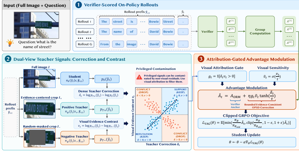
Figure 3: Overview of the VAG framework. Stage 1: A verifier derives A_{\text{ORM}} from on-policy rollouts. Stage 2: Dual-view teacher evaluation yields the distillation margin \delta_t and visual contrast v_t ; VAG retains same-sign corrections and discards conflicting ones. Stage 3: The retained correction modulates A_{\text{ORM}} for the clipped GRPO update.
