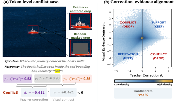
Figure 1: Illustrative contamination diagnostic. (a) A token-level conflict case and (b) the correction-evidence alignment used to motivate attribution.
