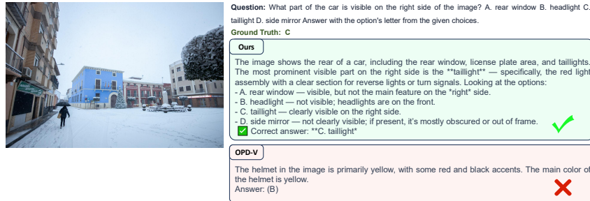
Figure 9: Object-part recognition. VAG rules out the parts that are not visible in the frame and identifies the part on the right side of the car as the taillight (option C), matching the ground truth, whereas OPD-V selects an incorrect option.
