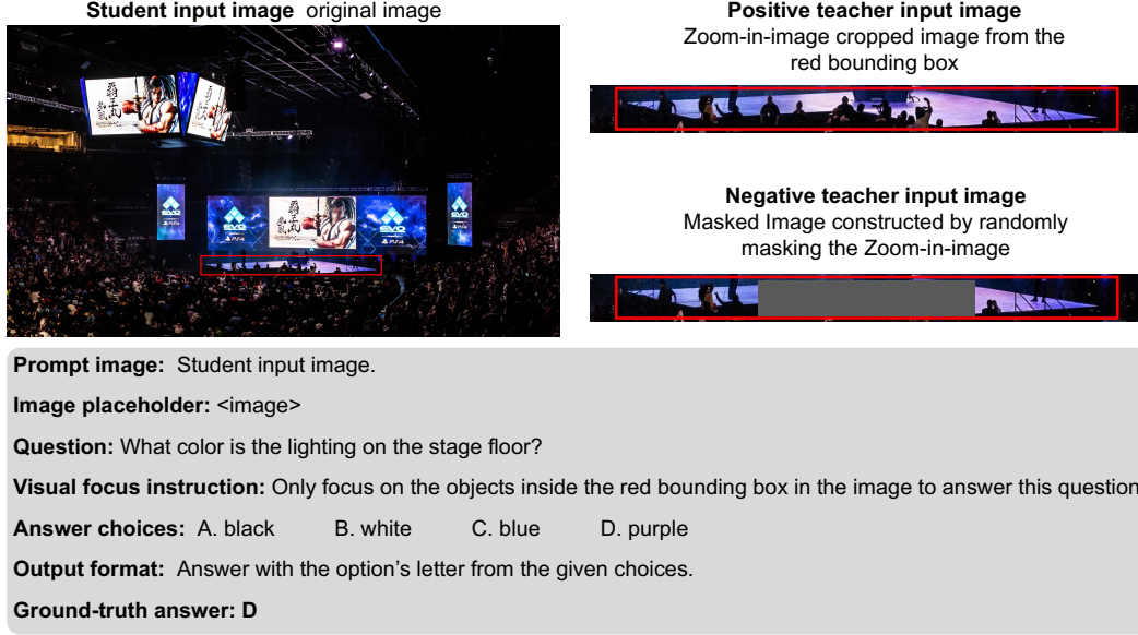
Figure 6: Training prompt and paired visual inputs. The textual prompt, comprising the image placeholder, question, visual focus instruction, answer choices, and output format, is shared across all three passes. The student is conditioned on the original image, the positive teacher on the evidence-centered crop given by the red bounding box, and the negative teacher on a randomly masked version of that crop. The ground-truth answer is used only by the verifier.
