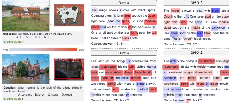
Figure 5: Prediction and token-importance comparison. VAG produces the correct evidence-grounded prediction and concentrates credit on decision-relevant visual tokens.
