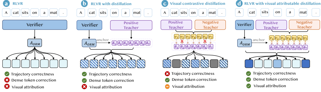
Figure 2: Comparison of on-policy learning paradigms. (a) RLVR, (b) RLVR with distillation, (c) Visual contrastive distillation, and (d) RLVR with visual attributable distillation.
