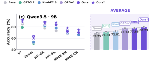
Figure 4: Performance comparison on Qwen3.5-9B.
