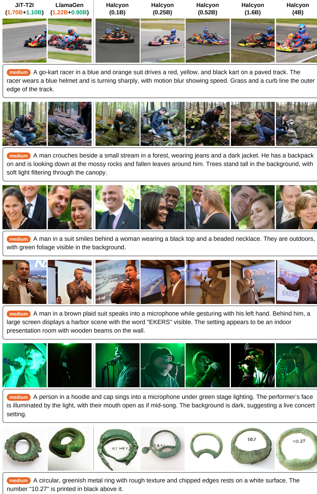
Figure 13: Comparison of generated images with “medium” captions. From left to right: JiT-T2I-XXL/8++, LlamaGen-XL/8, and Halcyon from 0.1B to 4B. For the baselines, we report the sizes of the language model and image generator separately. Image quality improves as Halcyon scales up. All prompts are from GPIC Test-50K.
