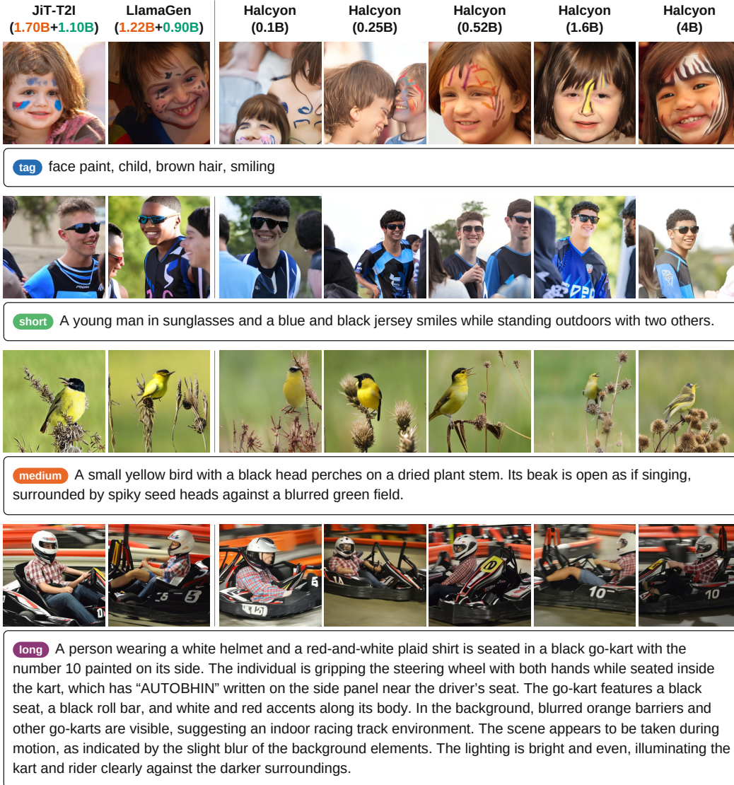
Figure 5: Comparison of generated images. From left to right: JiT-T2I-XXL/8++, LlamaGen-XL/8, and Halcyon models from 0.1B to 4B parameters. For the baselines, we report the sizes of the language model and image generator separately. Image quality improves as Halcyon scales up. All prompts are from GPIC Test-50K. Additional samples are provided in Appendix D.
