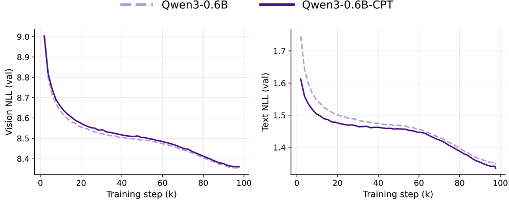
Figure 10: Effect of language pretraining on validation NLL. Validation NLL for image tokens conditioned on text ( \mathcal{I} \mid \mathcal{T} , left) and text tokens without conditioning ( \mathcal{T} \mid \emptyset , right) during training of Qwen3-0.6B with random vs. language-pretrained initialization. Random initialization consistently achieves lower image NLL, while language-pretrained initialization achieves lower text NLL.
