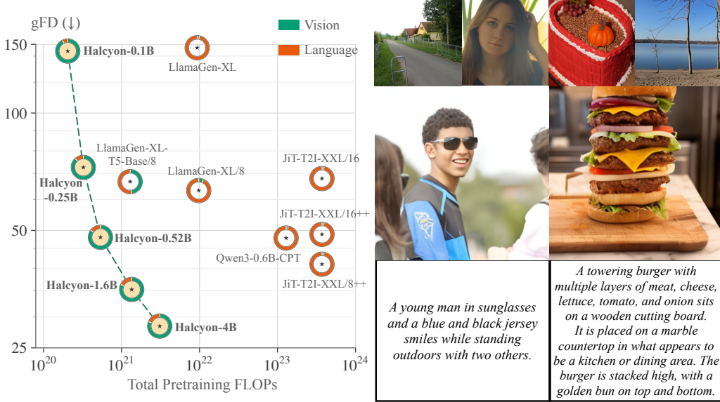
Figure 1: Text-to-image generation without internet-scale language pretraining. Left: Generation quality on GPIC (Chandrasegaran et al., 2026) (gFD, log scale) vs. total pretraining FLOPs required to build each T2I system, including language model, image tokenizer, and image generator pretraining. Each \star marks total pretraining FLOPs and gFD, while the donut breaks down language and vision compute. Halcyon (Ours) , trained entirely from scratch, achieves lower gFD with substantially lower total pretraining compute compared to: (i) LlamaGen (Sun et al., 2024), late-fusion autoregressive models with 0.78–0.90B image generators and pretrained FLAN-T5 encoders (0.11–1.22B); (ii) JiT-T2I (Li & He, 2026; Ma et al., 2026), late-fusion diffusion models with a 1.10B image generator and pretrained Qwen3-1.7B; and (iii) Qwen3-0.6B-CPT , an autoregressive model continually pretrained on image–text pairs, initialized from a pretrained Qwen3-0.6B language model (Yang et al., 2025a). Right: 256 \times 256 samples generated by Halcyon-4B with prompts shown for two samples. Best viewed in color.
