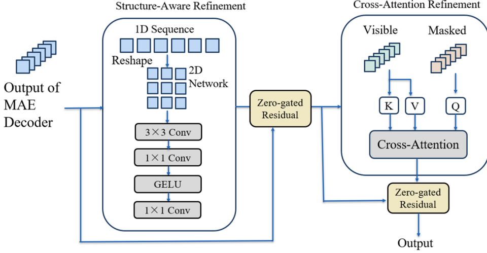
Figure 2: Conceptual illustration of the two appended refinement operations, adapted from the original project report. The actual implementation uses depthwise convolution and pre-normalization in the local branch, plus separately zero-gated cross-attention and MLP updates in each cross-refinement block (Equations 2–6).
