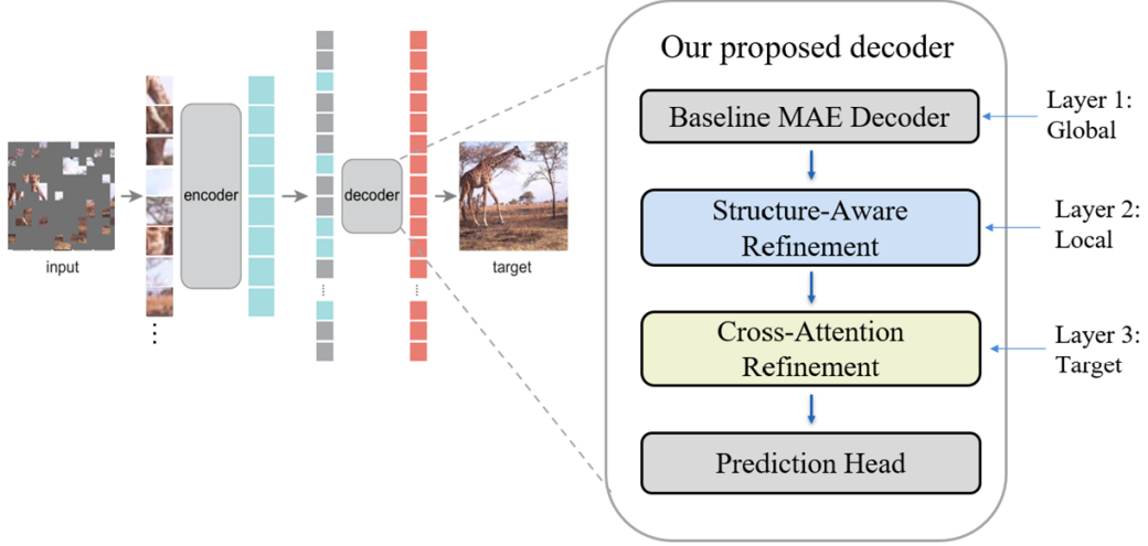
Figure 1: High-level WildMAE pipeline: the original MAE encoder and Transformer decoder are retained, followed by a local spatial refinement, masked-to-visible contextual refinement, and the pixel-prediction head. Exact internal normalizations and residual gates are specified in Sections 3.2–3.3. The diagram is conceptual.
