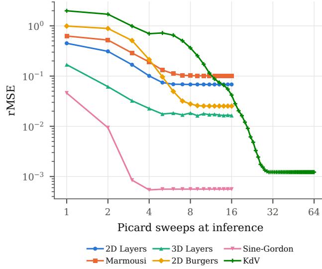
Figure 4: rMSE of the trained PaPi models after k cold Picard–Duhamel sweeps from the linear flow, mean over five seeds. Every problem but KdV is converged by eight sweeps.
