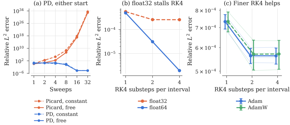
Figure 7: The PD gain comes from the update, and part of the training error comes from time integration. (a) Both updates from both initial paths (401 nodes). (b) Exact-force RK4 in float32 and float64. (c) Frozen Adam and AdamW models evaluated with finer RK4. Panels (b,c) score the original 201 nodes.
