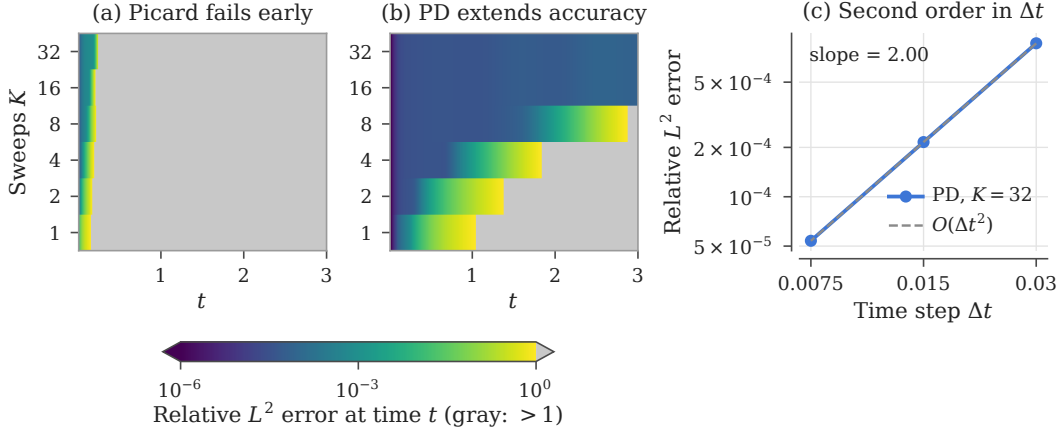
Figure 5: Each PD sweep extends the accurate time window, while Picard fails early at every budget. (a,b) Error at each time t on the 401-node grid (gray: above one); the bottom PD row is the Duhamel solution. (c) Once converged ( K = 32 ), PD error falls at exactly second order in \Delta t .
