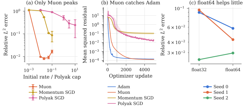
Figure 8: Given enough updates Muon matches Adam, while float64 does not rescue L-BFGS. (a) Extended step-size ranges at 1,000 updates. (b) Residuals continued to 5,000 updates: seed median with min–max band, smoothed by a 51-update running median (dotted line: original budget). (c) L-BFGS in float32 and float64 from identical initial parameters.
