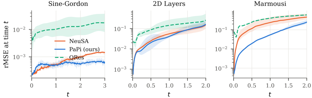
Figure 3: Relative L^2 error at each time t (mean over five seeds, band from best to worst seed) for PaPi, NeuSA and the best MLP-based baseline, QRes.
