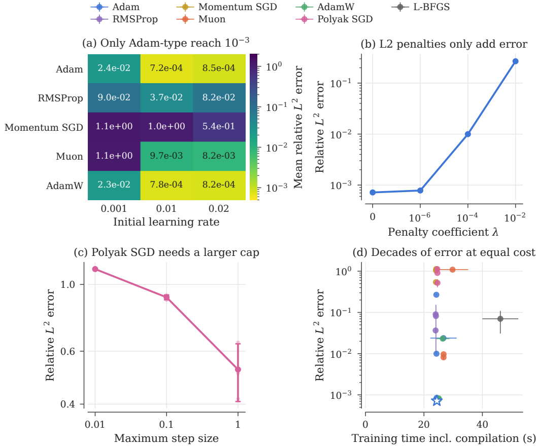
Figure 6: Step size and optimizer family determine accuracy; regularization only adds error. (a) Mean error per optimizer and initial learning rate. (b) L2 penalty for Adam at \eta_0 = 0.01 . (c) Polyak SGD step-size cap. (d) All configurations against training time; the star marks Adam at \eta_0 = 0.01 . Error bars are standard deviations over three seeds.
