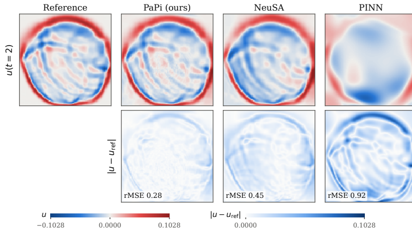
Figure 1: Wave equation in the Marmousi medium at t = 2 (seed 0): the displacement u on the region of interest [-2, 2]^2 (top) and the absolute error against the reference (bottom), with the relative L^2 error at this time in each error tile. PaPi resolves the reflected and refracted fronts that NeuSA blurs and the PINN misses.
