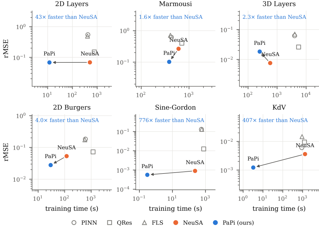
Figure 2: Training time against rMSE on every benchmark of Table 1 (means over five seeds, one RTX 5090). The arrow joins NeuSA to PaPi: the same model, trained through the parallel Picard–Duhamel rollout instead of the sequential RK4 one.
