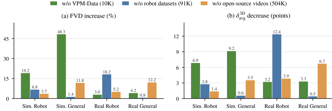
Figure 10: Ablation on training data sources. Relative FVD increase (a) and \delta_{\text{avg}}^{\text{3D}} decrease (b) of VPM (V+T) when one source is removed from training, measured against the model trained on all sources. Higher is worse.
