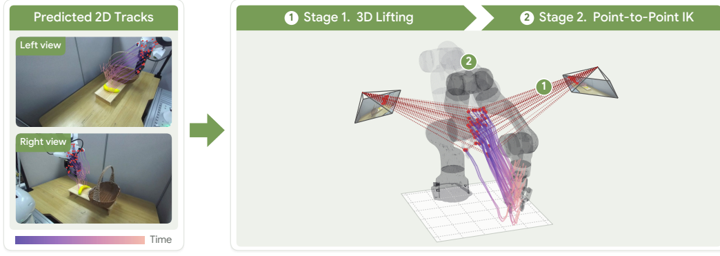
Figure 7: From predicted point trajectories to joint-space actions. Predicted 2D trajectories from both views are lifted to 3D (Stage 1) and converted into a joint trajectory by fitting the robot’s kinematic model to the lifted points (Stage 2).
