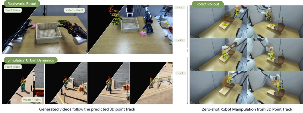
Figure 4: Predicted 3D point trajectories guide generation and action. Left: Predicted trajectories alone and overlaid on generated videos. Right: Zero-shot real-robot rollout obtained by converting predicted trajectories into commands with inverse kinematics.
