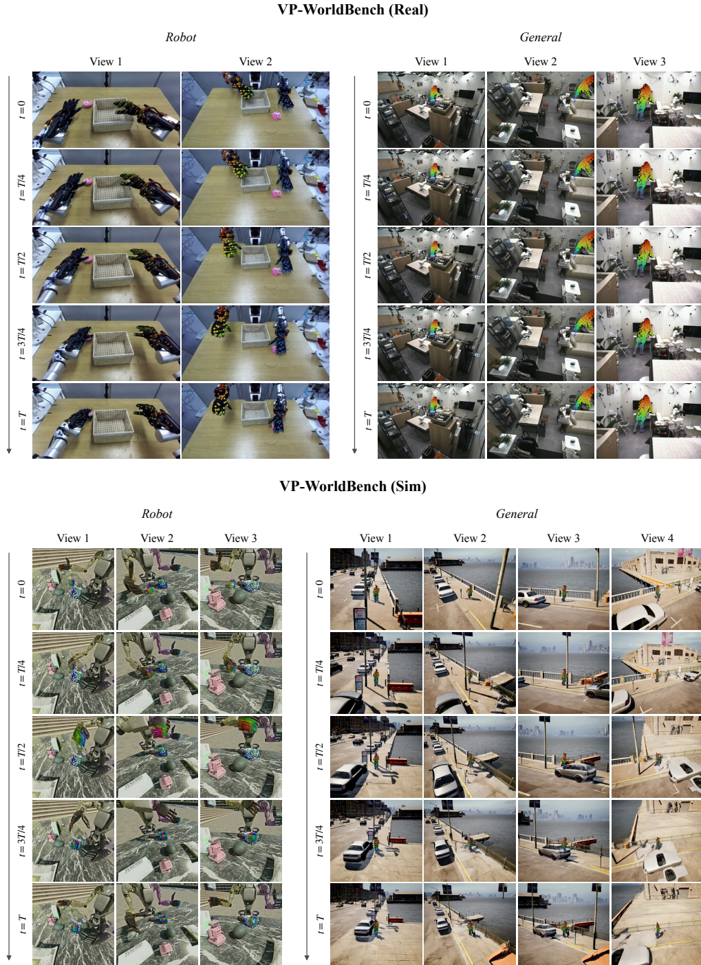
Figure 12: Additional qualitative results of multi-view prediction. Predicted video with overlaid predicted point track on robot and general scenes from VP-WorldBench (Real, top) and VP-WorldBench (Sim, bottom).
