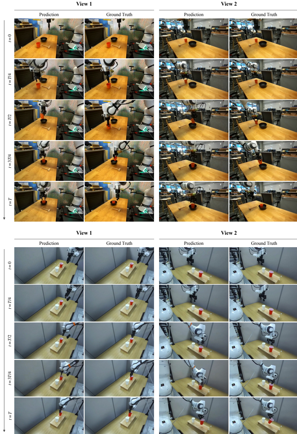
Figure 13: Predicted vs. ground-truth videos. Each view shows the prediction next to the ground truth. Conditioning frames are omitted.
