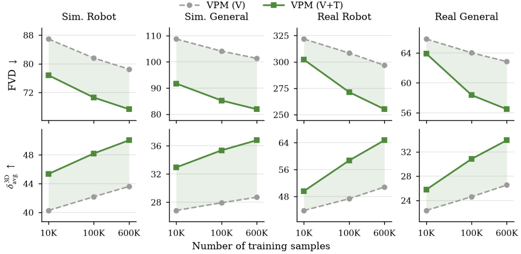
Figure 9: Data scalability. FVD (top) and \delta_{avg}^{3D} (bottom) of VPM (V) and VPM (V+T) trained on 10K, 100K, and 600K samples. The shaded area marks the gain from point supervision.
