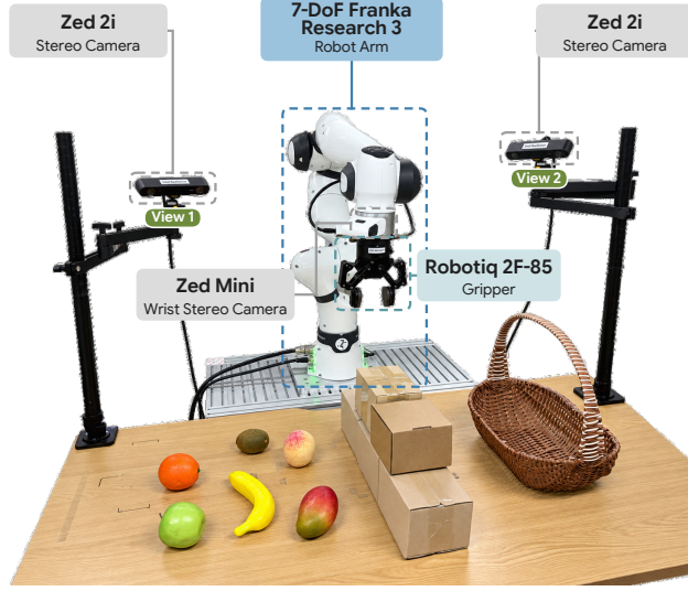
Figure 5: Real-world hardware platform. A 7-DoF Franka Research 3 robot arm equipped with a Robotiq 2F-85 gripper and a wrist-mounted Zed Mini stereo camera. Two external Zed 2i stereo cameras (view 1 and view 2) observe the workspace from different viewpoints, providing synchronized multi-view observations.
