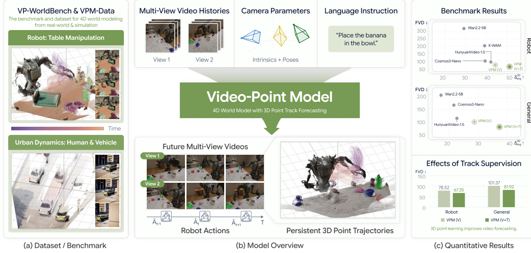
Figure 1: Teaser. We introduce simulated and real-world multi-view videos paired with 3D point tracks (left), jointly forecast future videos and point trajectories (center), and show that point supervision improves visual forecasting (right).
