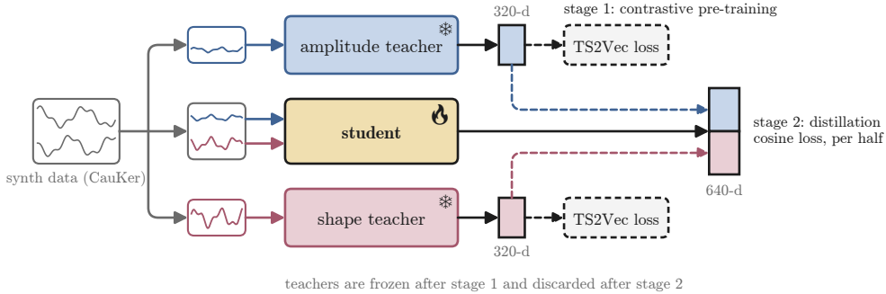
Figure 1: TS2Vec-FM architecture and training. (a) Raw and instance-normalized inputs pass through an MLP and a linear stem, respectively. Their concatenation feeds a shared convolutional trunk and temporal max pooling. (b) Two specialists are pretrained on synthetic data with the TS2Vec objective and then frozen. On the same data, each teacher supervises one 320-dimensional half of the student through timestamp-level and pooled cosine losses. Downstream, only a classifier on frozen student features is fitted.
