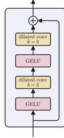
Figure 3: One TS2Vec residual block: two GELU–dilated-convolution pairs plus a skip connection (identity, or a 1 \times 1 convolution when the width changes).
