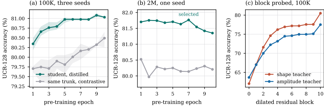
Figure 4: Colours are shared across panels; accuracy is UCR-128 with the random-forest probe. (a) At 100K, the distilled student stabilizes after the first few epochs and remains above the same trunk trained contrastively; bands span the three pre-training seeds. (b) At 2M (one seed) the student peaks at epoch 7 and then declines, while the gradient-clipped contrastive control stays within 0.56 pp of its epoch-1 accuracy across ten epochs. (c) Probing each dilated residual block of the two 100K specialists: accuracy increases with depth and the final block is best for both.
