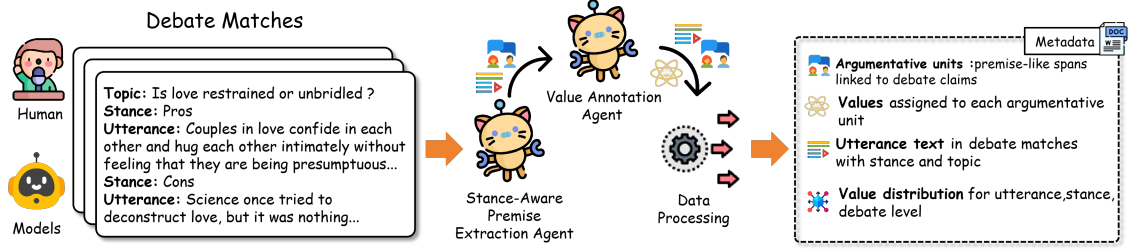
Figure 3: Operational pipeline. Transcripts are structured with metadata, processed by SAPE-Agent (premise extraction and argumentative-unit construction) and VA-Agent (Basic-10 value annotation), then aggregated into utterance-, stance-, and debate-level representations for metric computation.
