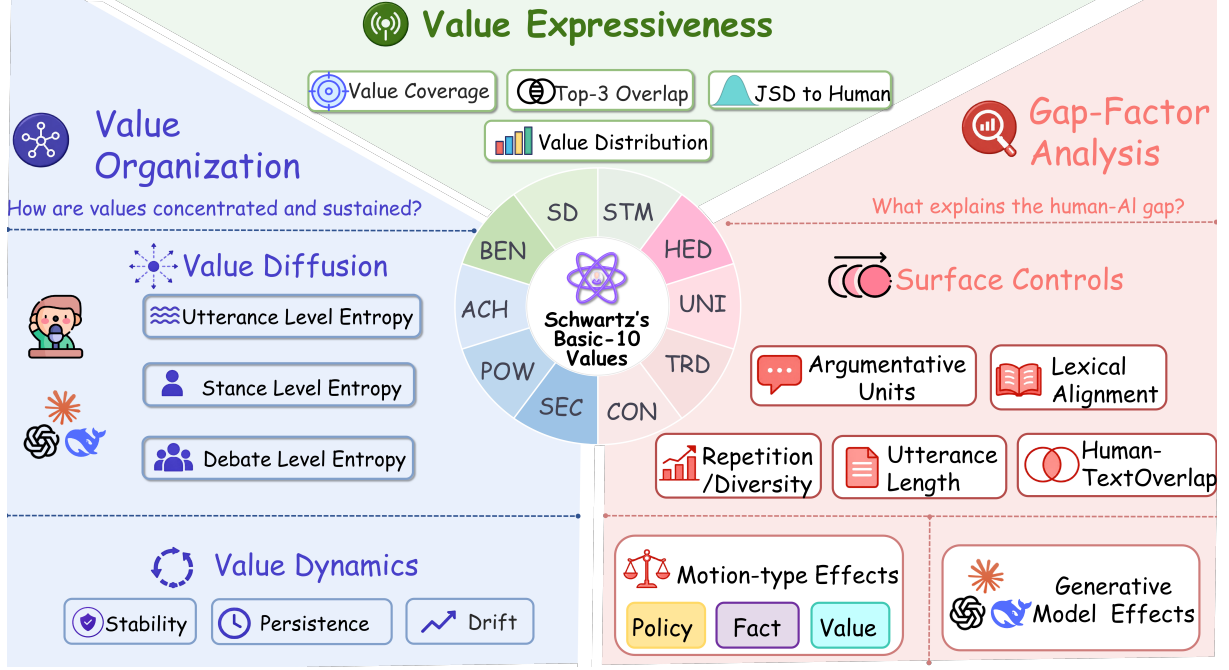
Figure 2: Conceptual framework. The shared Schwartz Basic-10 space (center) grounds two evaluation dimensions: value expression (breadth of value activation) and value organization (concentration and cross-turn dynamics). The right panel shows how paired differences are interpreted through surface controls, motion-type effects, and generation-system effects. Here, Human-TextOverlap denotes BLEU similarity between a generated debate and its matched human reference.
