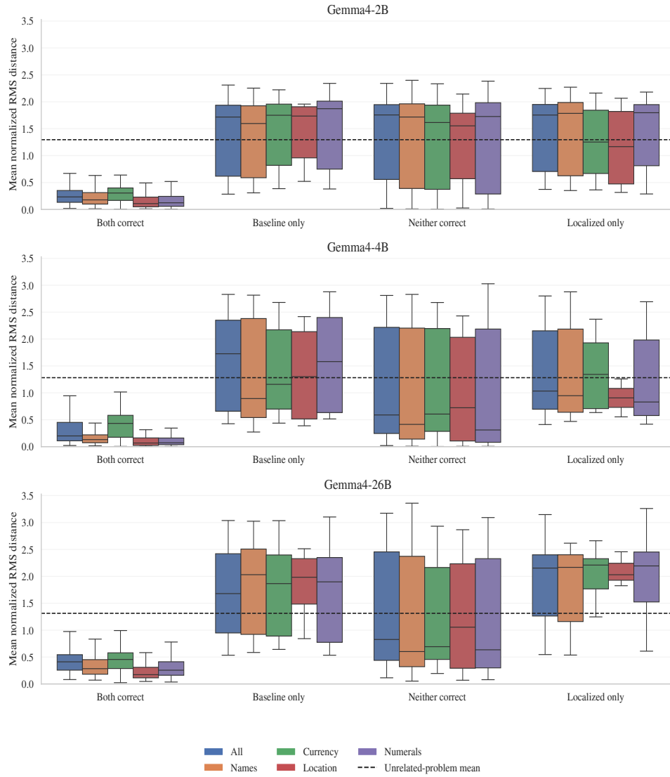
Figure 5: Residual-stream RMS distance by paired correctness group. Discordant examples show substantially larger trajectory separation than examples that remain correct in both conditions.
