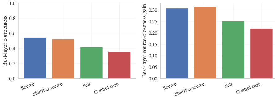
Figure 3: Activation patching correctness by baseline. Source patching partially recovers source-condition behavior on discordant examples.
