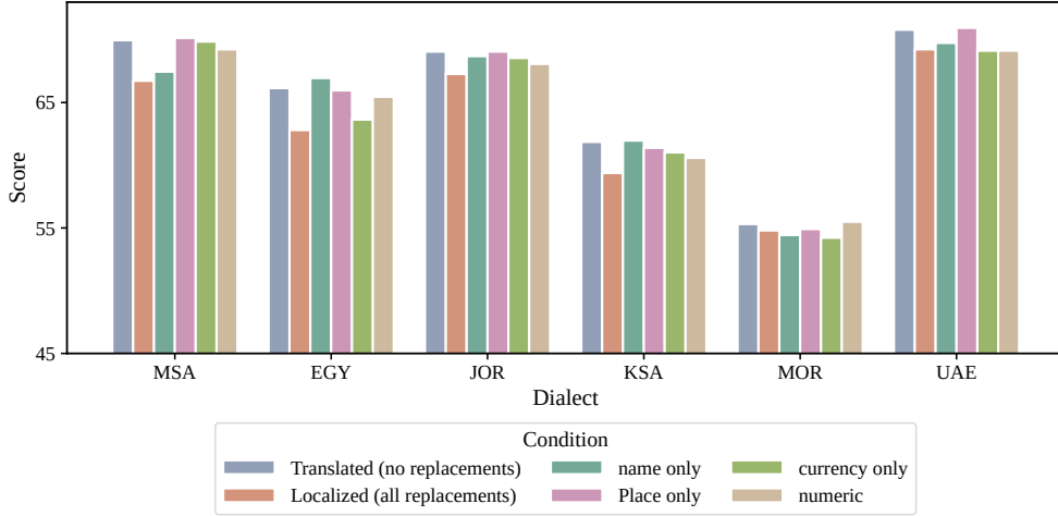
Figure 2: Performance by region and localization.
