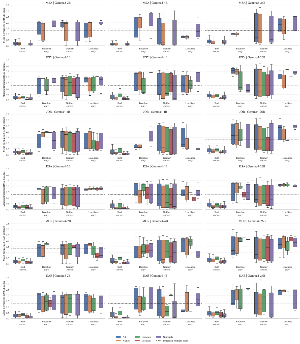
Figure 4: Residual-stream path distance by correctness group; dashed line = unrelated-problem average.
