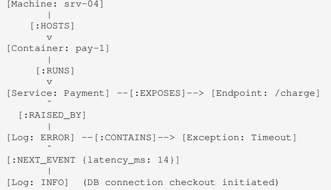
Fig. 1. Illustrative property-graph fragment linking physical infrastructure, logical services, and a temporal event chain.
