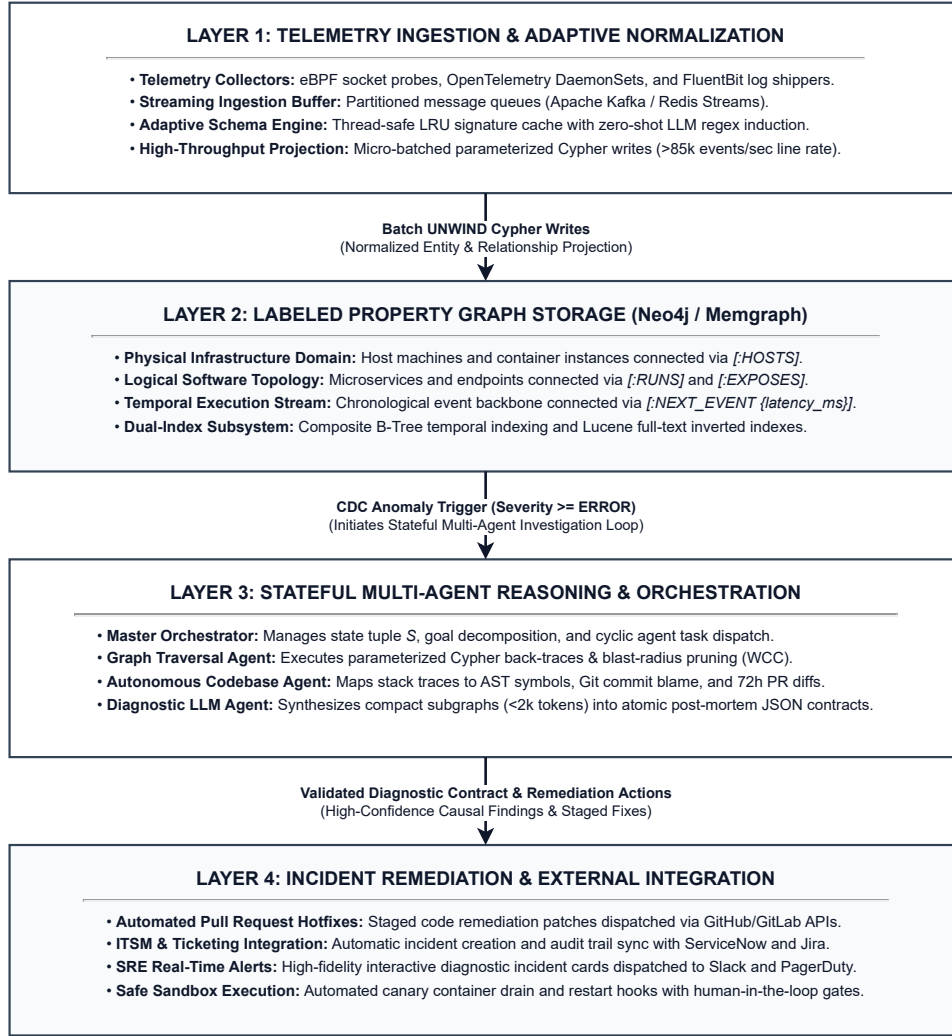
Fig. 2. Semantic Observability: end-to-end system architecture.
