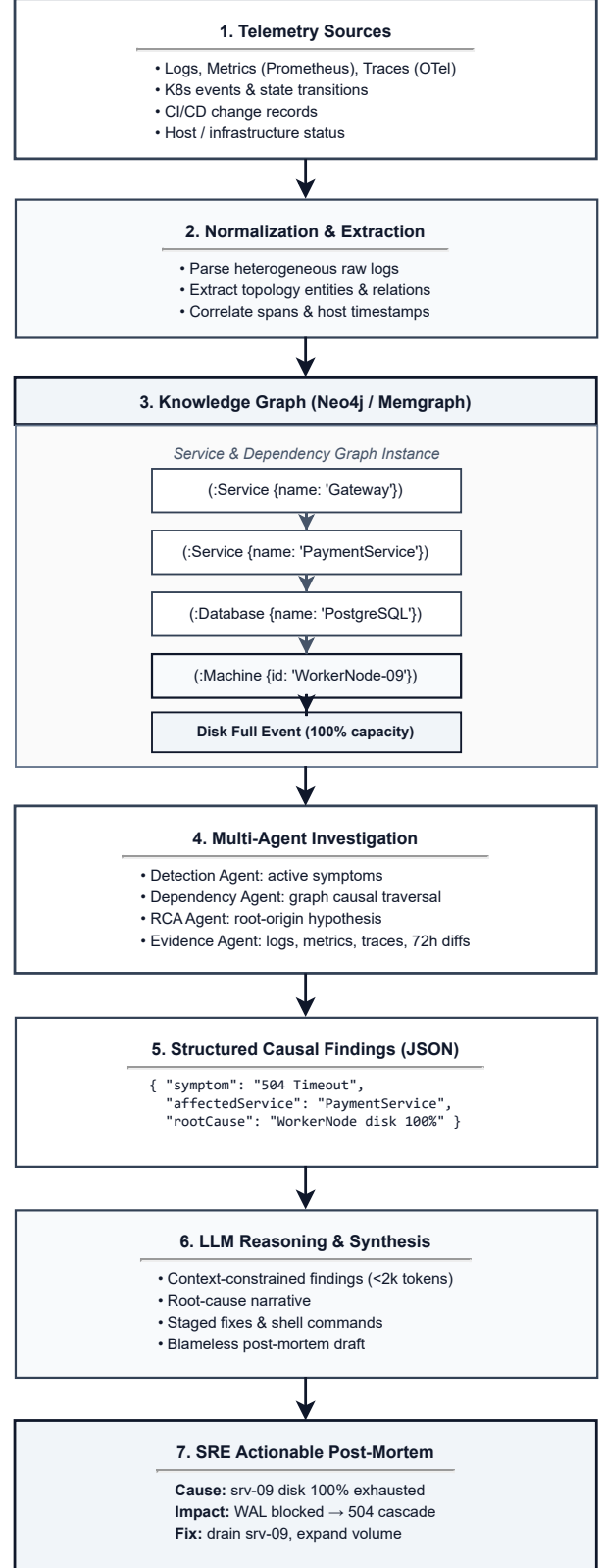
Fig. 4. Conceptual diagnostic pipeline architecture: end-to-end flow from telemetry ingestion to staged remediation.
