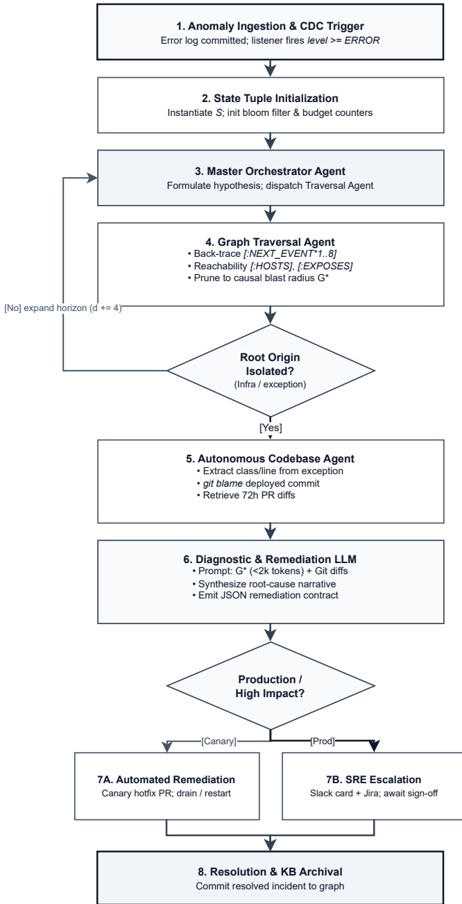
Fig. 3. Semantic Observability: multi-agent diagnostic workflow.
