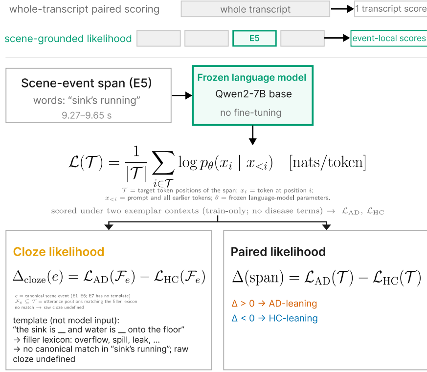
Figure 2: Two inputs, one scoring model: AD training examples followed by the target event text, and HC training examples followed by that same text. Only target tokens are scored. Their mean log-likelihood difference gives an event contrast; the cloze contrast restricts the average to lexicon-matched subwords of that text. The illustrated excerpt is abridged, and the hand-written cloze template is not a model input.
