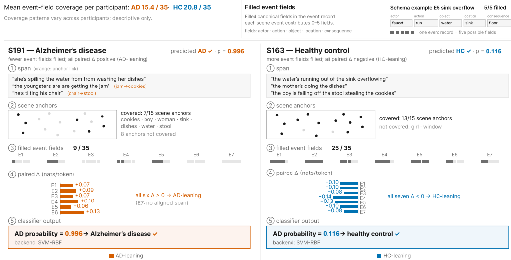
Figure 3: Inspecting scene-linked measurements through their source speech. Reports for two test participants connect retrieved utterances with scene-anchor matches, event-field coverage, and likelihood contrasts. E1–E7 denote cookie reaching, stool instability, girl observing, dishwashing, overflow, unawareness, and kitchen context. Filled fields indicate lexical matches; excerpts are abridged, while scores use the full retrieved text. Header means summarize event-field coverage across the 48 official-test participants. For each participant, the displayed probability is the model-estimated probability of Alzheimer’s disease, averaged across fifty runs. E7’s “no aligned span” indicates an unavailable event-text contrast.
