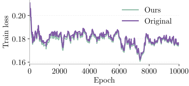
Figure 3. Training loss comparison between FlexAttentionGT (Ours) and GT (Original), smoothed with a window size of 20. Similar optimization dynamics suggest that gains stem from the attention layer’s inductive bias.
