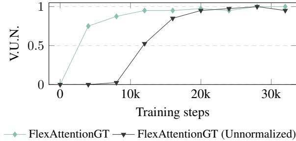
Figure 4. V.U.N. curves comparing normalized and unnormalized networks over training steps on the Planar dataset, evaluated with 1000 generation steps.
