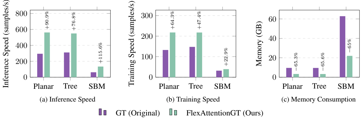
Figure 1. Computational efficiency across datasets. Percentages denote the relative change compared to the original implementation.
