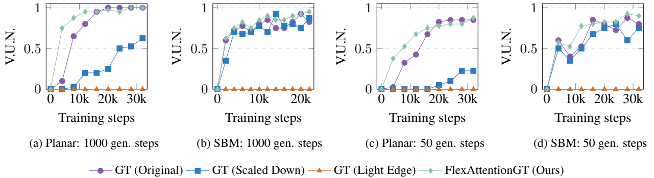
Figure 2. V.U.N. curves over training steps on the Planar and SBM datasets, comparing FlexAttentionGT against the original GT and its lightweight variants. We evaluate 1000 and 50 generation steps, respectively.
