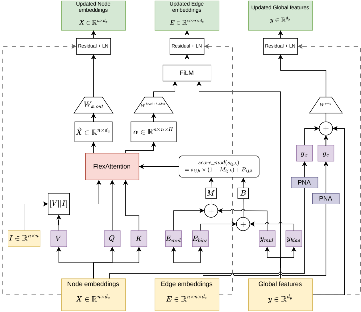
Figure 5. Schematic of the FlexAttentionGT architecture.
