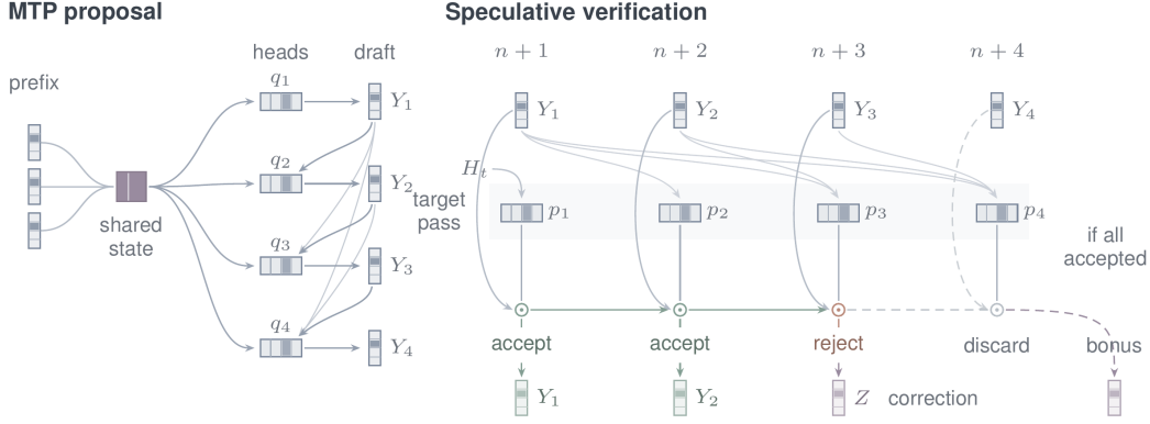
Figure 1: MTP with exact verification. Proposal heads condition on earlier sampled tokens. One target pass scores p_j(\cdot|H_t, Y_{<j}) , and circles denote prefix-ordered acceptance. Rejection emits a residual correction Z . The dashed bonus branch requires full acceptance.
