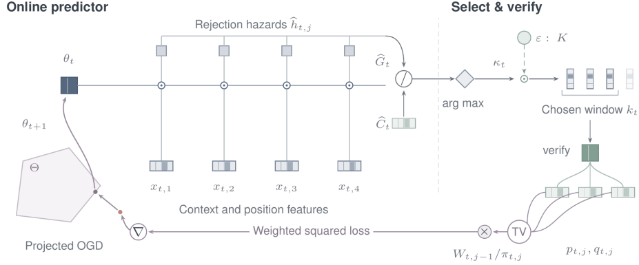
Figure 2: AMTP’s online control loop. Before drafting, it picks the horizon with the highest predicted throughput. Verification feedback at every drafted position, including those after a rejection, enters the weighted loss in Equation 8, and an OGD step updates the hazard predictor.
