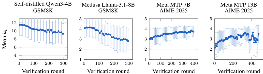
Figure 3: Draft window chosen by AMTP, averaged over generations in bins of 10 verification rounds (points; bars show one standard deviation across rounds in the bin). The window adapts as generation proceeds instead of staying at a single value.
