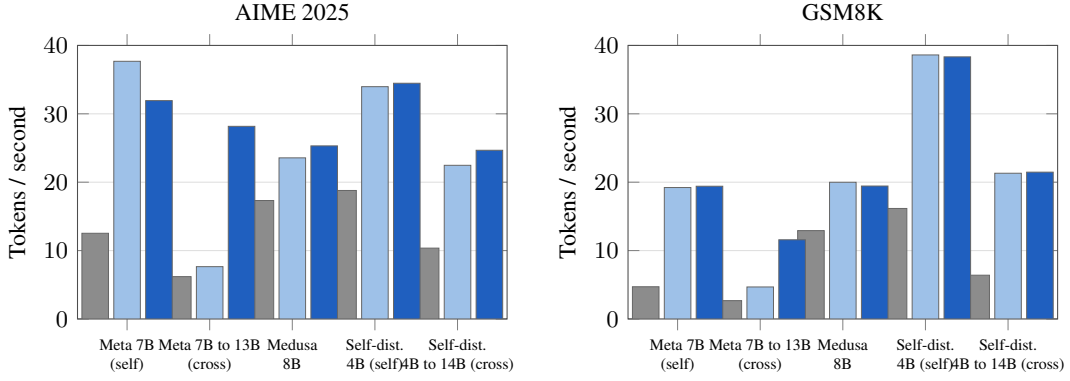
(a) Decoding throughput (tokens/second) for plain decoding, the best fixed window, and AMTP, across all five pairings and both evaluation tasks. Every multi-token-prediction condition beats plain decoding; the Meta MTP cross-model pairing (facebook/multi-token-prediction draft to Llama-2-13B target) shows the largest absolute gap between fixed and adaptive.
