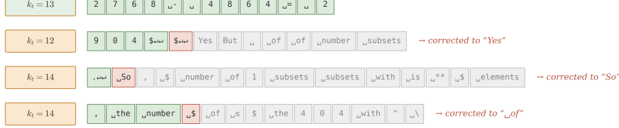
Figure 5: Four consecutive real verification rounds (648–651) from one adaptive-control-block run on AIME 2025 (self-distilled Qwen3-4B). Green tokens were accepted, the red token was rejected and replaced by the correction shown on the right (resampled from the residual), and grey tokens were drafted but never verified because the round already stopped at the rejection. The control block re-selects the window k_t every round (shown on the left). All tokens, windows, and corrections are taken directly from logged telemetry.
