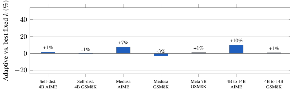
(b) Throughput of AMTP, relative to the best fixed window, self-speculative pairings and the modest-effect cross-model pairing (self-distilled 4B→14B).
