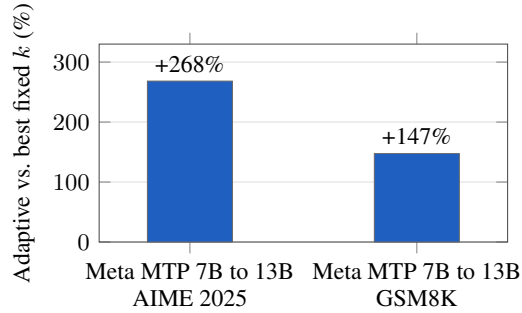
(c) The cross-model Meta MTP pairing (draft/target cost asymmetry), shown on its own axis given the scale of the effect relative to every other condition.
